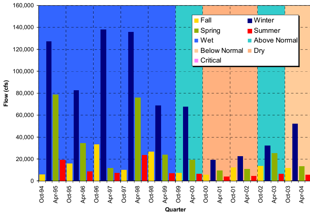
Figure 2B-14 Seasonal Net Delta Outflow Index, Water Years 1995 to 2004
