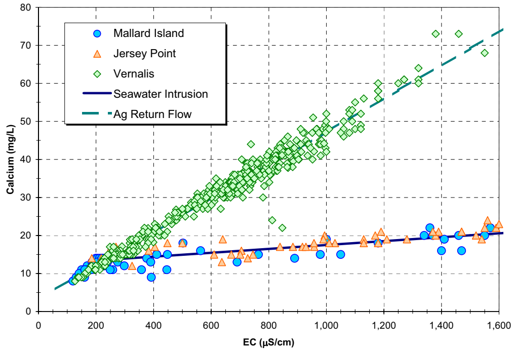
Figure 2C-11 Relationship Between Calcium Concentration and Electrical Conductivity
