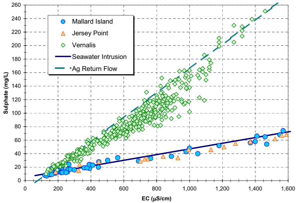
Figure 2C-12 Relationship Between Sulfate Concentration and Electrical Conductivity
