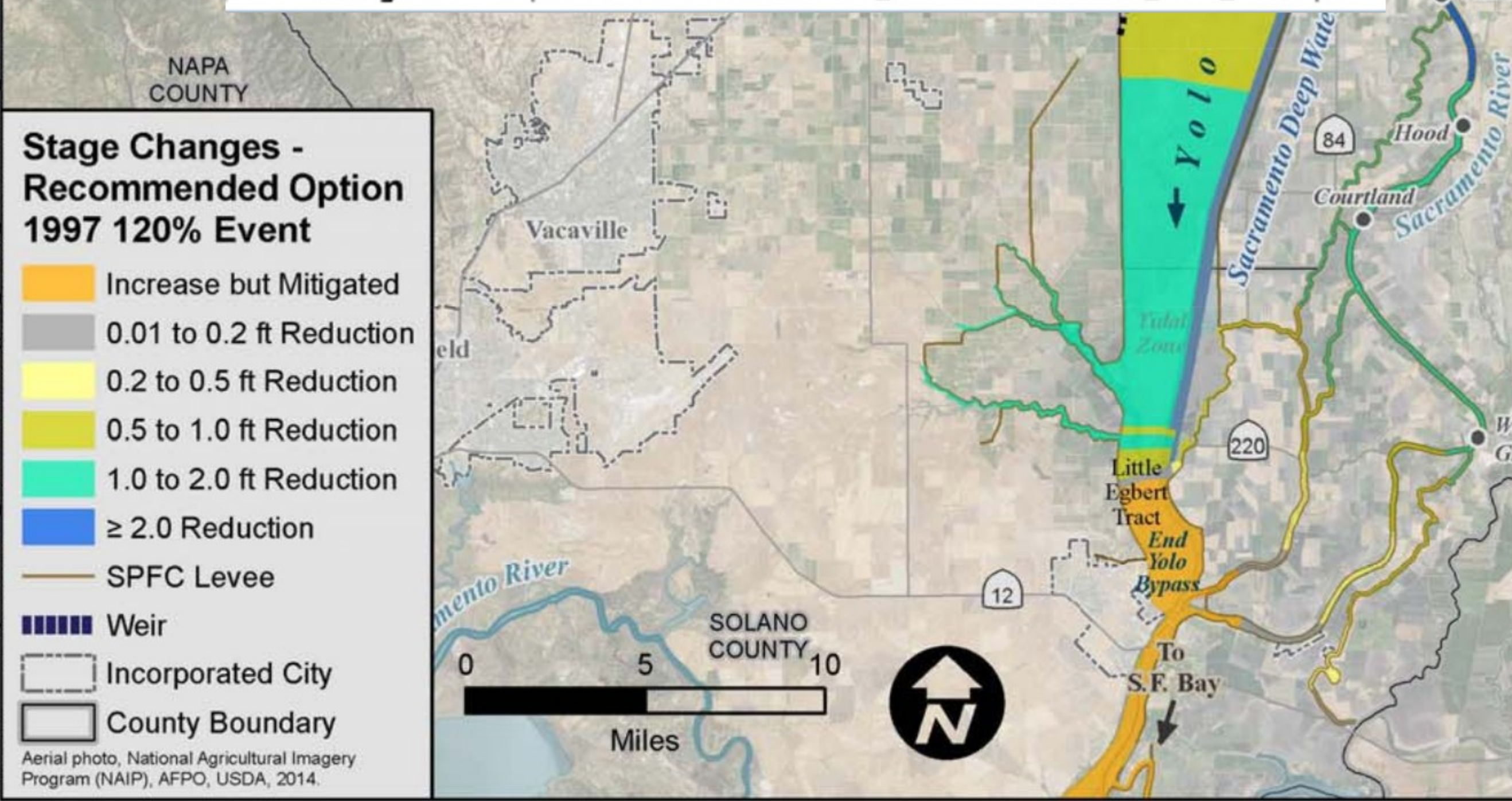
Figure 5-29. Hydraulic Performance in the Sacramento River Basin from Yolo Bypass Recommended Flood Event
