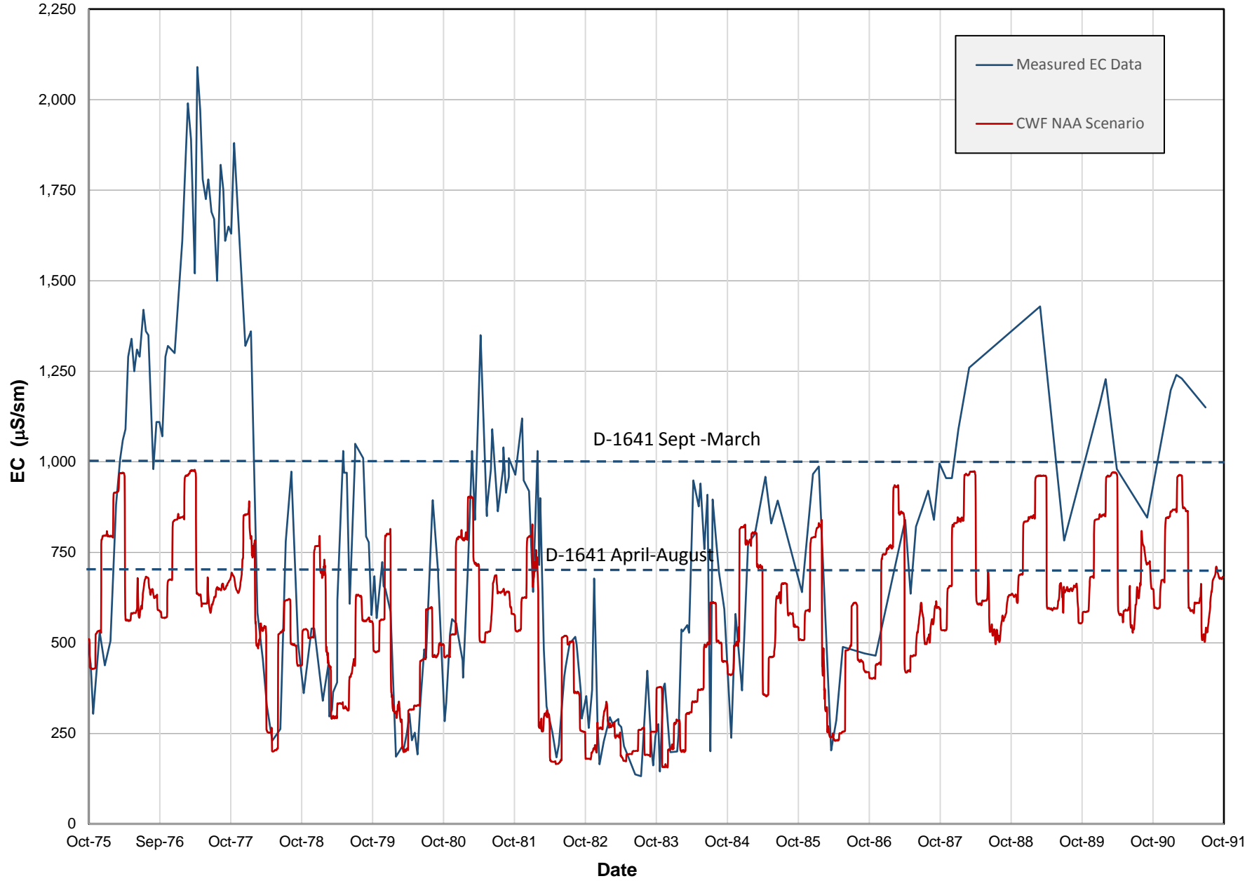
Figure 4-7 Measured Salinity At Old River at Tracy and The Predicted Salinity from The NAA
