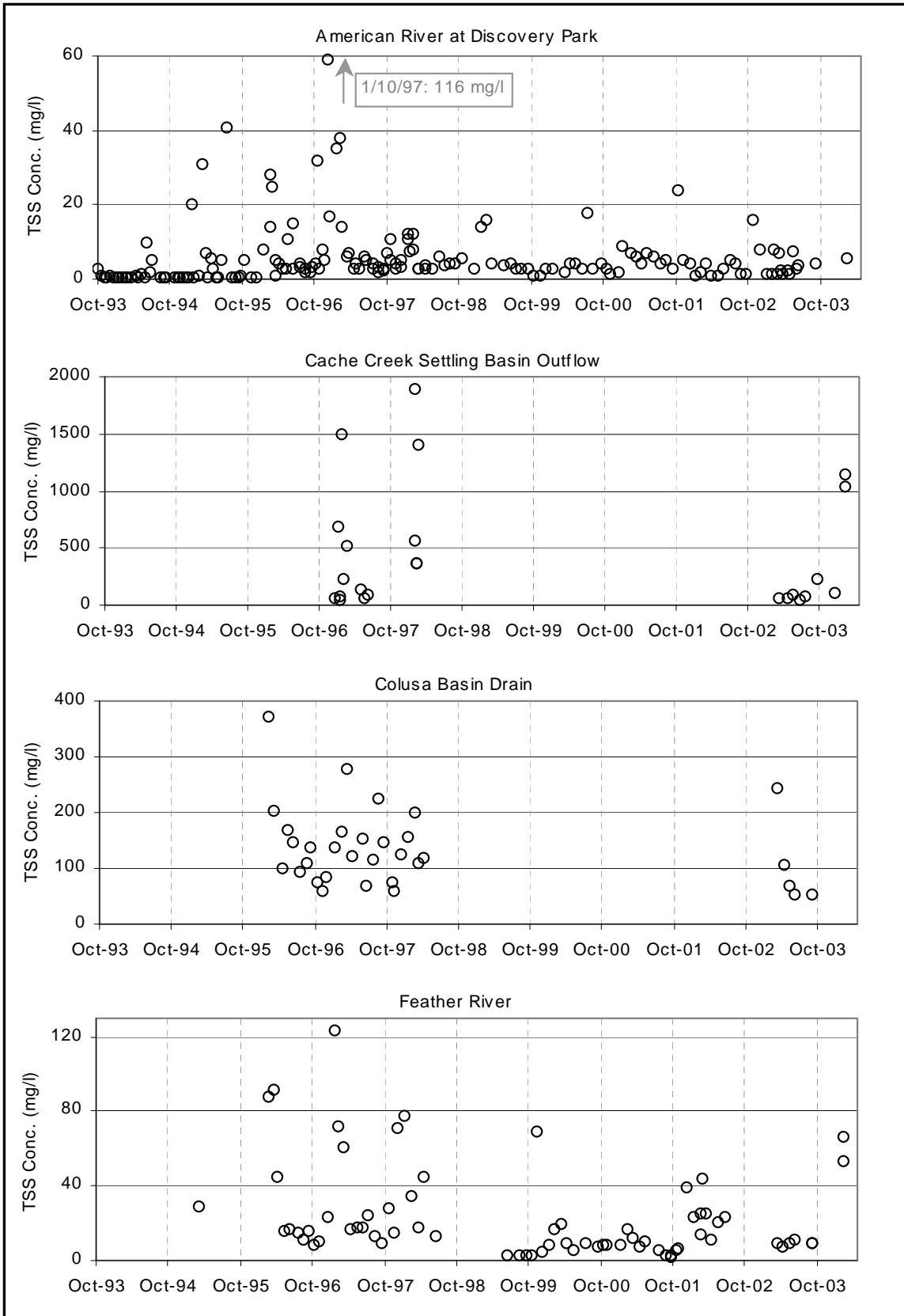
Figure I.5b: Available TSS Concentration Data for American River, Cache Creek, Colusa Basin & Feather River Watershed Outflow Locations.
