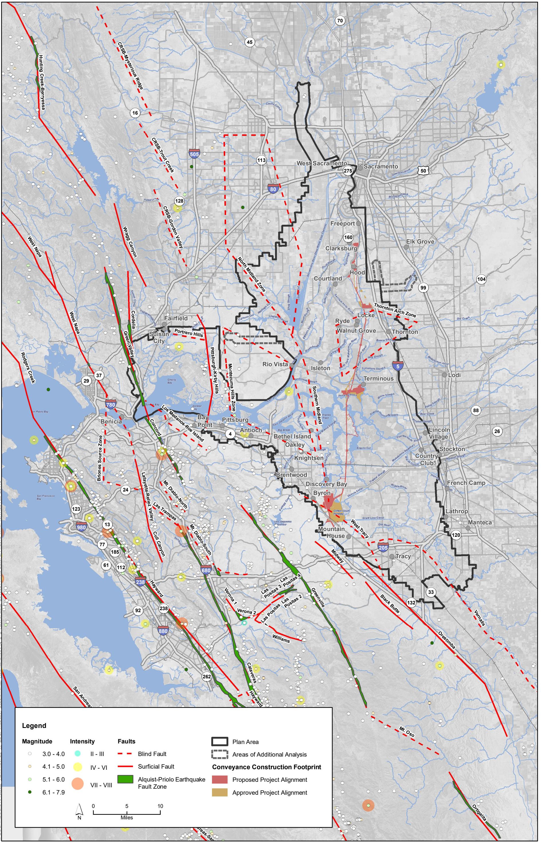
Figure 9-3 Active Faults and Historical Seismicity of the Bay and Delta Region, 1800–2010
