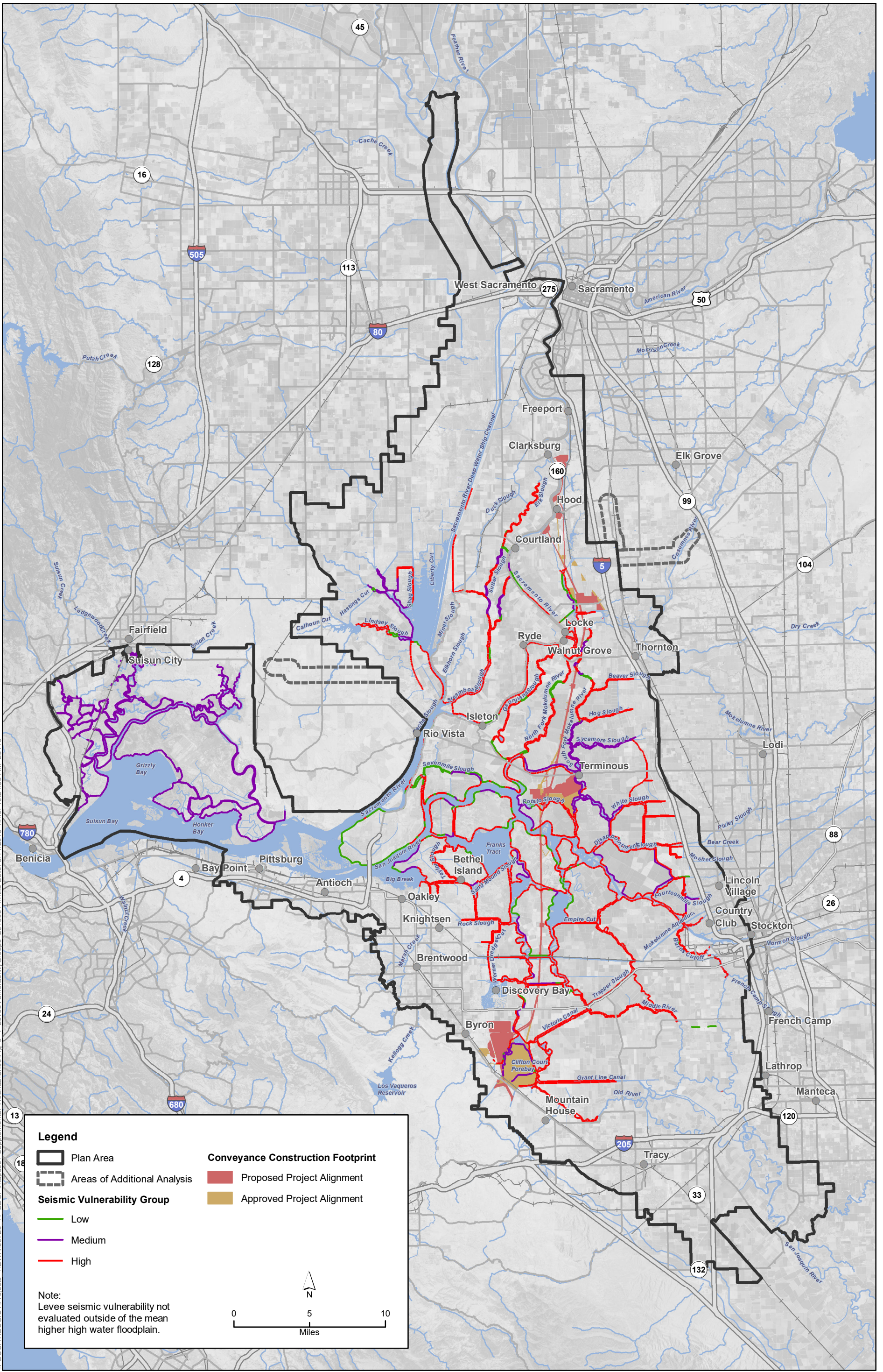
Figure 9-4 Levee Seismic Vulnerability Groups
