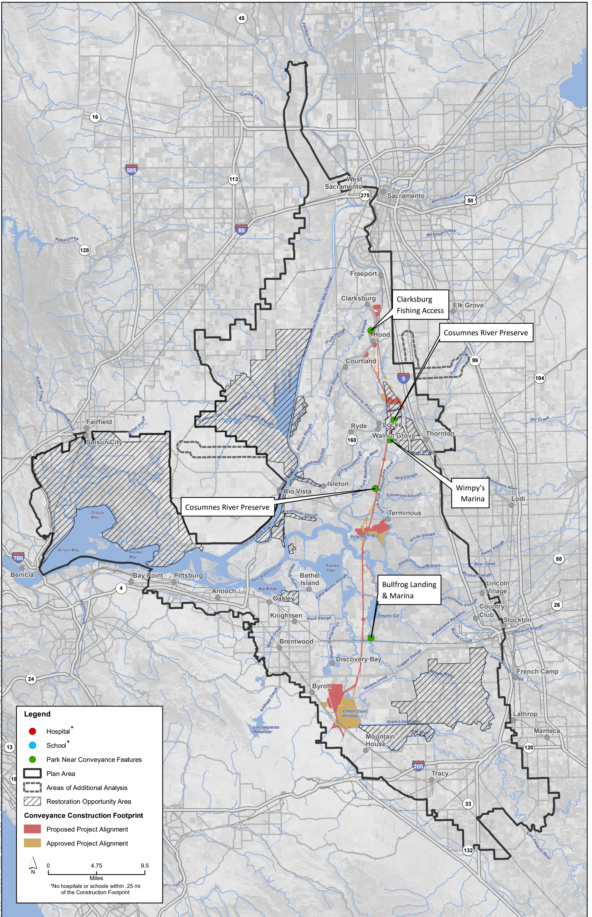
Figure 24-5 Sensitive Receptors
