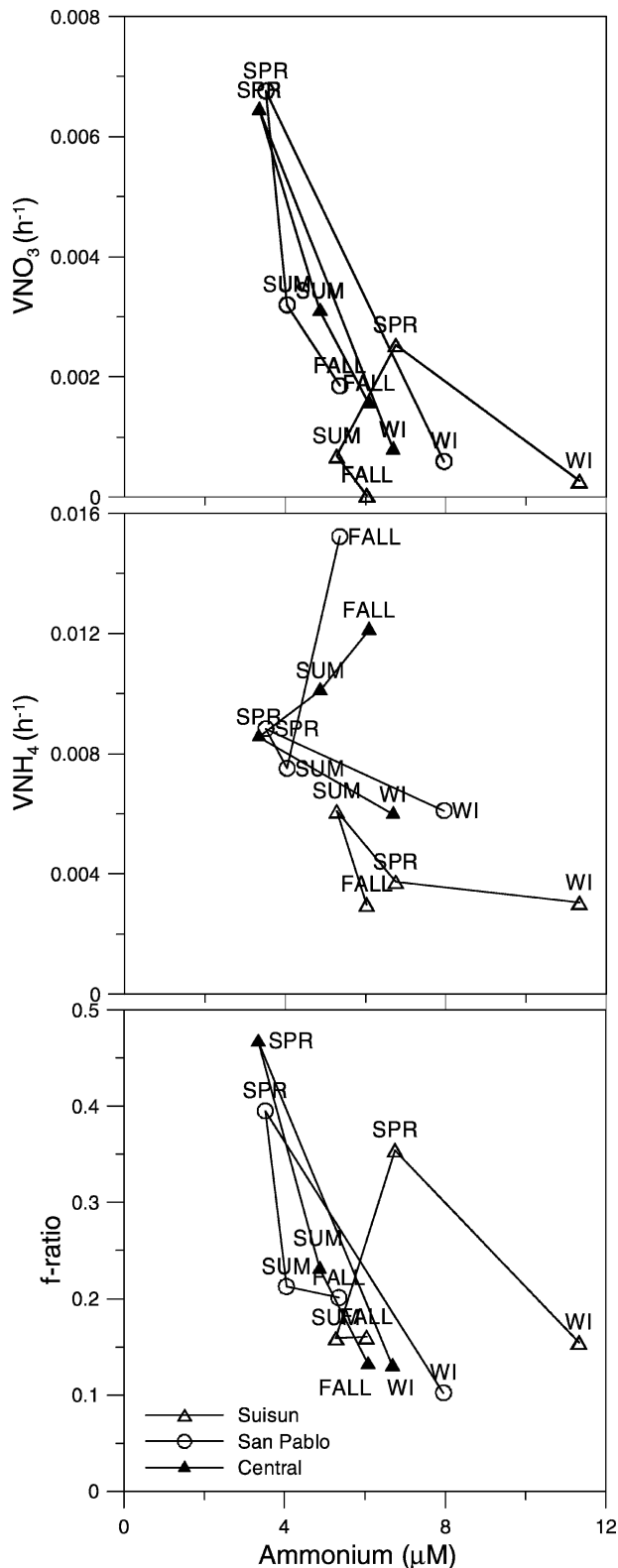
Fig. 6. Mean \text{NO}_3 uptake ( \text{VNO}_3 ), mean \text{NH}_4 uptake ( \text{VNH}_4 ), and f ratio calculated as \rho\text{NO}_3/(\rho\text{NO}_3 + \rho\text{NH}_4) for Suisun, San Pablo, and Central Bays versus mean \text{NH}_4 concentration for all three years for winter (WI), spring (SPR), summer (SUM), and fall (FALL) months.
