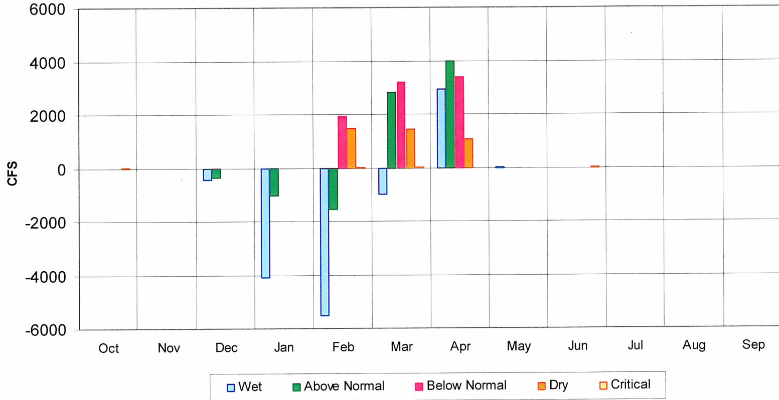
EXHIBIT SVWU-44 SACRAMENTO RIVER FLOW TO YOLO BYPASS DIFFERENCE BETWEEN UCD2 (SACRAMENTO RIVER TARGETS) AND BIOLOGICAL OPINION'S AVERAGE MONTHLY DIFFERENCE BY WATER-YEAR TYPE FOR 1922-2003
