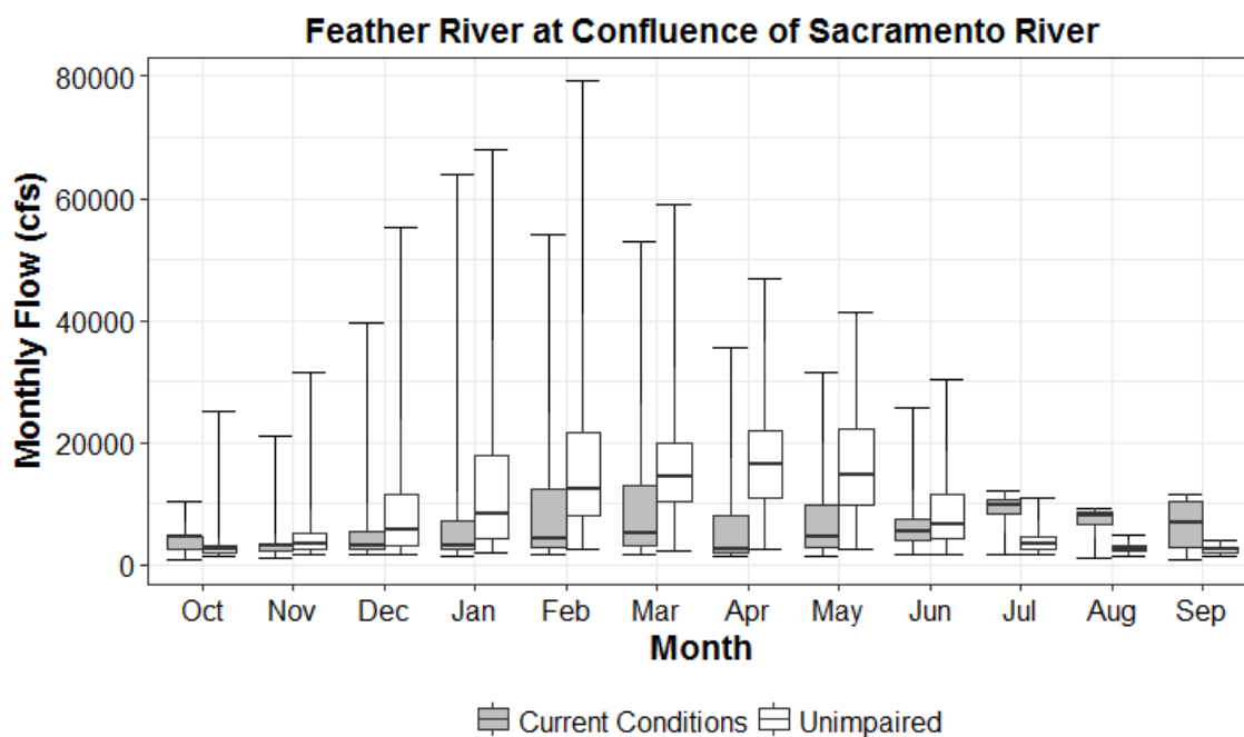
Figure 2.2-14. Feather River at Confluence with the Sacramento River Simulated Current Conditions (gray) and Unimpaired (white) Monthly Flows
