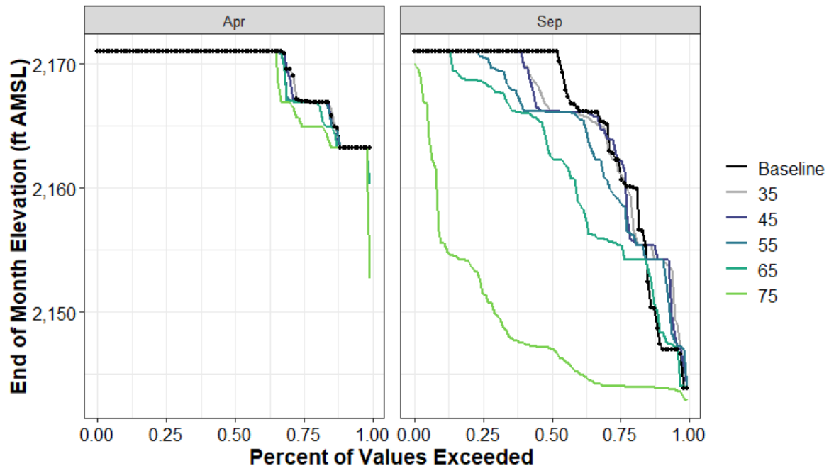
Figure A1-145. Rollins Reservoir End-of-April and End-of-September Elevation Percent Exceedance Plot
