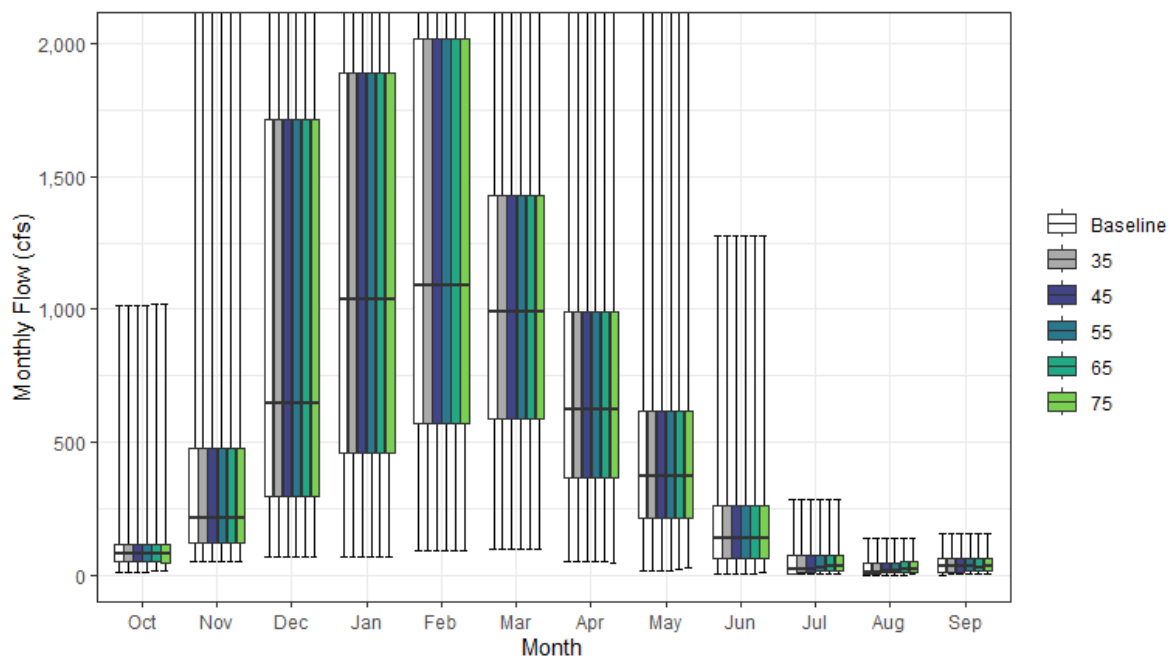
Figure A1-19. Cow Creek Streamflow above Confluence with Sacramento River Monthly Boxplot
