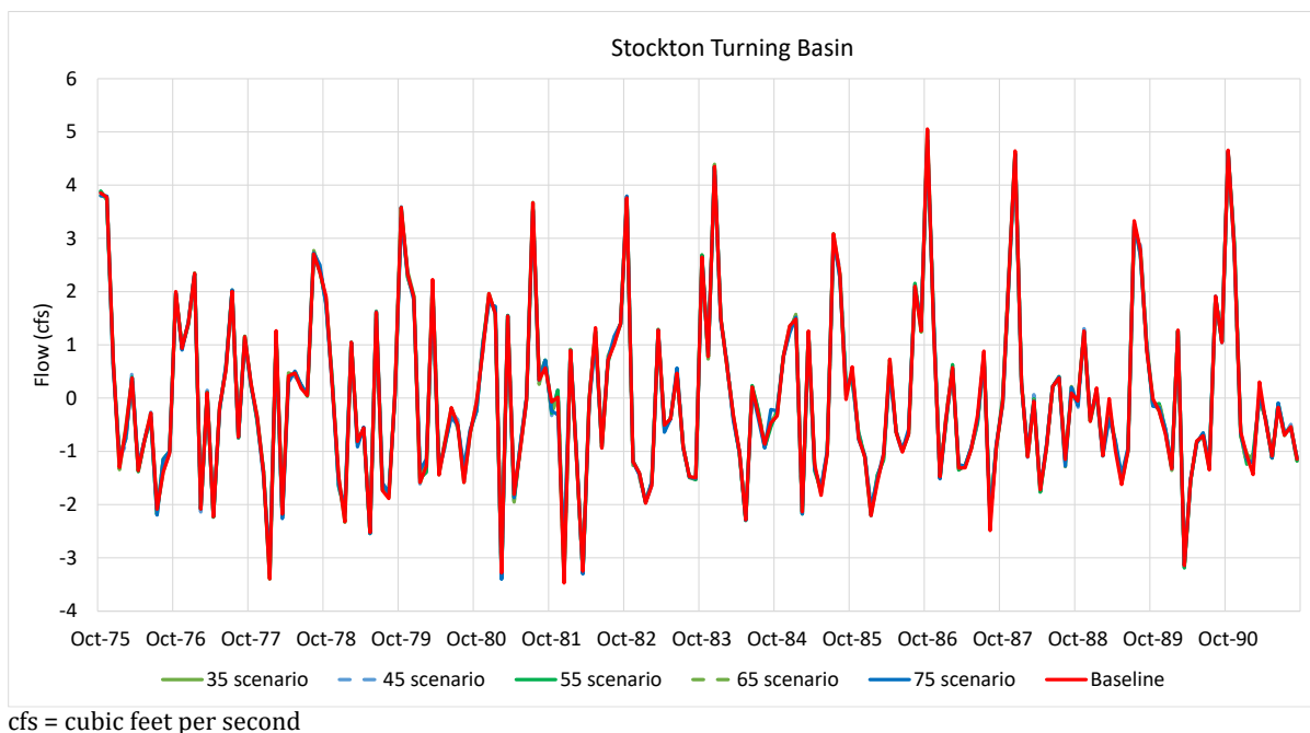
Figure A2-15. DSM2 Flow in the San Joaquin River near Stockton – Baseline and Flow Scenarios for WY 1976–1991
