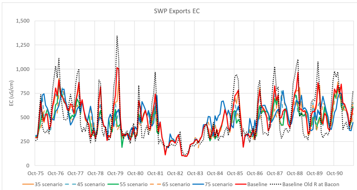
Figure A2-27. Time Series of DSM2 EC Values for SWP Exports – Baseline and Flow Scenarios for WY 1976–1991 with Baseline Old River at Bacon Island EC for Reference
