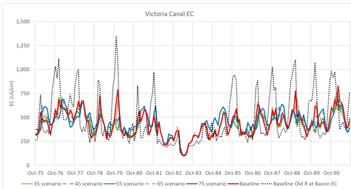
Figure A2-26. Time Series of DSM2 EC Values for Victoria Canal EC (CCWD Middle River Intake) for Baseline and Flow Scenarios for WY 1976–1991
