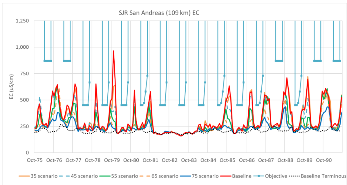
Figure A2-22. Time Series of DSM2 EC Values for San Andreas Landing – Baseline and Flow Scenarios for WY 1976–1991 with EC Objectives for Reference
