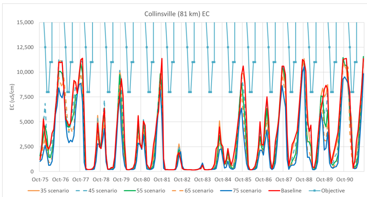
Figure A2-19. Time Series of DSM2 EC Values for Collinsville – Baseline and Flow Scenarios for WY 1976–1991 with EC Objectives for Reference
