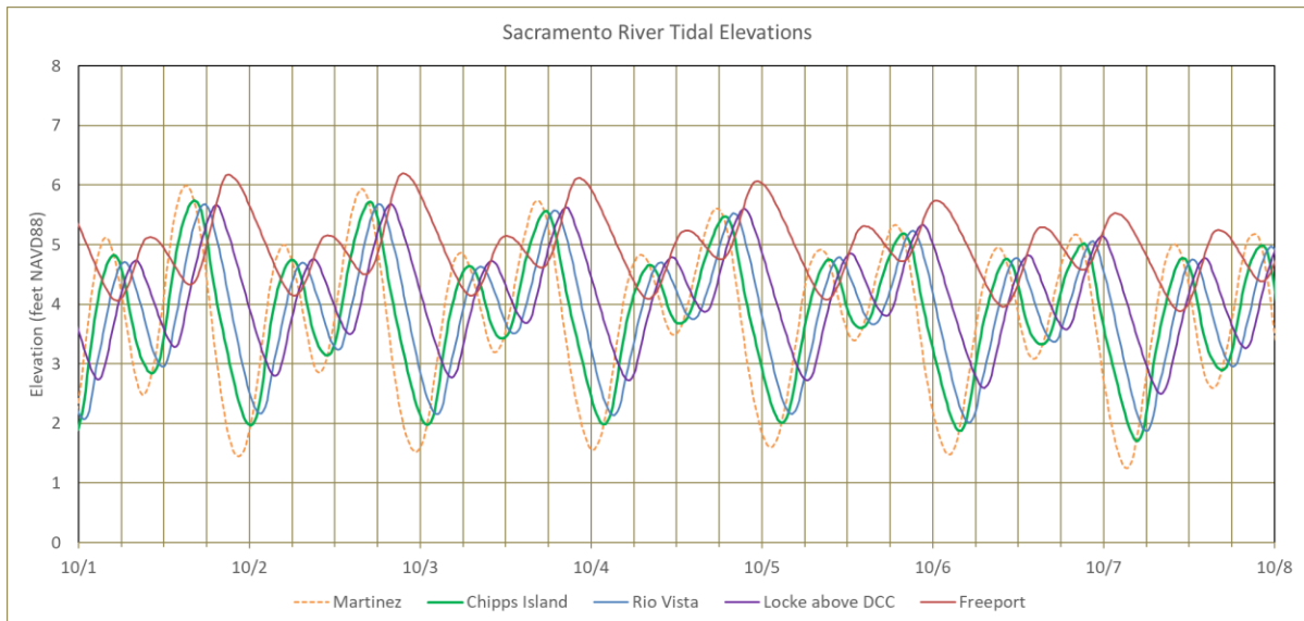
Figure A2-3. DSM2 Tidal Elevations at Martinez and at Upstream Sacramento River Locations for October 1–7, 1977
