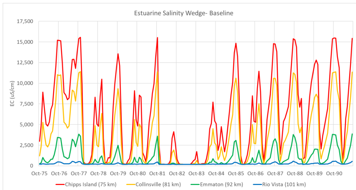
Figure A2-16. Time Series of DSM2 EC Values at Chipps Island (75 km), Collinsville (81 km), Emmaton (92 km), and Rio Vista (101 km) – Baseline for WY 1976–1991
