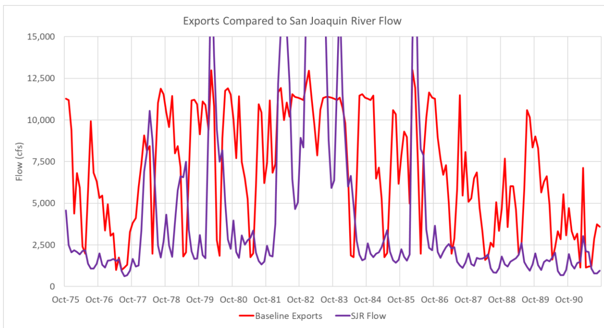
Figure A2-8. Comparison of San Joaquin River Inflows with Baseline Combined CVP and SWP Exports for WY 1976–1991
