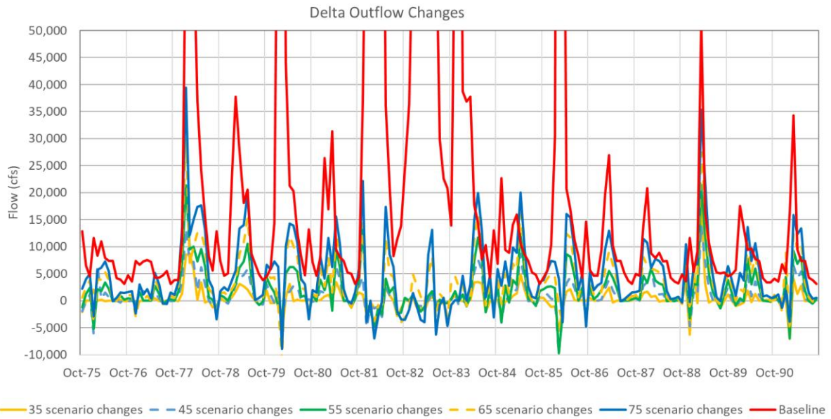
Figure A2-10. Delta Outflow – Baseline and Changes from Baseline for the Flow Scenarios for WY 1976–1991
