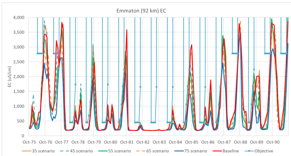
Figure A2-21. Time Series of DSM2 EC Values for Emmaton – Baseline and Flow Scenarios for WY 1976–1991 with EC Objectives for Reference
