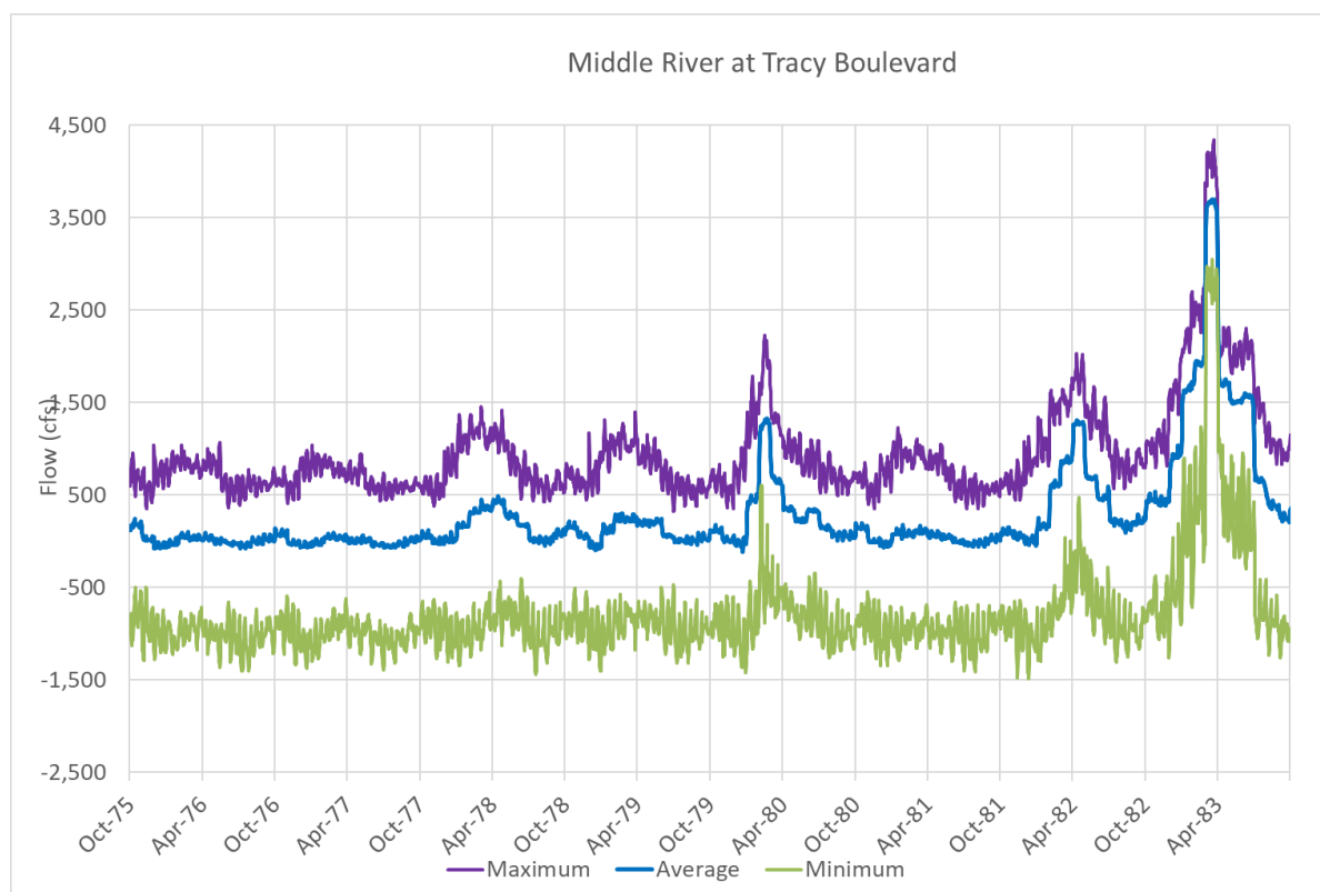
Figure A2-6. DSM2 Daily Tidal Flows in Middle River at Tracy Boulevard Upstream of the Temporary Barrier for WY 1976–1983
