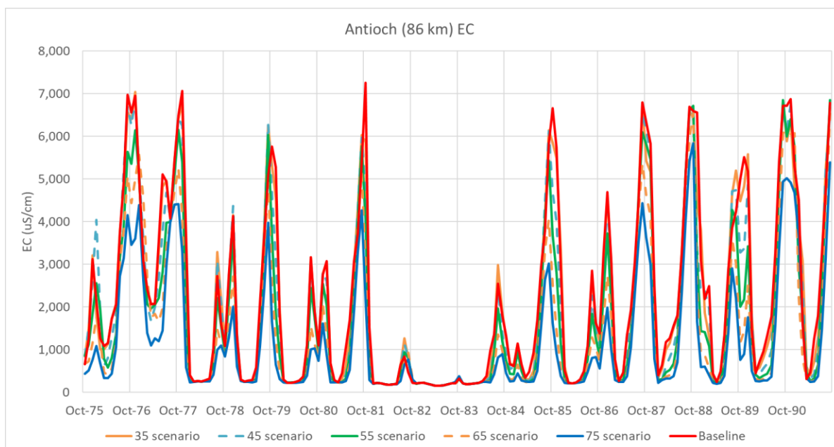
Figure A2-23. Time Series of DSM2 EC Values for Antioch EC – Baseline and Flow Scenarios for WY 1976–1991
