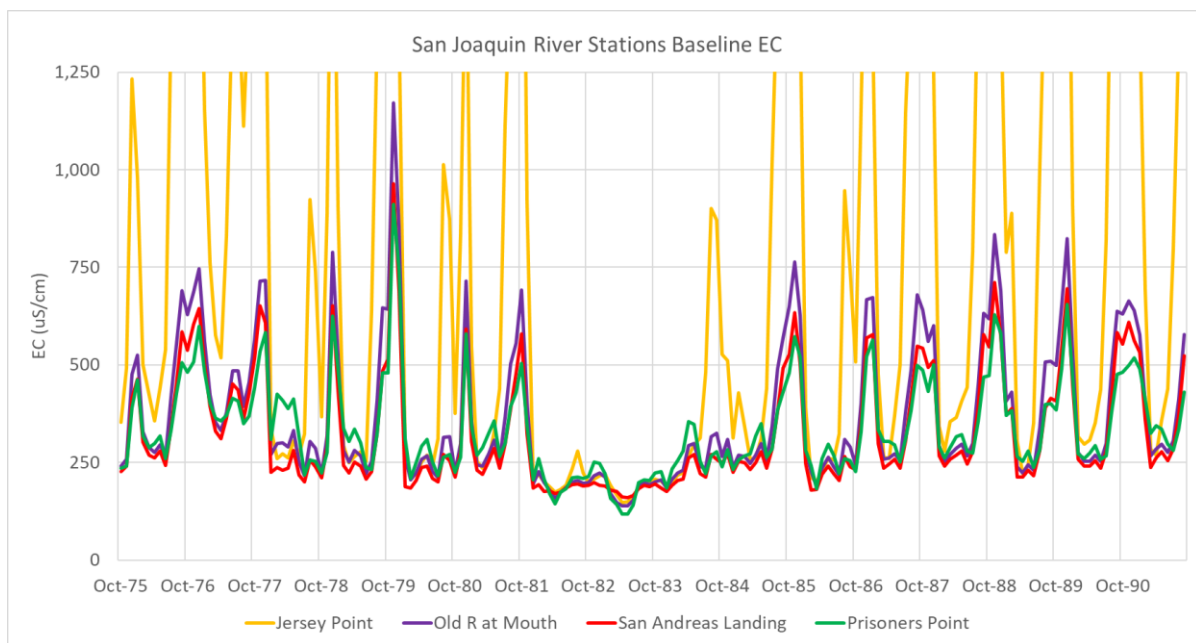
Figure A2-30. Time Series of DSM2 Baseline EC Values for San Joaquin River Stations for WY 1976–1991
