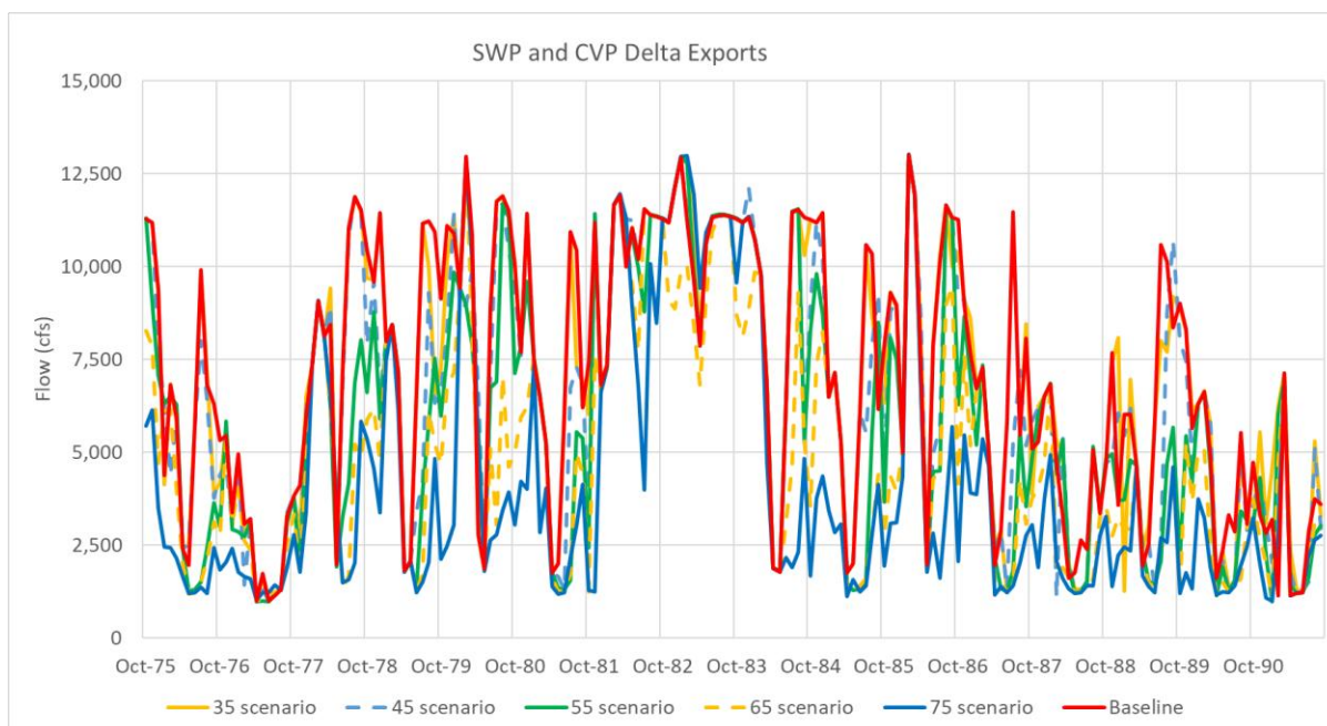
Figure A2-11. SacWAM CVP and SWP Delta Exports – Baseline and Flow Scenarios for WY 1976–1991
