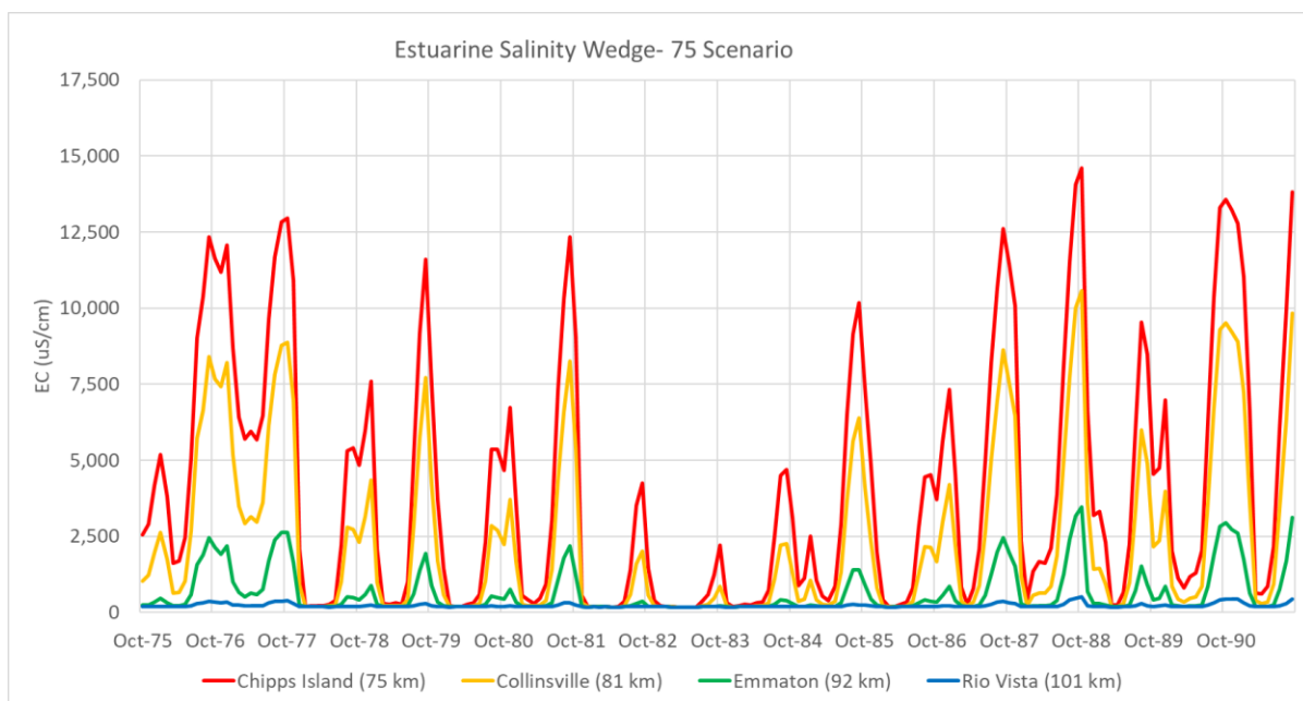
Figure A2-17. Time Series of DSM2 EC Values at Chippis Island (75 km), Collinsville (81 km), Emmaton (92 km), and Rio Vista (101 km) – 75 Scenario for WY 1976–1991
