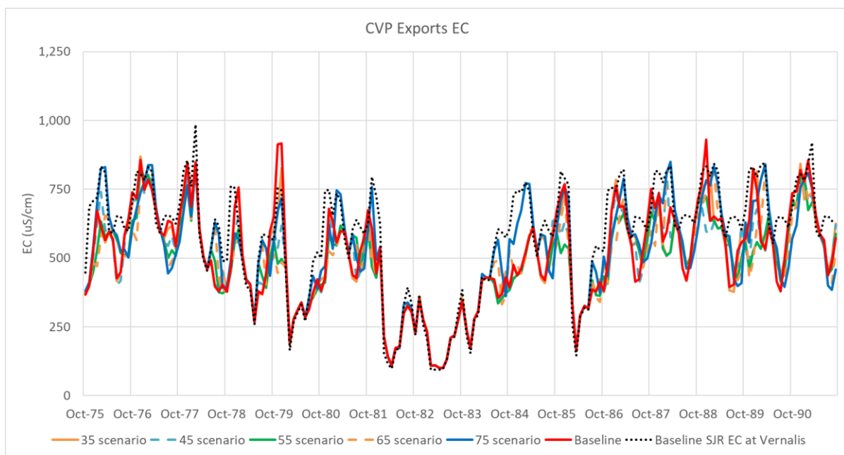
Figure A2-28. Time Series of DSM2 EC Values for CVP Exports – Baseline and Flow Scenarios for WY1976–1991 with Baseline San Joaquin River EC for Reference
