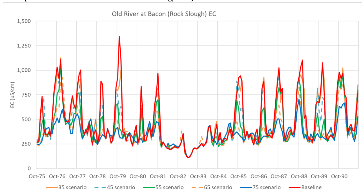
Figure A2-24. Time Series of DSM2 EC Values for Old River at Bacon Island (CCWD Rock Slough Intake) – Baseline and Flow Scenarios for WY 1976–1991
