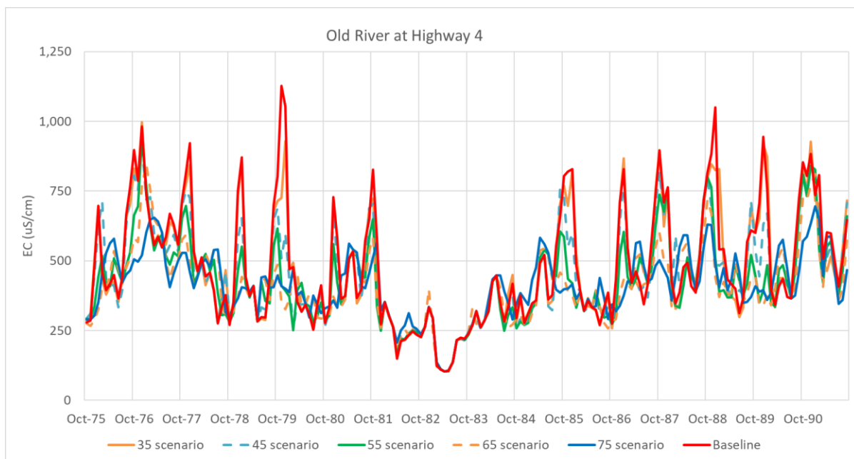
Figure A2-25. Time Series of DSM2 EC Values for Old River at Highway 4 (CCWD Old River Intake) – Baseline Compared with Flow Scenarios for WY 1976–1991
