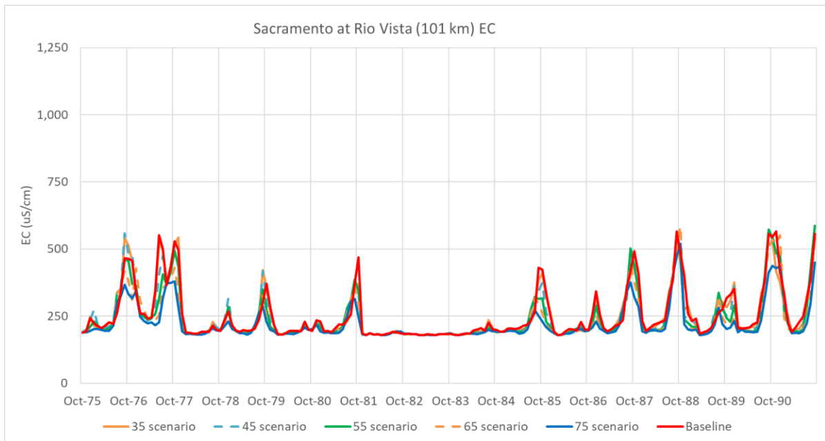
Figure A2-29. Time Series of DSM2 EC Values for the Sacramento River at Rio Vista – Baseline and Flow Scenarios for WY 1976–1991
