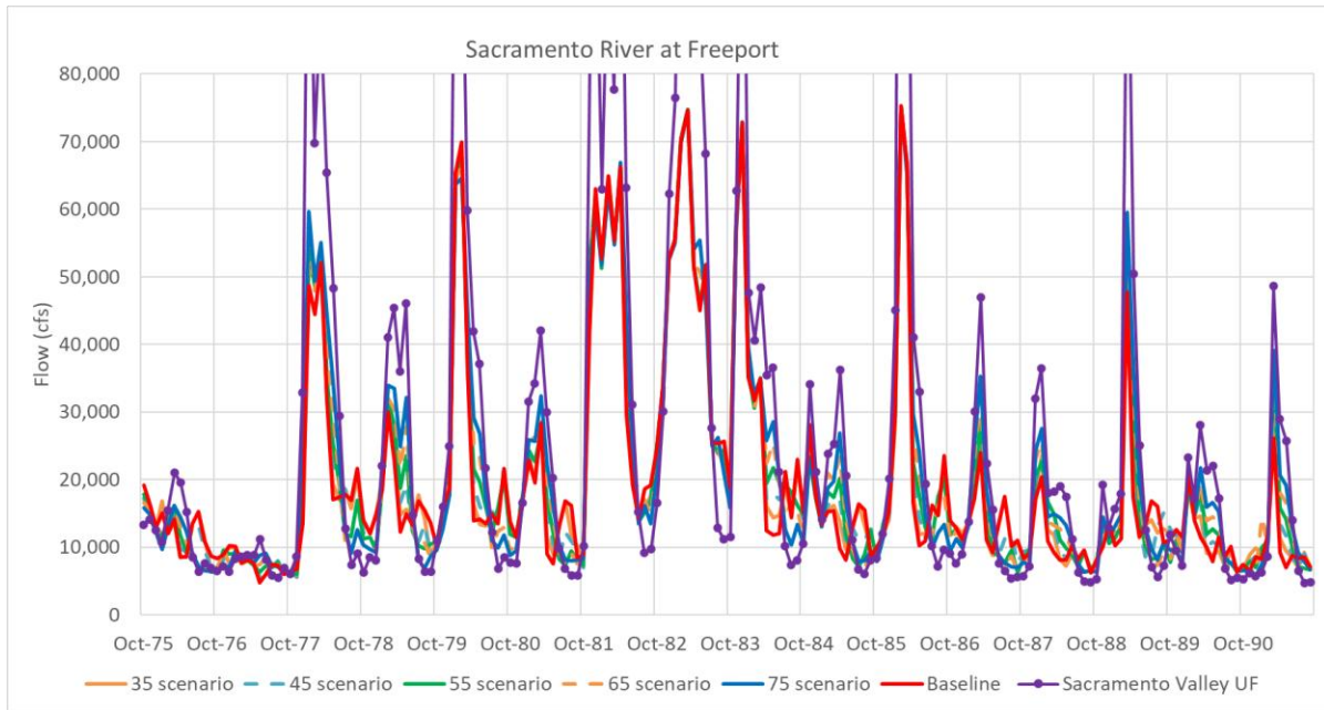
Figure A2-9. SacWAM Sacramento River Flow at Freeport – Baseline and Flow Scenarios for WY 1976–1991
