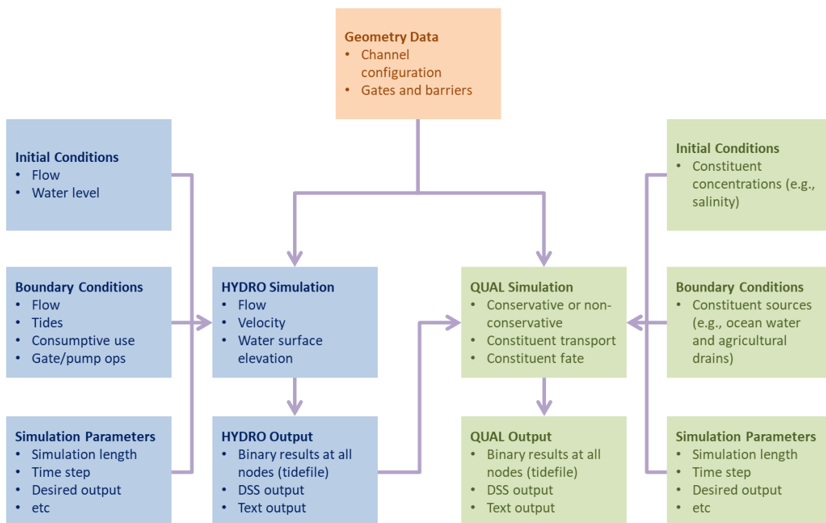
Figure A2a-3. Flow Chart of HYDRO and QUAL Inputs and Outputs
