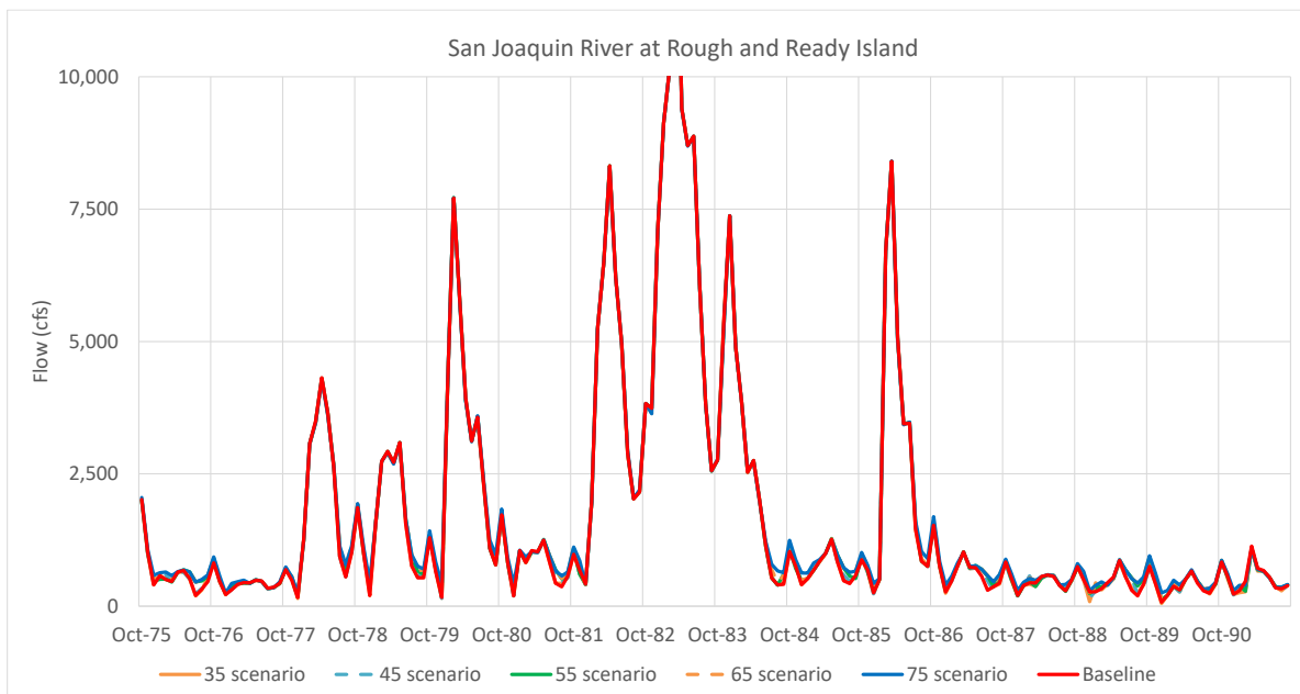
Figure A2-14. DSM2 Flow in the San Joaquin River near Stockton – Baseline and Flow Scenarios for WY 1976–1991
