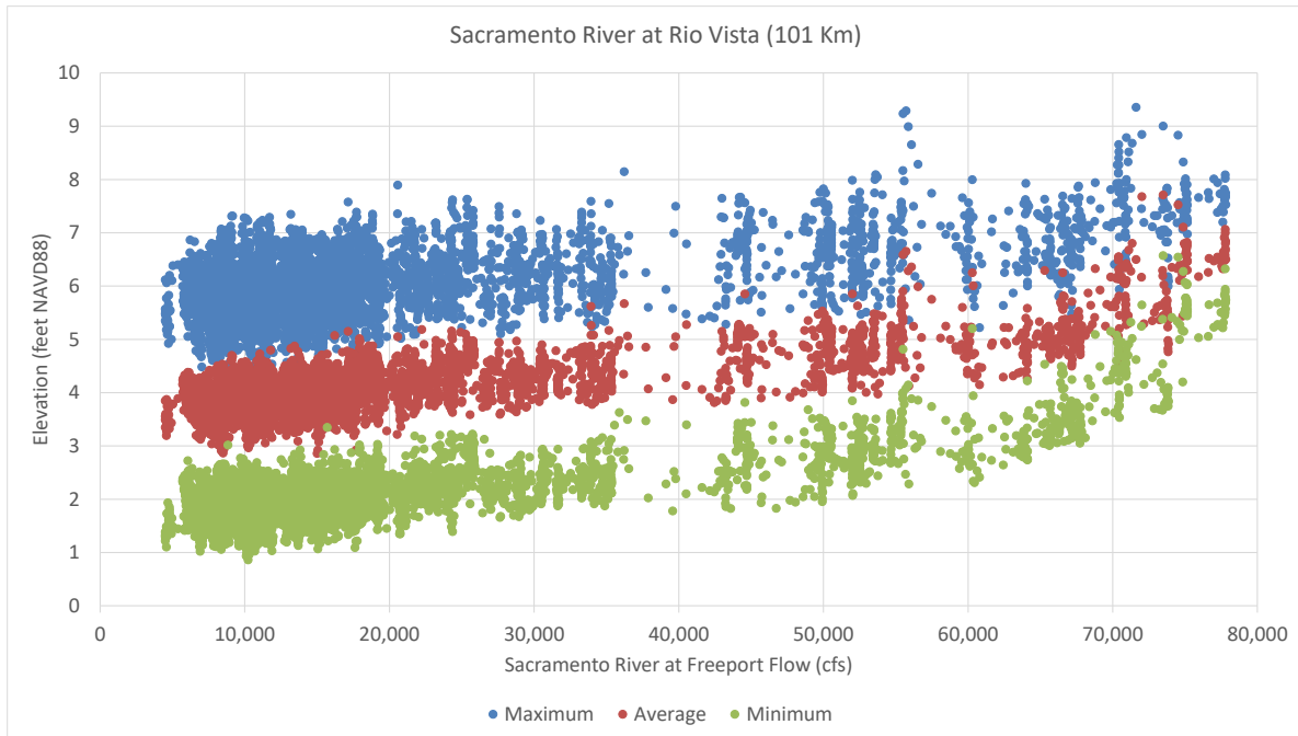
Figure A2-4. DSM2 Daily Tidal Elevations (Minimum, Average, Maximum) at Rio Vista as Influenced by Sacramento River Flow
