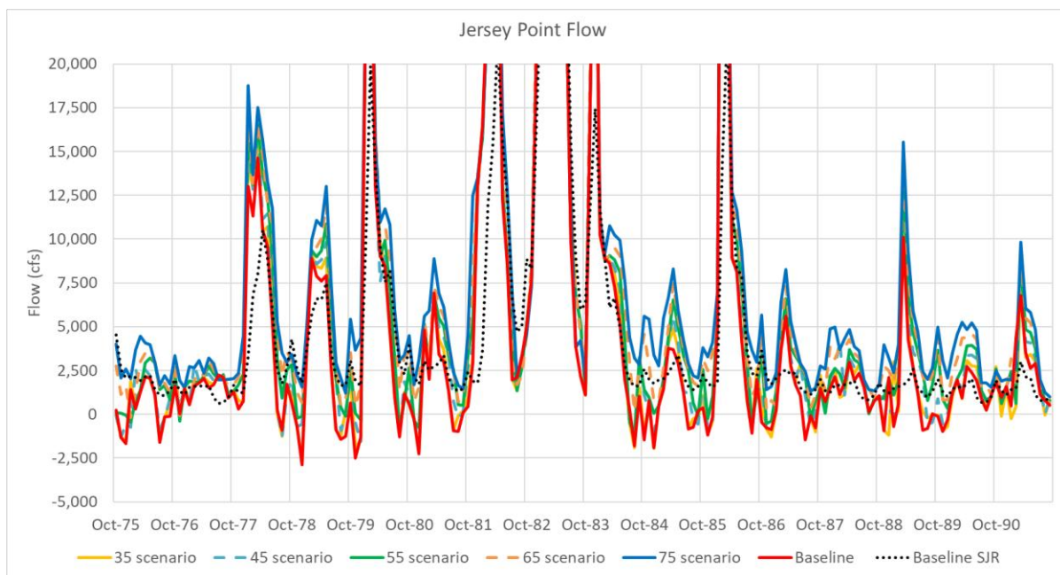
Figure A2-12. San Joaquin River Flow at Jersey Point – Baseline and Flow Scenarios for WY 1976–1991
