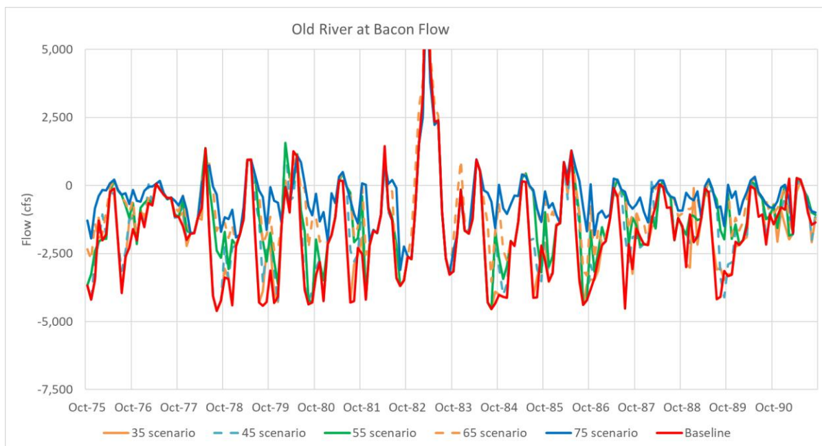
Figure A2-13. DSM2 Flow in Old River at Bacon Island – Baseline and Flow Scenarios for WY 1976–1991
