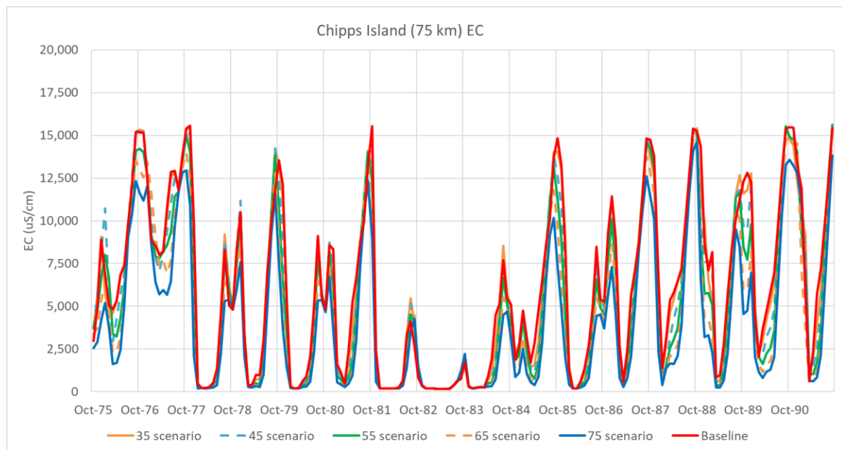
Figure A2-18. Time Series of DSM2 EC Values for Chipps Island – Baseline and Flow Scenarios for WY 1976–1991
