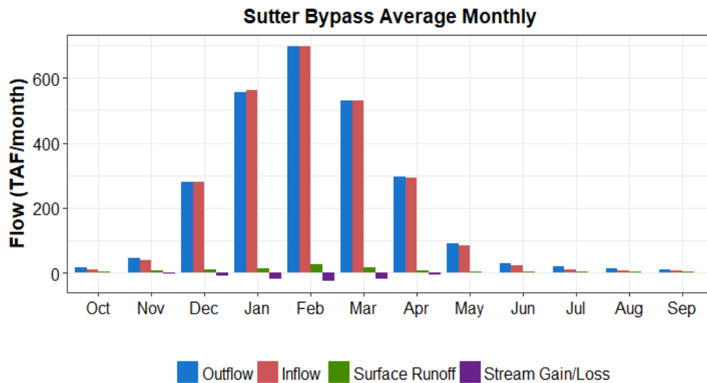
Figure A7-23. Monthly Average Unimpaired Flow Components for Sutter Bypass
