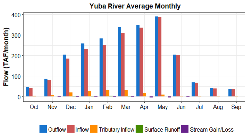
Figure A7-27. Monthly Average Unimpaired Flow Components for Yuba River
