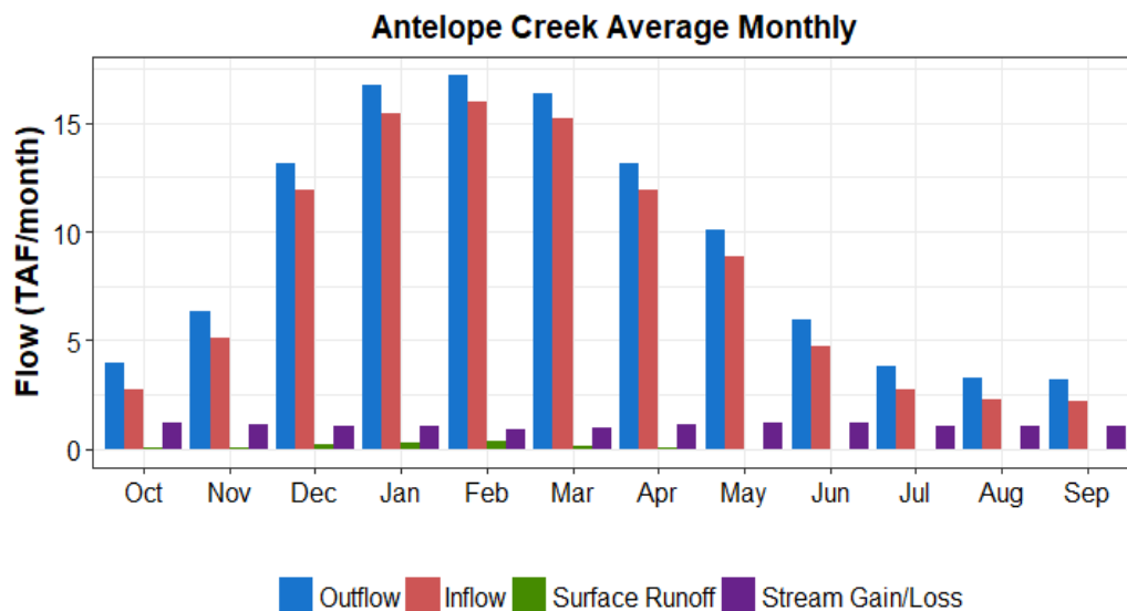
Figure A7-3. Monthly Average Unimpaired Flow Components for Antelope Creek
