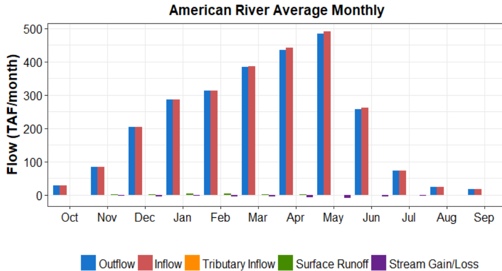
Figure A7-2. Monthly Average Unimpaired Flow Components for the American River
