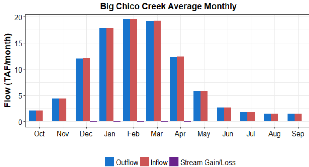
Figure A7-6. Monthly Average Unimpaired Flow Components for Big Chico Creek
