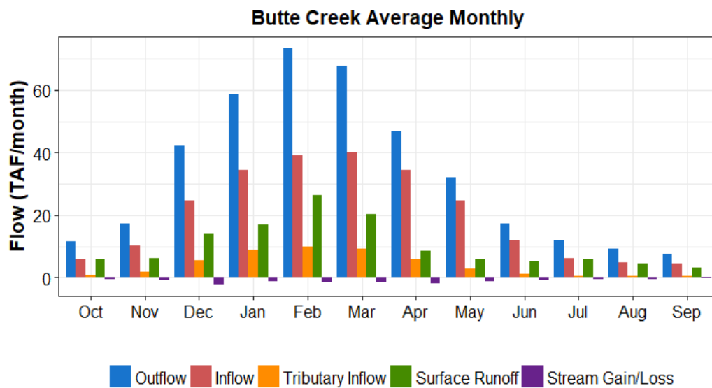
Figure A7-7. Monthly Average Unimpaired Flow Components for Butte Creek
