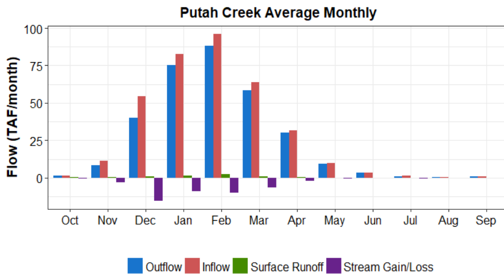
Figure A7-21. Monthly Average Unimpaired Flow Components for Putah Creek
