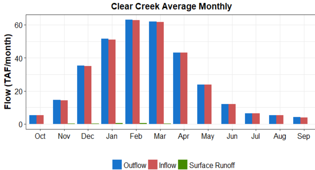
Figure A7-10. Monthly Average Unimpaired Flow Components for Clear Creek
