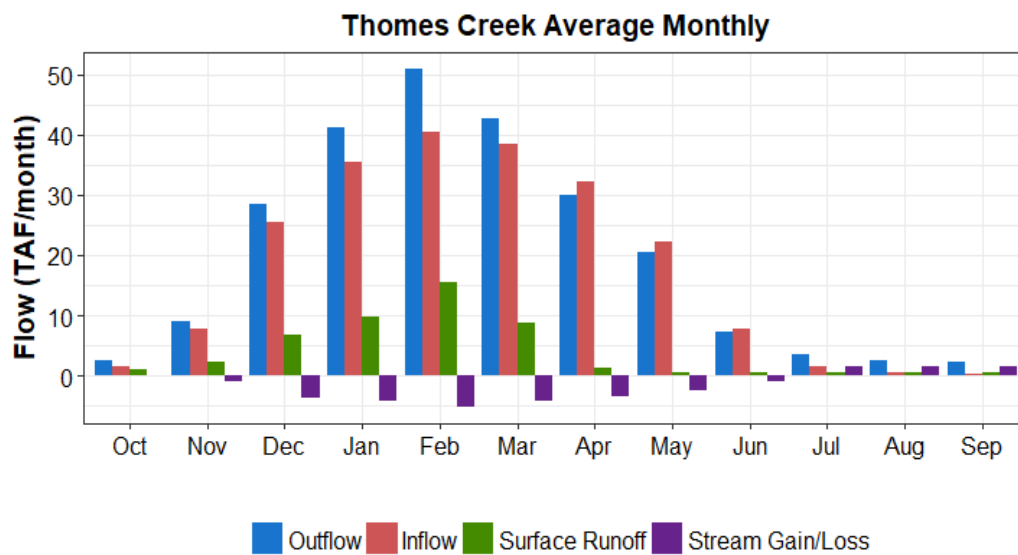
Figure A7-25. Monthly Average Unimpaired Flow Components for Thomes Creek
