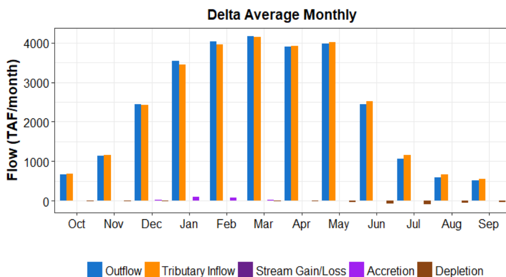
Figure A7-28. Monthly Average Unimpaired Flow Components for the Delta
