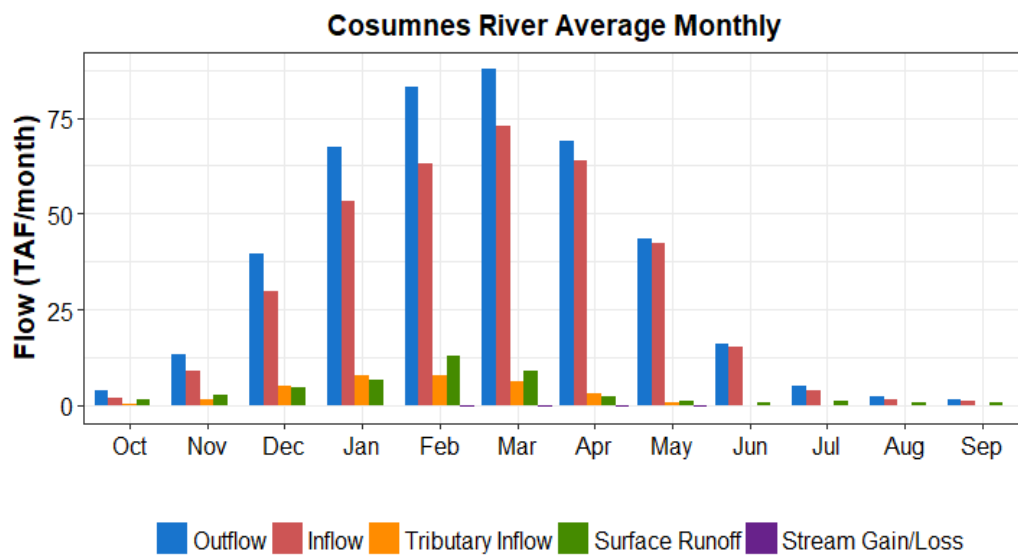
Figure A7-11. Monthly Average Unimpaired Flow Components for Cosumnes River
