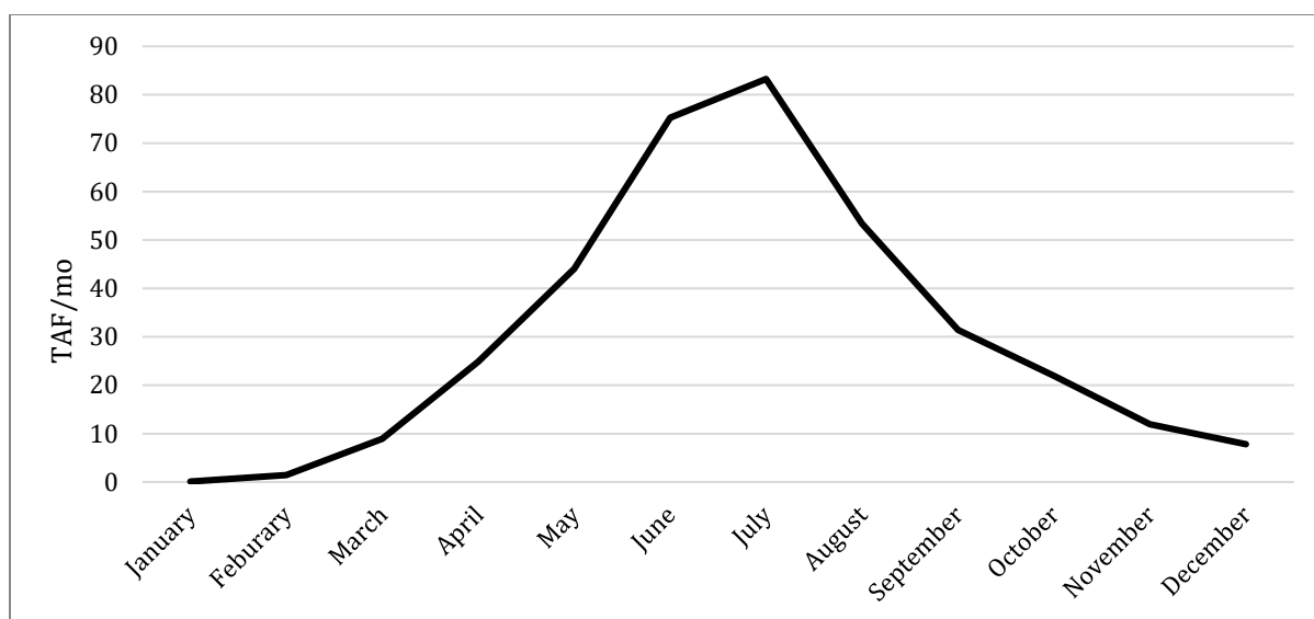
Figure A7-30. Monthly Average Total Delta Depletions
