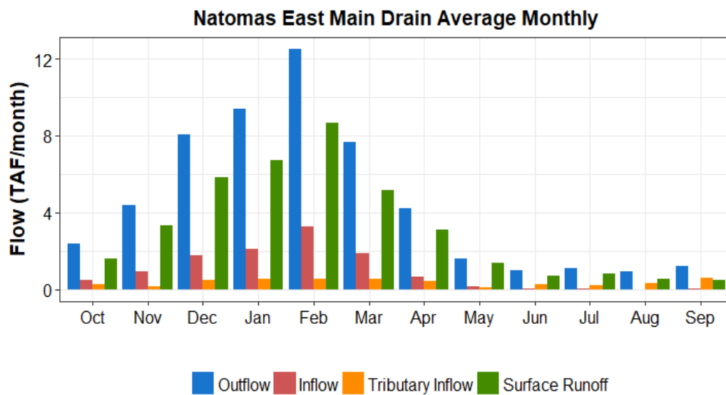
Figure A7-19. Monthly Average Unimpaired Flow Components for Natomas East Main Drain
