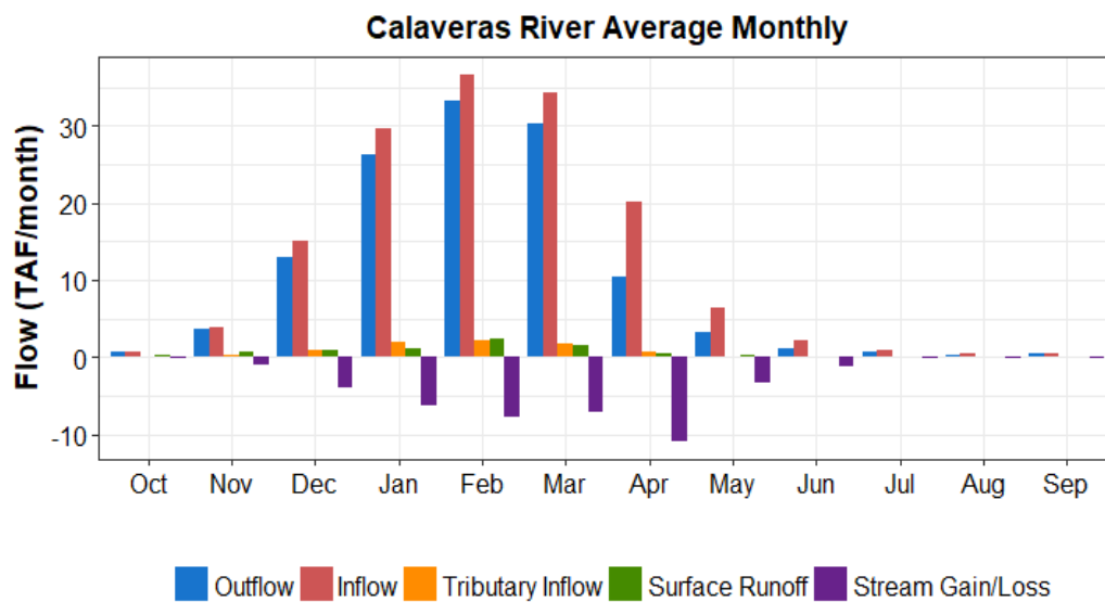
Figure A7-9. Monthly Average Unimpaired Flow Components for Calaveras River
