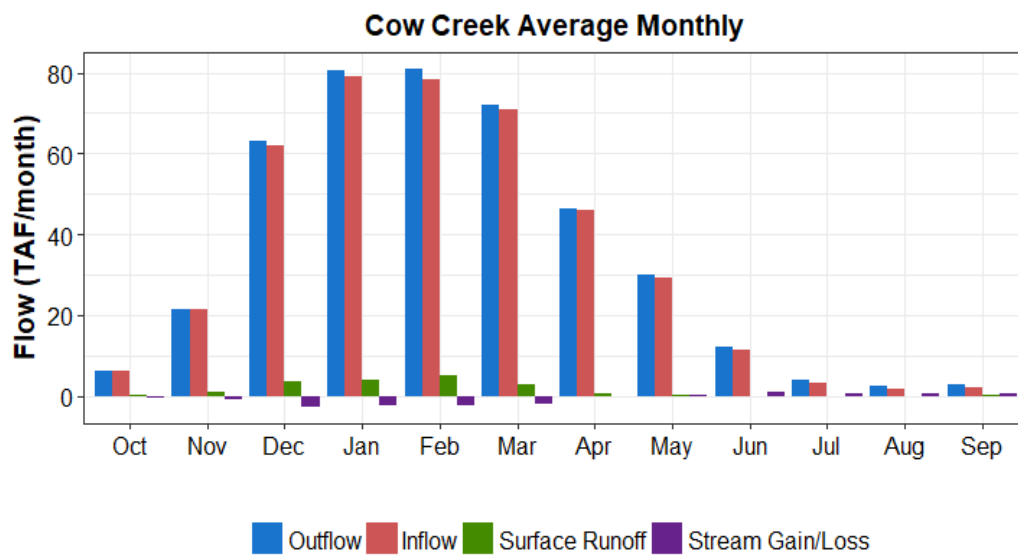
Figure A7-13. Monthly Average Unimpaired Flow Components for Cow Creek
