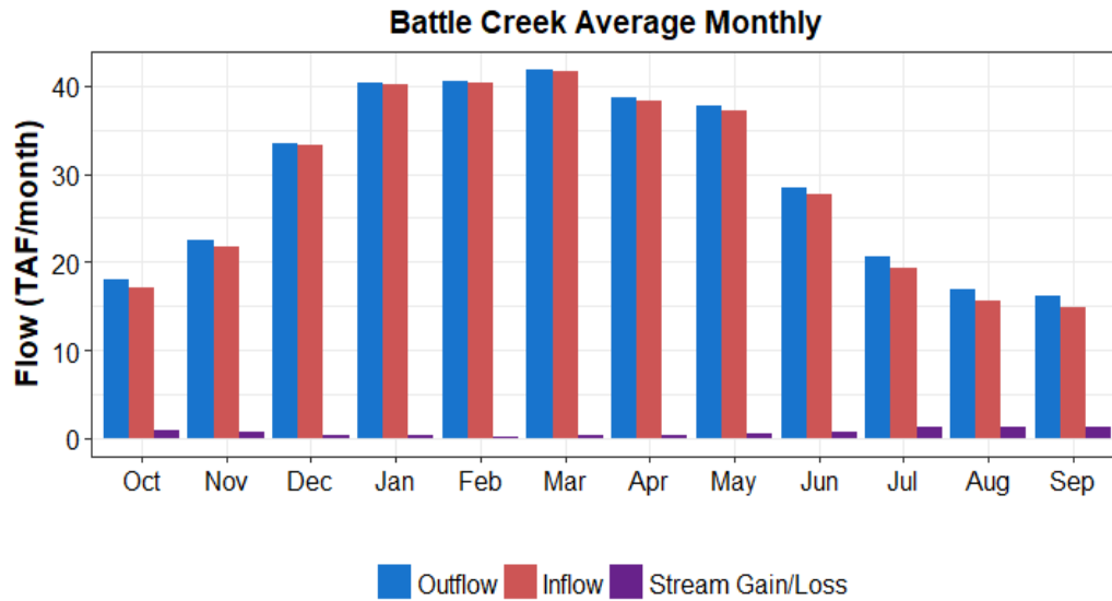
Figure A7-4. Monthly Average Unimpaired Flow Components for Battle Creek
