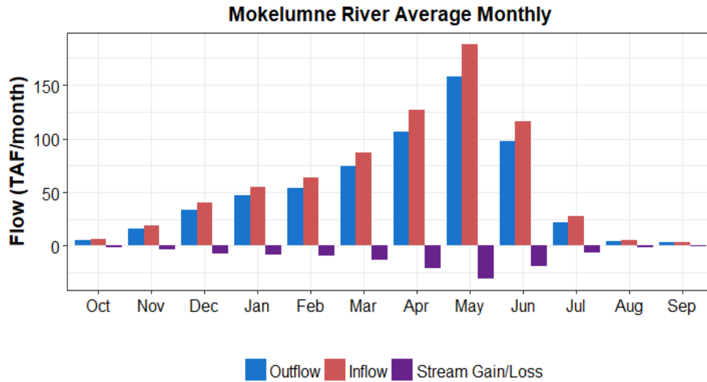
Figure A7-18. Monthly Average Unimpaired Flow Components for Mokelumne River
