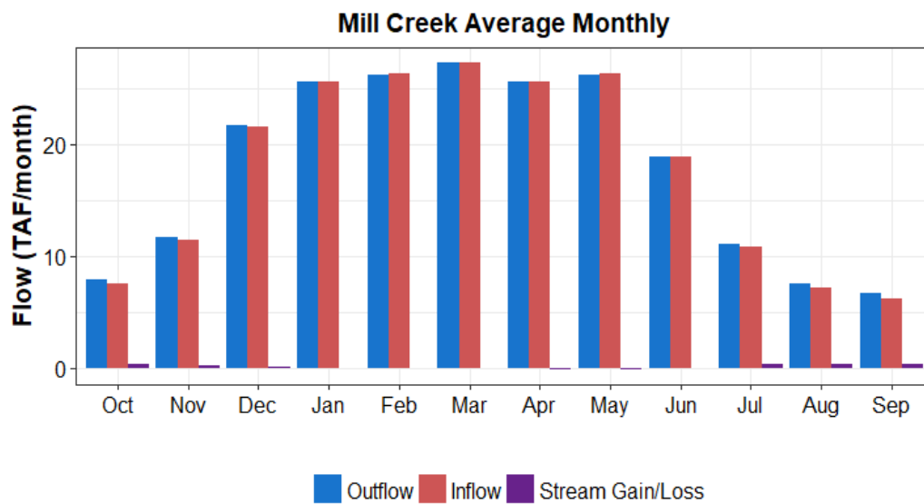
Figure A7-17. Monthly Average Unimpaired Flow Components for Mill Creek
