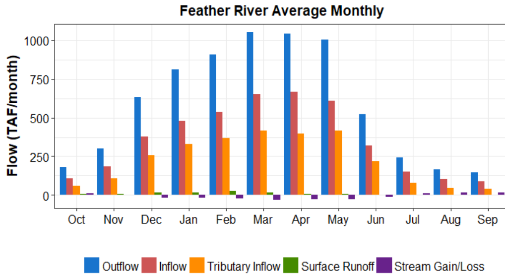
Figure A7-16. Monthly Average Unimpaired Flow Components for Feather River
