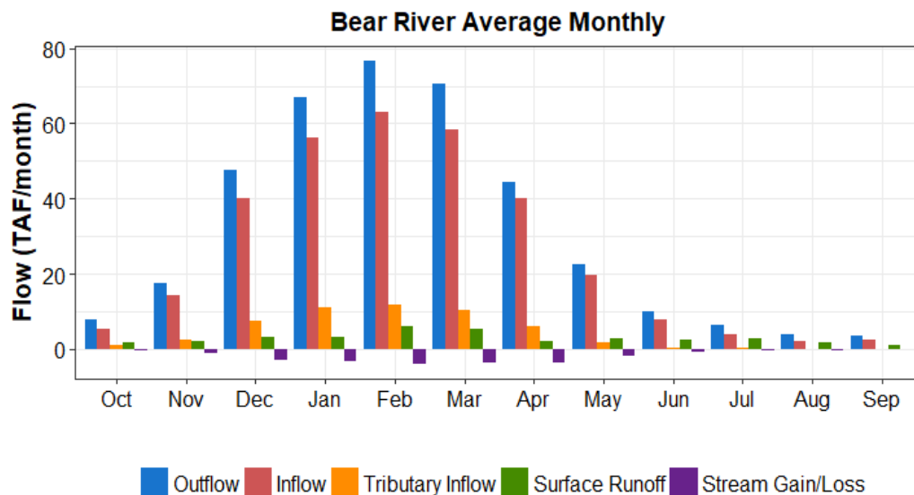
Figure A7-5. Monthly Average Unimpaired Flow Components for Bear River
