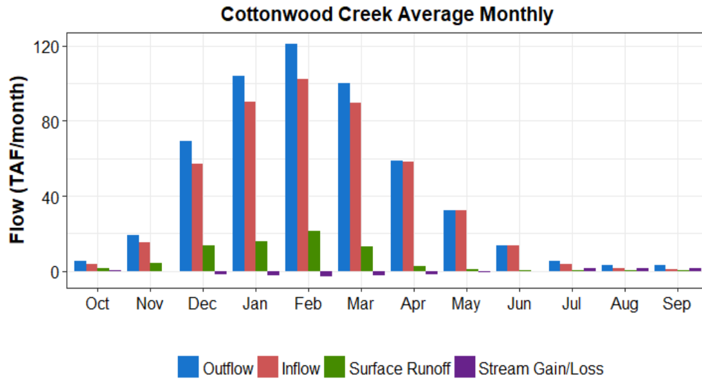
Figure A7-12. Monthly Average Unimpaired Flow Components for Cottonwood Creek
