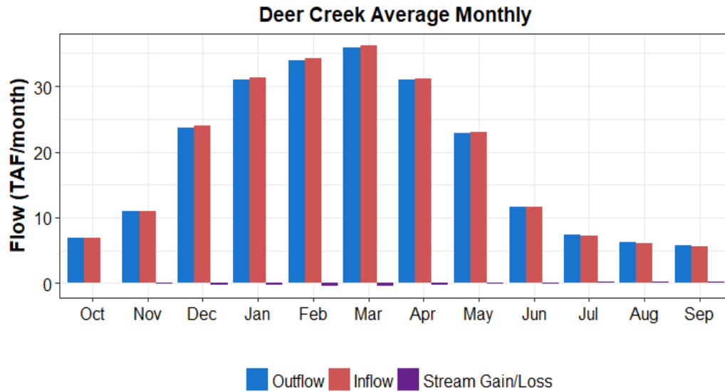
Figure A7-14. Monthly Average Unimpaired Flow Components for Deer Creek
