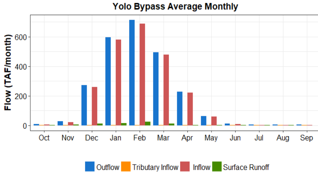
Figure A7-26. Monthly Average Unimpaired Flow Components for Yolo Bypass
