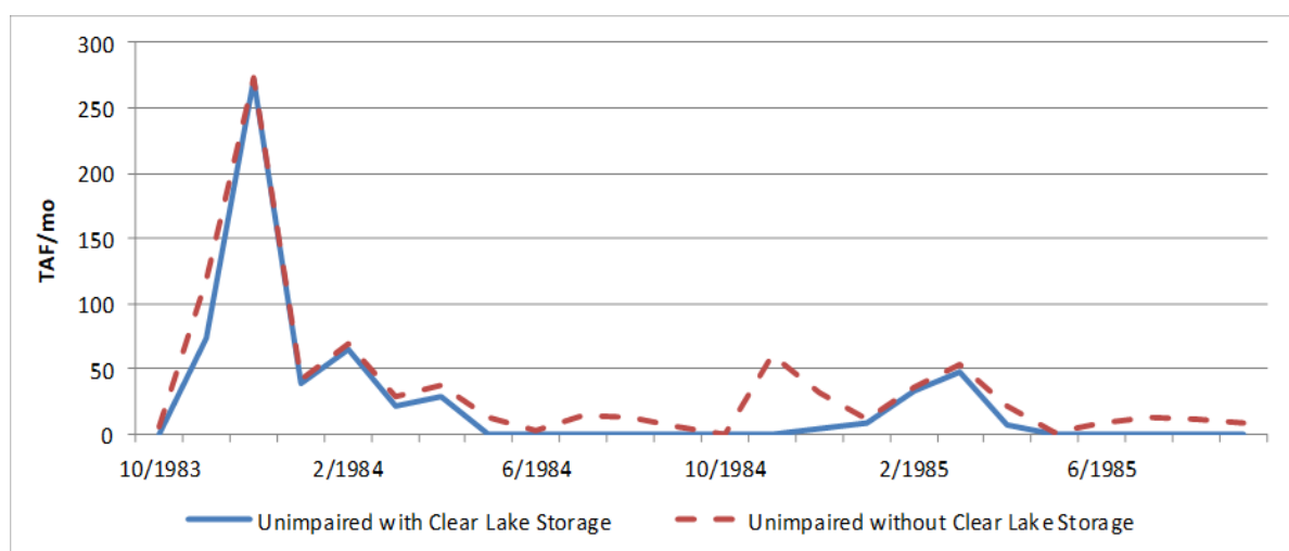
Figure A7-29. Monthly Unimpaired Flow on Cache Creek below Clear Lake for Water Years 1984–1985
