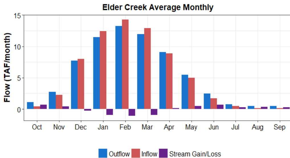
Figure A7-15. Monthly Average Unimpaired Flow Components for Elder Creek
