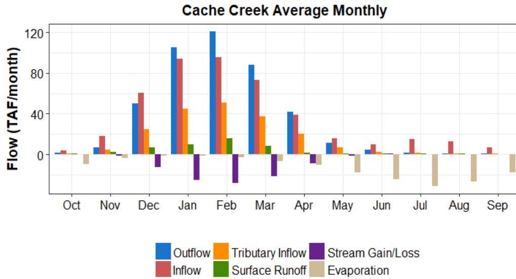
Figure A7-8. Monthly Average Unimpaired Flow Components for Cache Creek
