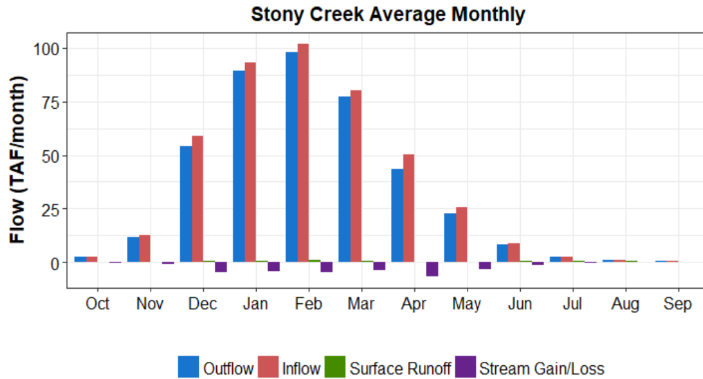
Figure A7-24. Monthly Average Unimpaired Flow Components for Stony Creek
