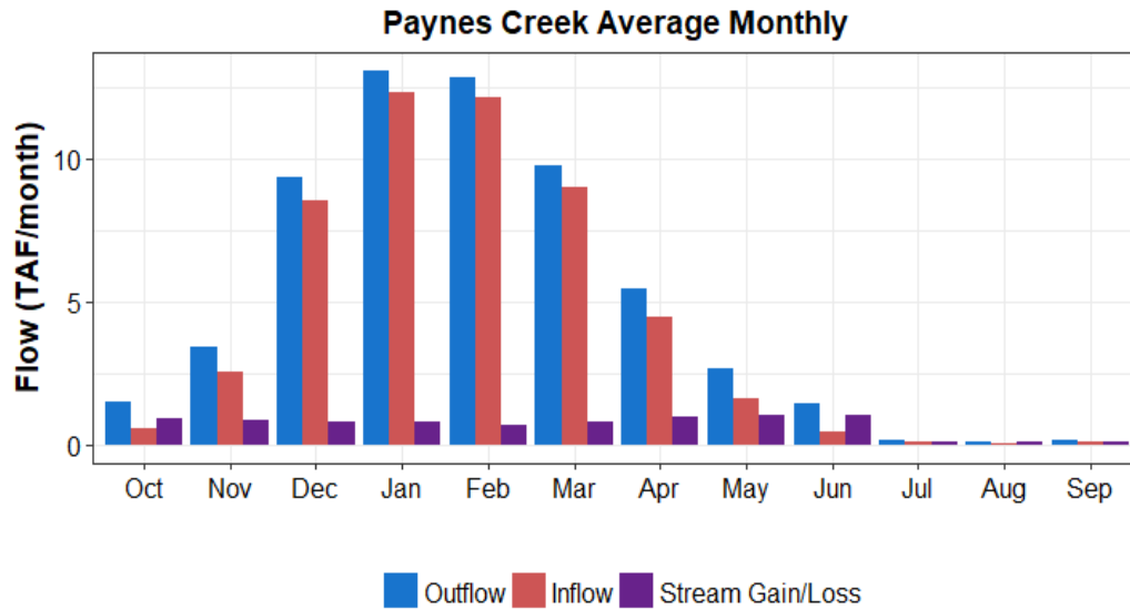
Figure A7-20. Monthly Average Unimpaired Flow Components for Paynes Creek
