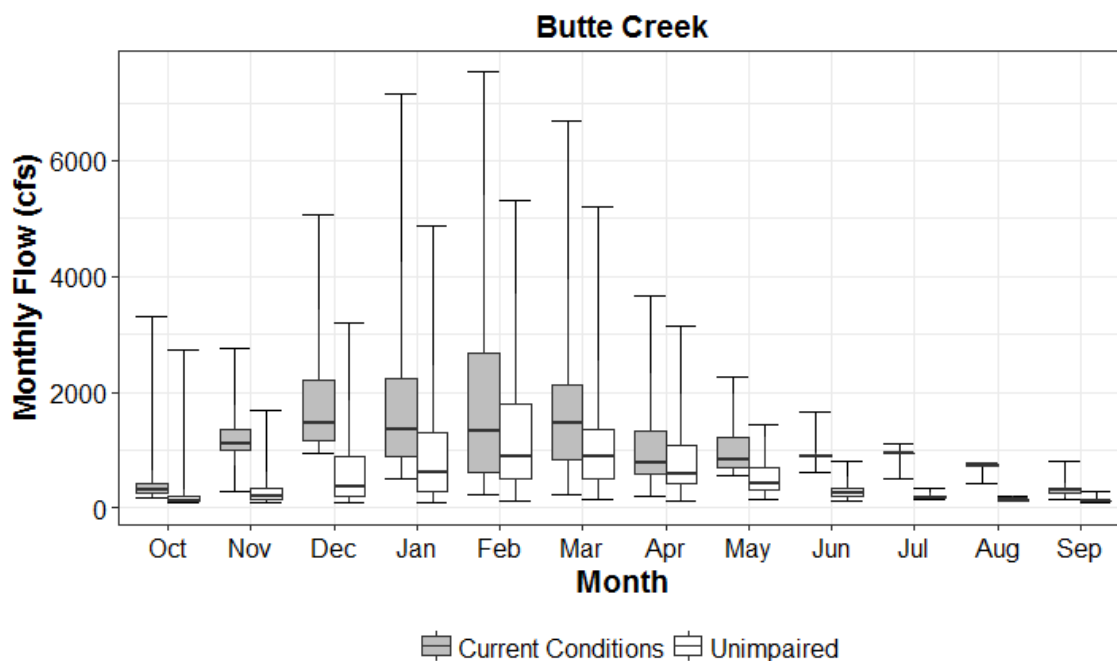
Figure 2.2-12. Butte Creek Simulated Current Conditions (gray) and Unimpaired (white) Monthly Flows
