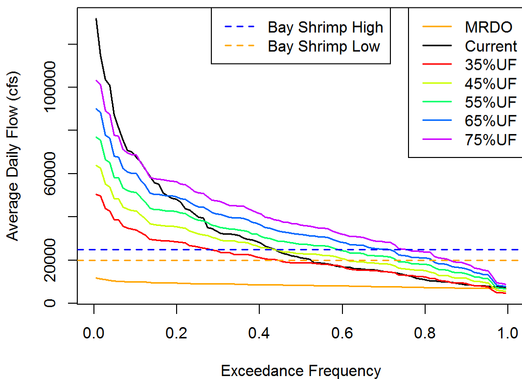
Figure 5.3-3. Frequency of Meeting March–May Delta Outflows to Benefit California Bay Shrimp for MRDO, Current Conditions as Modeled by SacWAM, and Inflow-Based Delta Outflow Scenarios Corresponding to Sacramento River and Eastside Delta Tributary Inflows from 35 to 75 Percent of Unimpaired Flow
