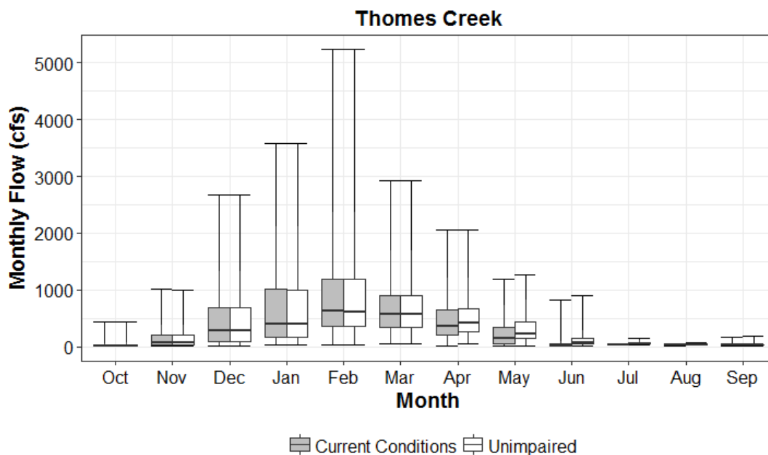
Figure 2.2-23. Thomes Creek Simulated Current Conditions (gray) and Unimpaired (white) Monthly Flows
