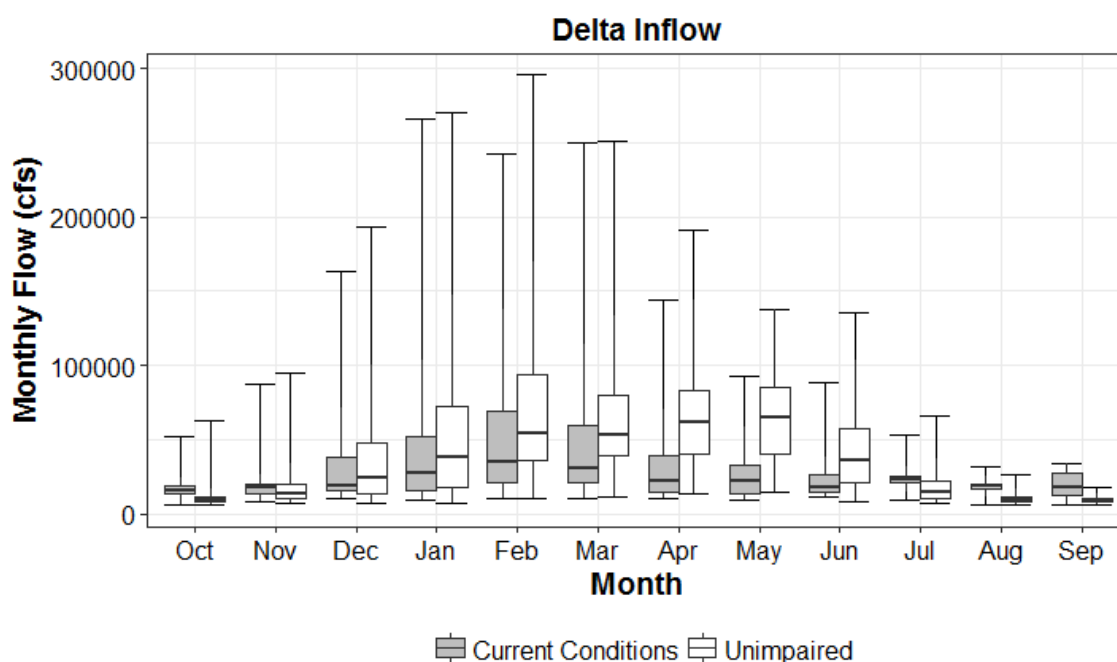
Figure 2.4-2. Delta Inflow Simulated Current Conditions (gray) and Unimpaired (white) Monthly Flows
