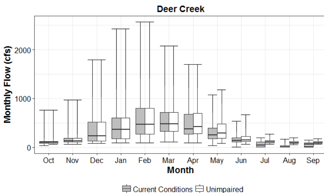
Figure 2.2-9. Deer Creek Simulated Current Conditions (gray) and Unimpaired (white) Monthly Flows
