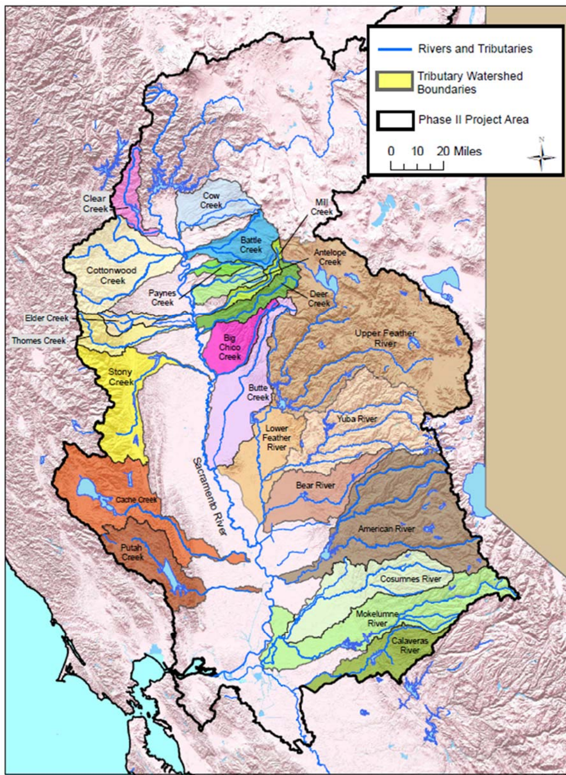
Figure 2.1-4. Major Tributaries and Watersheds in the Project Area
