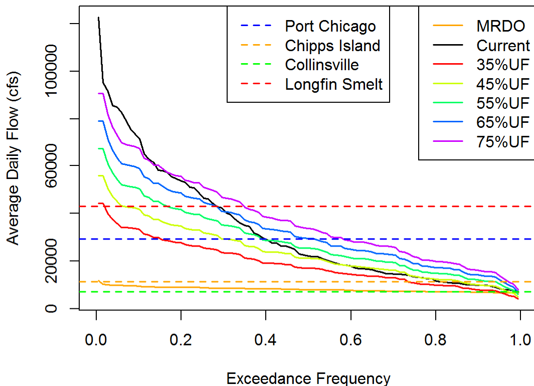
Figure 5.3-2. Frequency of Meeting January–June Delta Outflows to Benefit Estuarine LSZ Habitat and Longfin Smelt for MRDO, Current Conditions as Modeled by SacWAM, and Inflow-Based Delta Outflow Scenarios Corresponding to Sacramento River and Eastside Delta Tributary Inflows from 35 to 75 Percent of Unimpaired Flow
