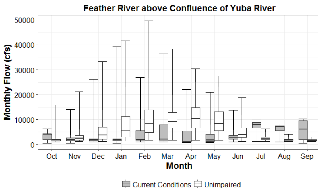
Figure 2.2-13. Feather River above Confluence with the Yuba River Simulated Current Conditions (gray) and Unimpaired (white) Monthly Flows
