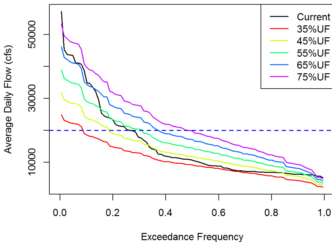
Figure 5.2-1. Frequency of Meeting April–June Sacramento River at Rio Vista Flows of 20,000 cfs for Current Conditions as Modeled by SacWAM, and 35 to 75 Percent of Unimpaired Flow at Rio Vista
