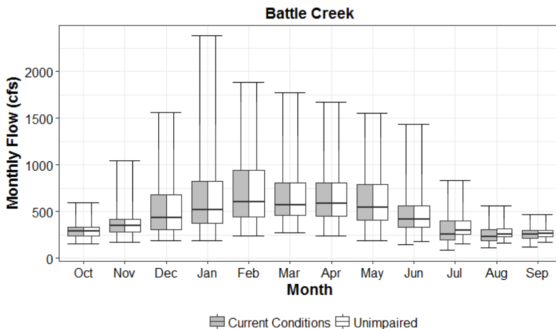
Figure 2.2-6. Battle Creek Simulated Current Conditions (gray) and Unimpaired (white) Monthly Flows
