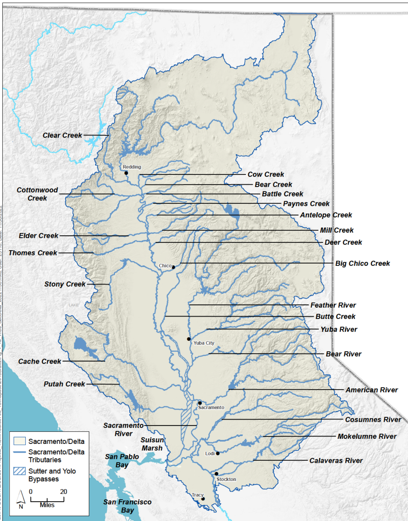
Figure 1-1a Sacramento/Delta Tributaries
