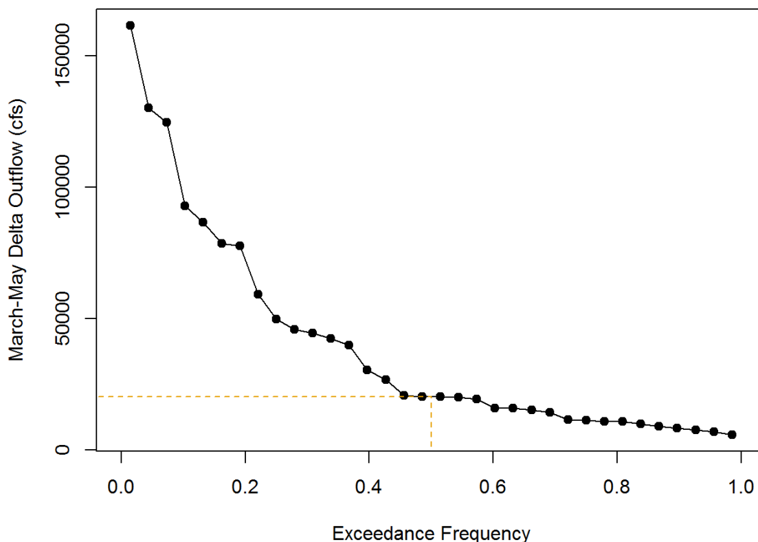
Figure 3.10-3. Cumulative Frequency Distribution of Average Daily Outflow for March–May, 1980–2013
