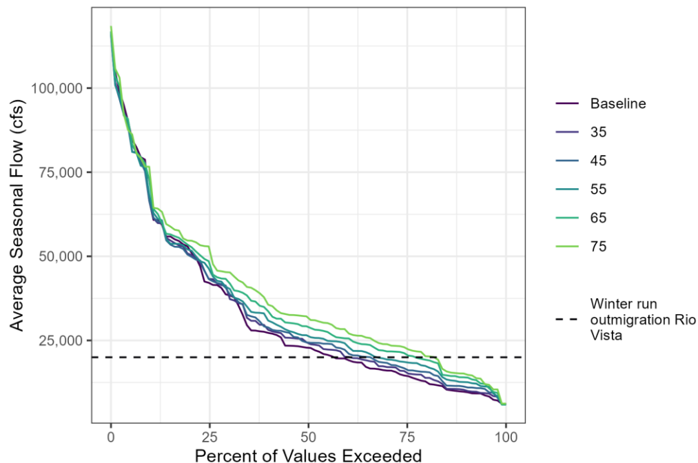
Figure 3.14-2. Frequency of Meeting April–June Sacramento River at Rio Vista Flows of 20,000 cfs for Current Conditions
