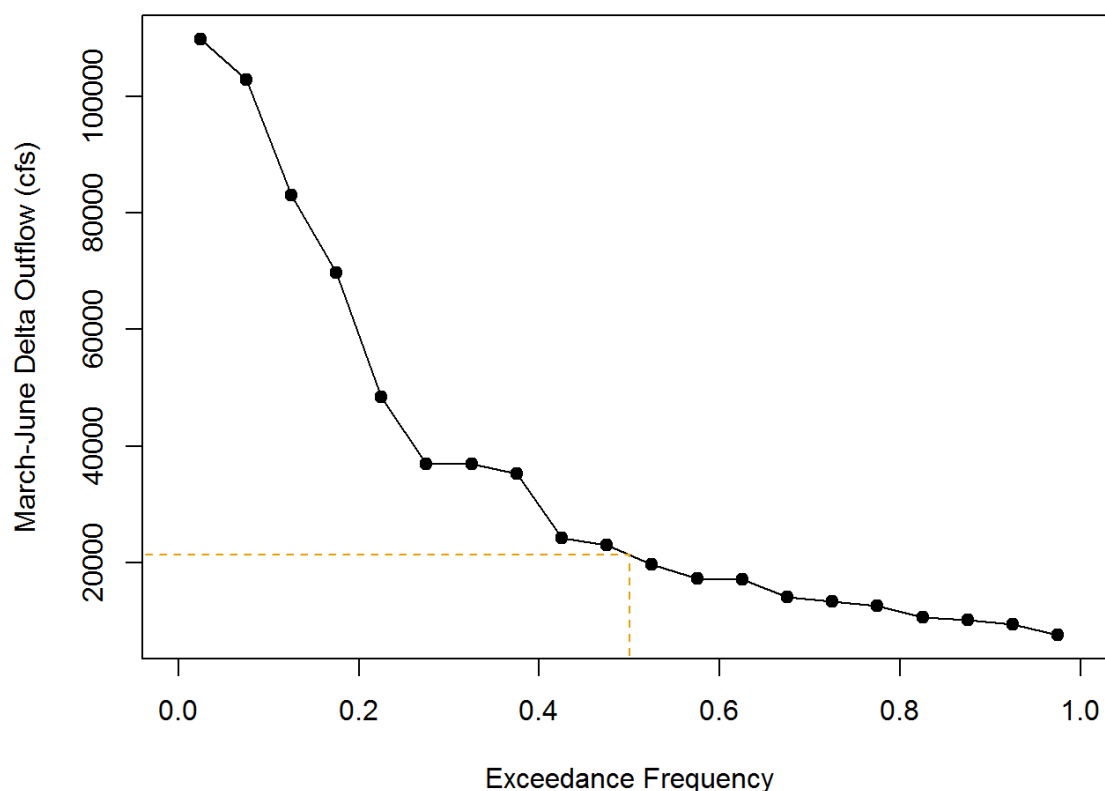
Figure 3.9-3. Cumulative Frequency Distribution of Monthly Average Daily Delta Outflow for March through June, 1994–2013
