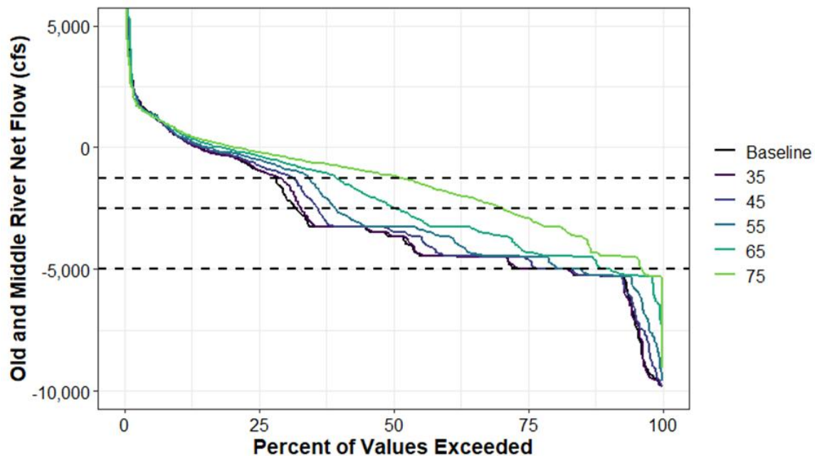
Figure 3.14-11. Frequency of Meeting Old and Middle River Reverse Flow Thresholds to Protect Salmonids and Estuarine-Dependent Fish Species during December through June under Range of Flow Scenarios
