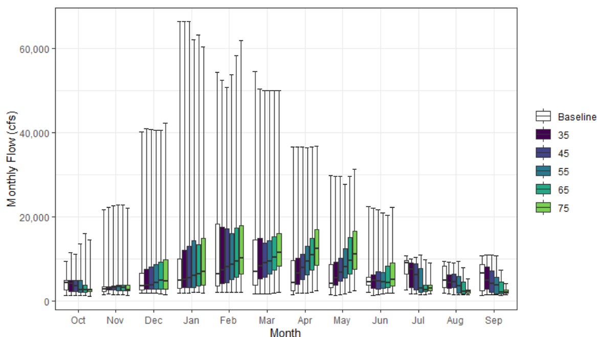
Figure 7.6.2-6. SacWAM Results for Feather River Flows (SWRCB Feather River) for Baseline Condition and 35 to 75 Scenarios
