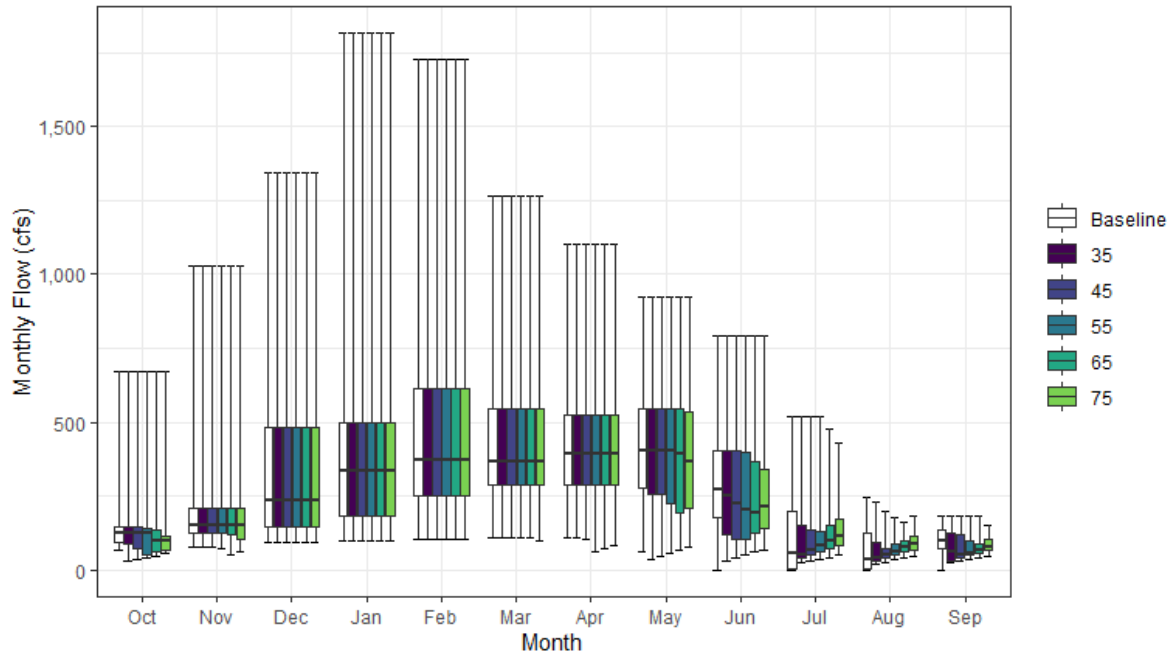
Figure 7.6.2-12. SacWAM Results for Mill Creek Flows (SWRCB Mill Creek) for Baseline Condition and 35 to 75 Scenarios
