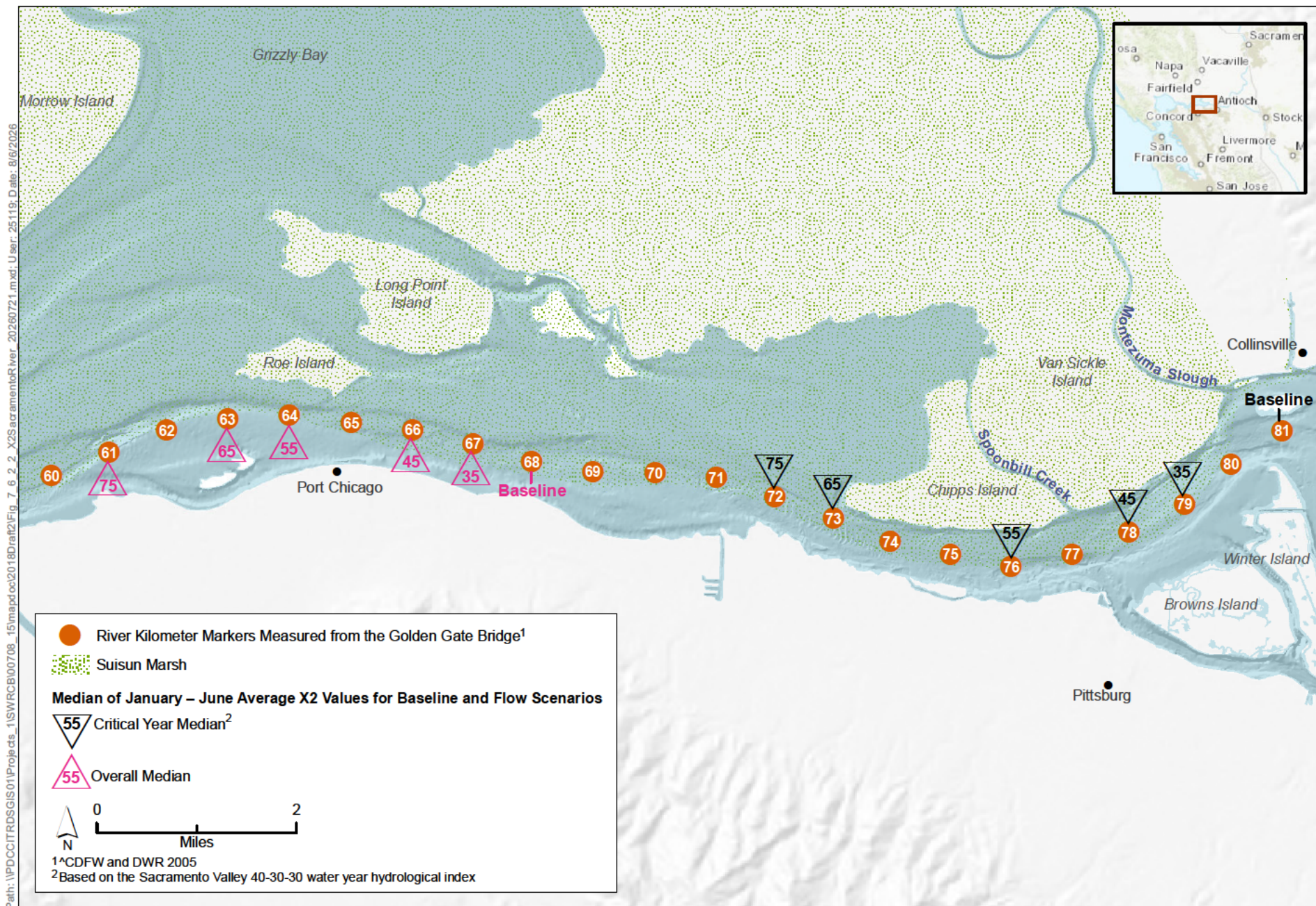
Figure 7.6.2-2 X2 Position for Baseline and Flow Scenarios Presented as Median of the January through June Average Values
