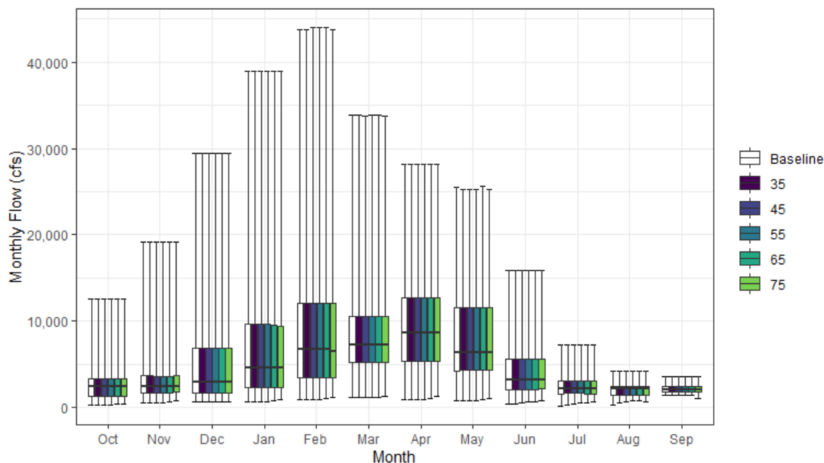
Figure 7.6.2-9. SacWAM Results for Feather River above Oroville Reservoir (SWRCB Oroville Inflow)
