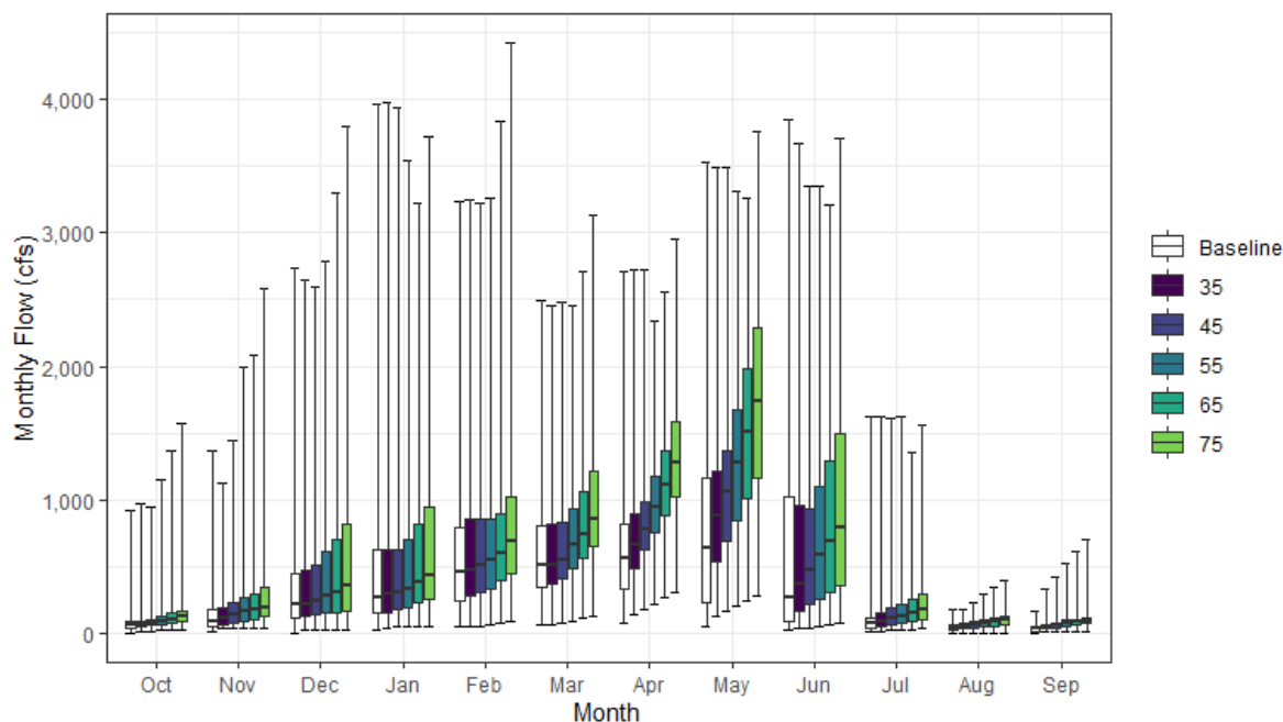
Figure 7.6.2-10. SacWAM Results for South Yuba River above Englebright Reservoir Flows (SWRCB S Yuba Inflow) for Baseline Condition and 35 to 75 Scenarios
