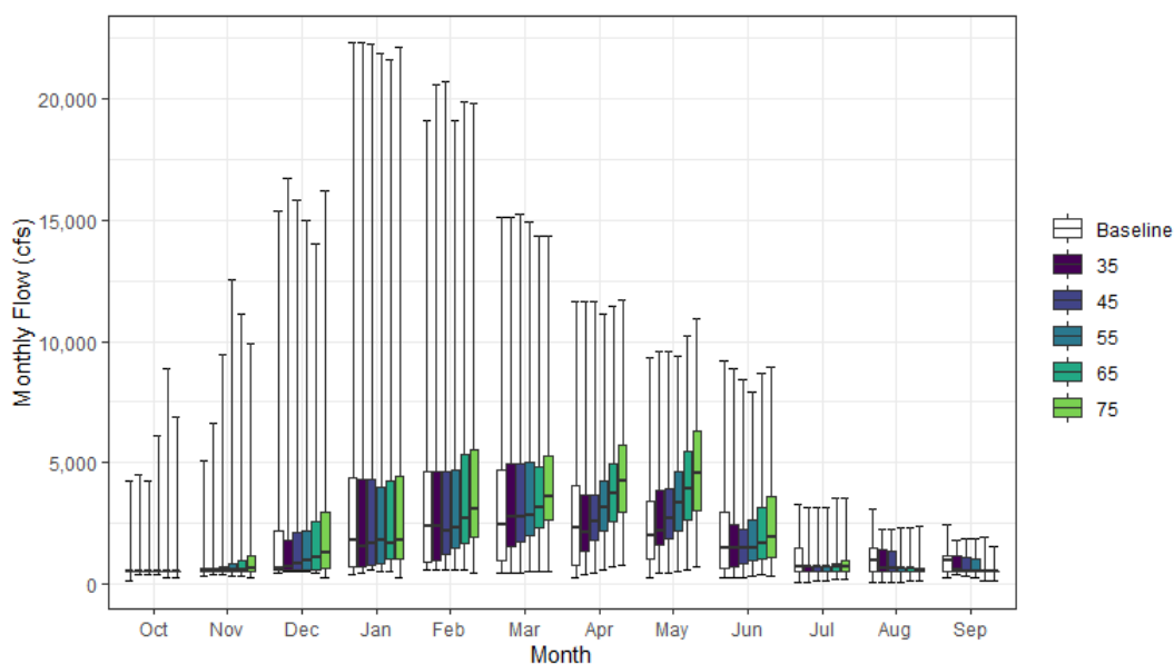
Figure 7.6.2-8. SacWAM Results for Lower Yuba River Flows (SWRCB Yuba River) for Baseline Condition and 35 to 75 Scenarios
