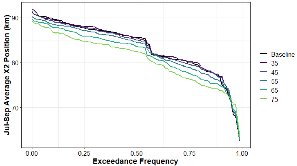
Figure 7.6.2-4. SacWAM Results for July–September Average X2 Positions for Baseline and 35 to 75 Scenarios
