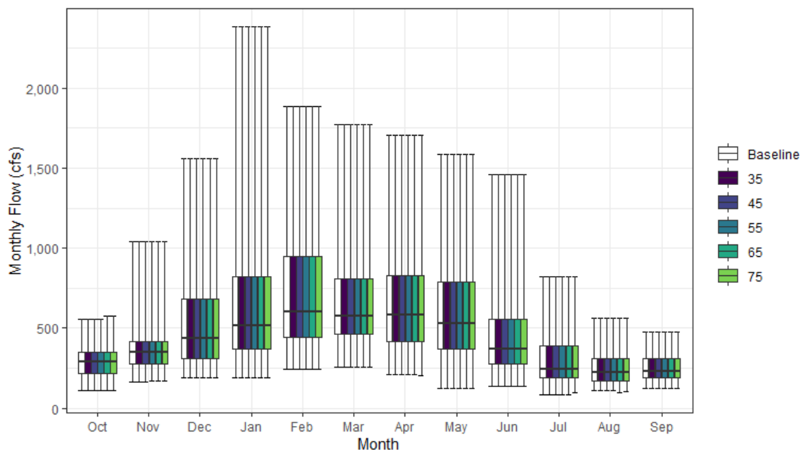
Figure 7.6.2-11. SacWAM Results for Battle Creek Flows (SWRCB Battle Creek) for Baseline Condition and 35 to 75 Scenarios
