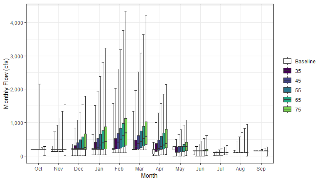
Figure 7.6.2-7. SacWAM Results for Lower Clear Creek Flows (SWRCB Clear Creek) for Baseline Condition and 35 to 75 Scenarios
