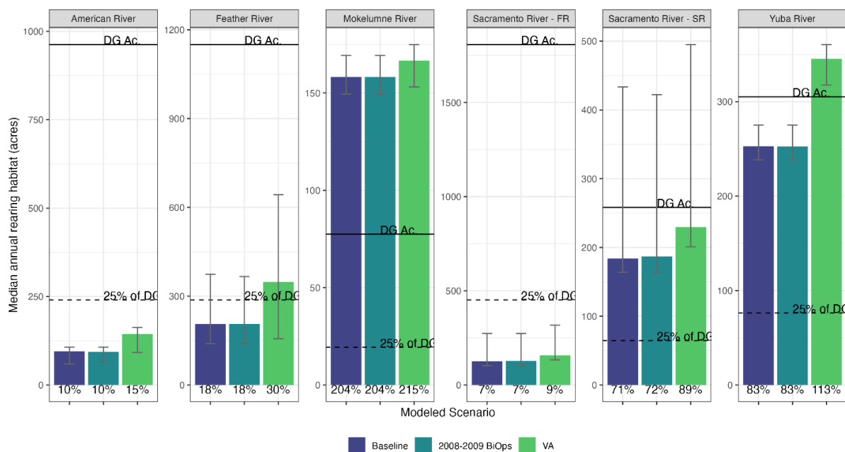
Figure 9.6-2. Median (across All Years) Rearing Habitat (Acres) under 2008–2009 BiOps Condition and VA Scenarios for Each Watershed, Including Both Floodplain and In-Channel Rearing Habitat
