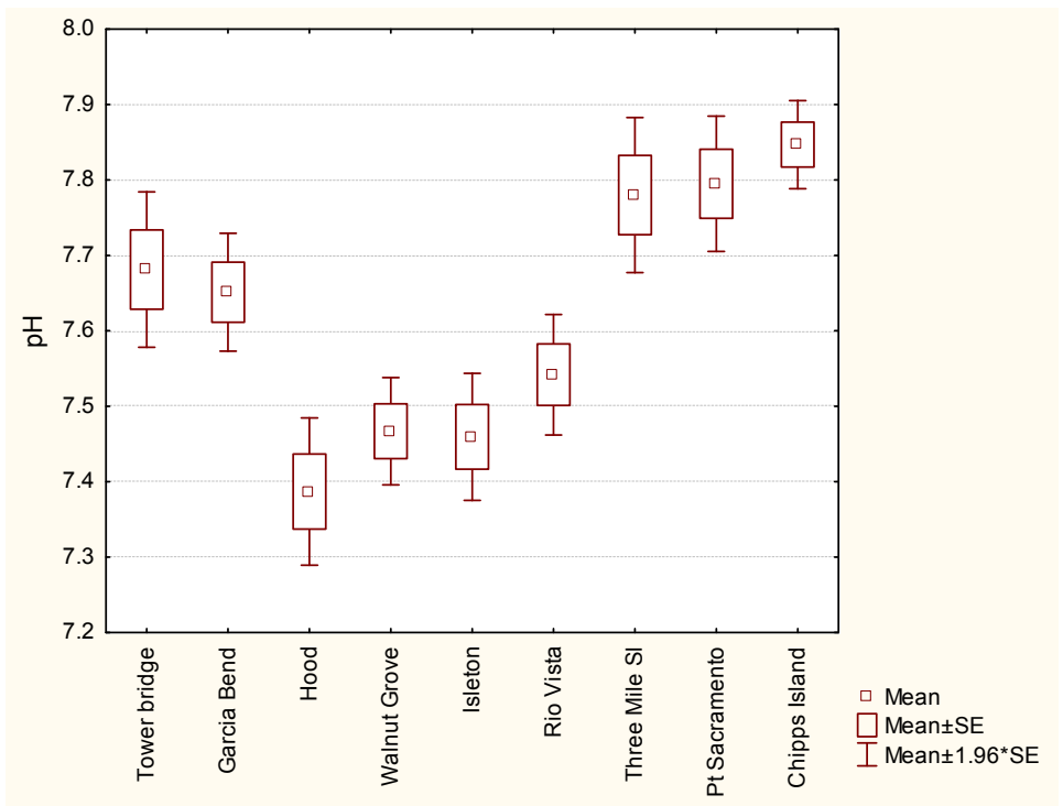
Figure 6. Average pH values down the Sacramento River and across the Delta to Chipps Island. The SRWTP discharges between Garcia Bend and Hood.
