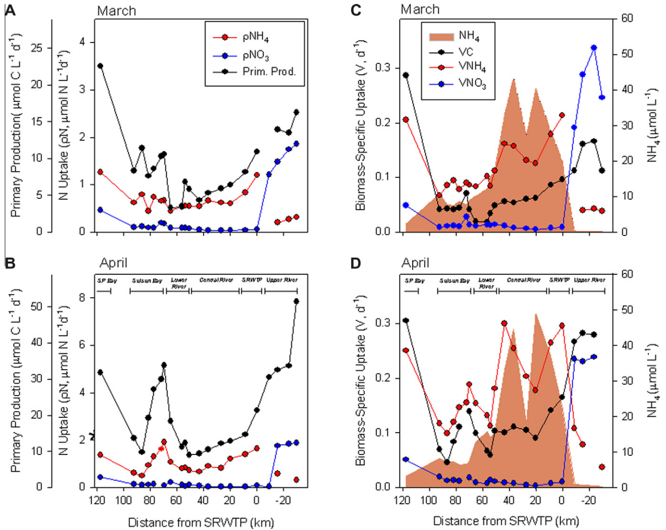
Fig. 5. Primary production and phytoplankton nitrogen uptake in the Sacramento River and Northern SFE during (A) March and (B) April 2009. Biomass-specific carbon uptake and phytoplankton nitrogen uptake and \text{NH}_4 concentrations (shaded area) during (C) March and (D) April 2009. Y-axes for phytoplankton C and N uptake are scaled at 6.6 C:1 N (i.e. the Redfield ratio).
