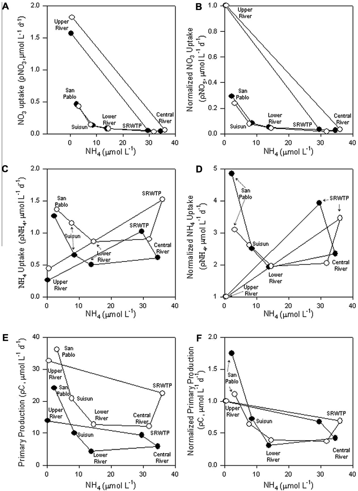
Fig. 7. River and estuary region means of C, \text{NO}_3 and \text{NH}_4 uptake versus \text{NH}_4 concentrations in the Sacramento River and the Northern SFE. (A, C, E) nitrate uptake ( \rho\text{NO}_3 ), ammonium uptake ( \rho\text{NH}_4 ), and carbon uptake ( \rho\text{C} ). (B, D, F) The same data with uptake rates normalized to Upper River region mean uptake ( \rho ) rates.
