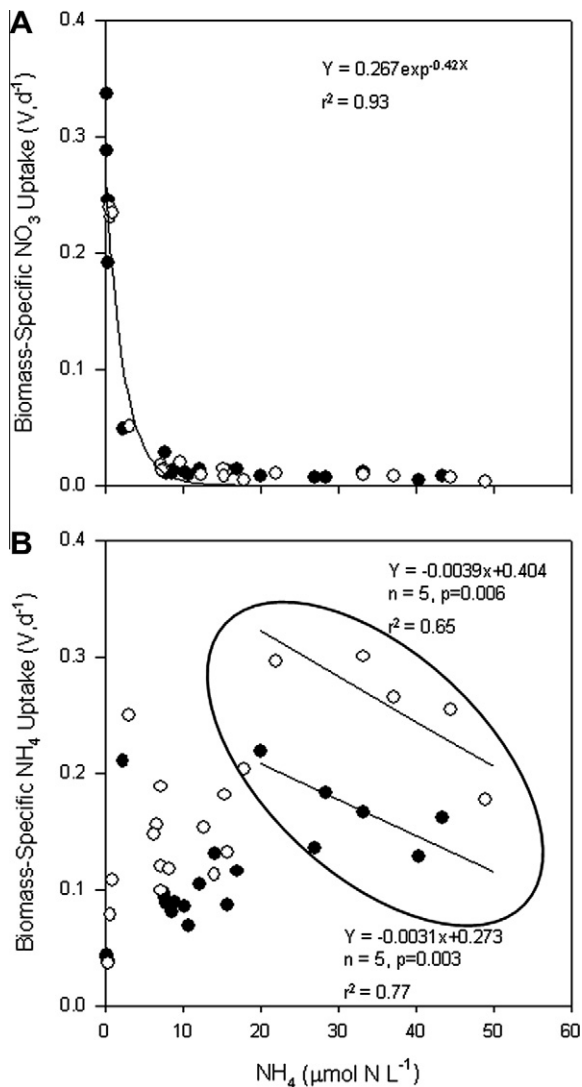
Fig. 6. Effect of \text{NH}_4 concentration on phytoplankton N uptake processes in the Sacramento River and Northern Sacramento River. (A) Biomass-specific \text{NO}_3 uptake rate ( \text{VNO}_3 ) and (B) biomass-specific \text{NH}_4 uptake rate ( \text{VNH}_4 ) versus \text{NH}_4 concentrations measured during March (closed circles) and April (open circles) 2009. Linear regression shown in panel B is based on the five stations occupied in the SRWTP and Central River regions (RM44, HOD, KEN, L37, ISL).
