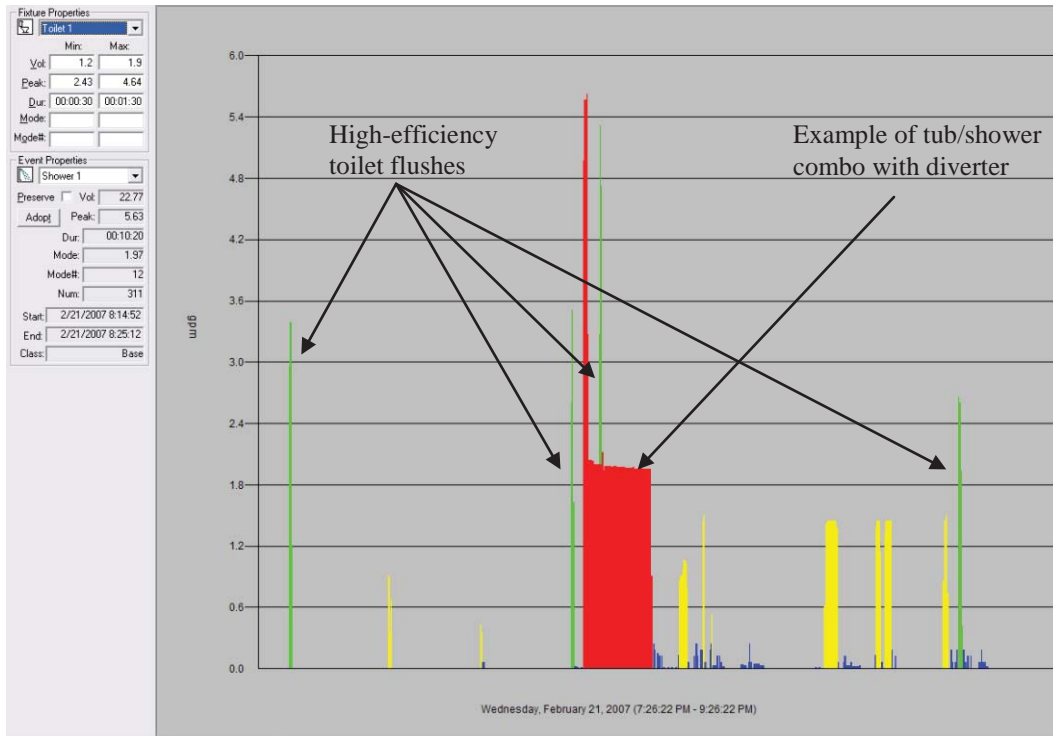
Figure 16: Classic profile of tub/shower combo with HE toilet events and some faucet use
