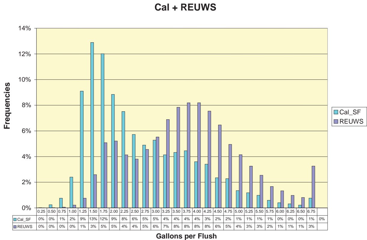
Figure 4: Comparison of toilet flush histograms of California SF Study to REUWS
