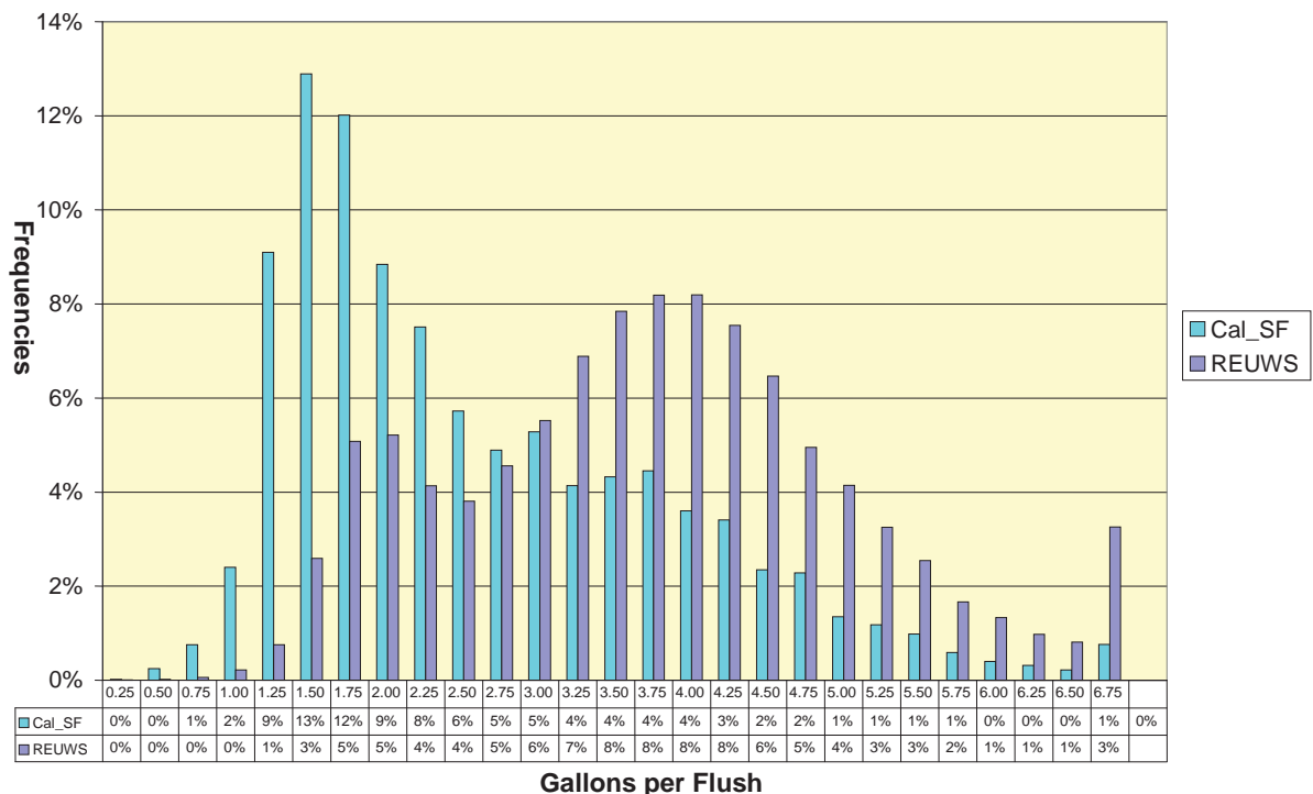
Figure 43: California Single-Family Homes vs. REUWS toilet flush volume distributions
