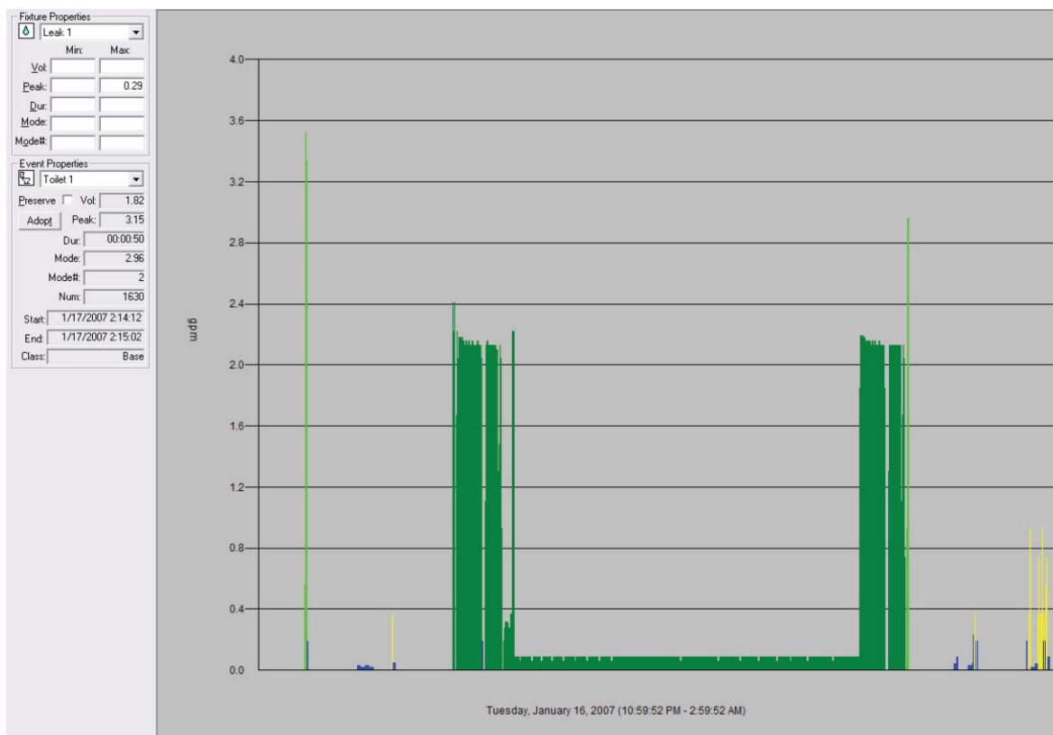
Figure 19: An example of a residential water softener in Trace Wizard
