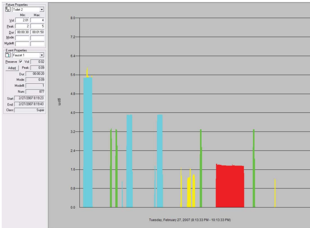
Figure 17: Profile typical of a stall shower with clothes washer, faucet, and toilet events
