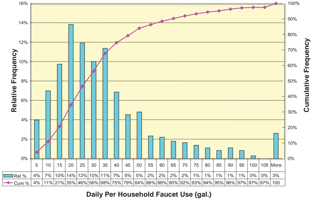
Figure 52: Distribution of daily faucet use (gphd)
