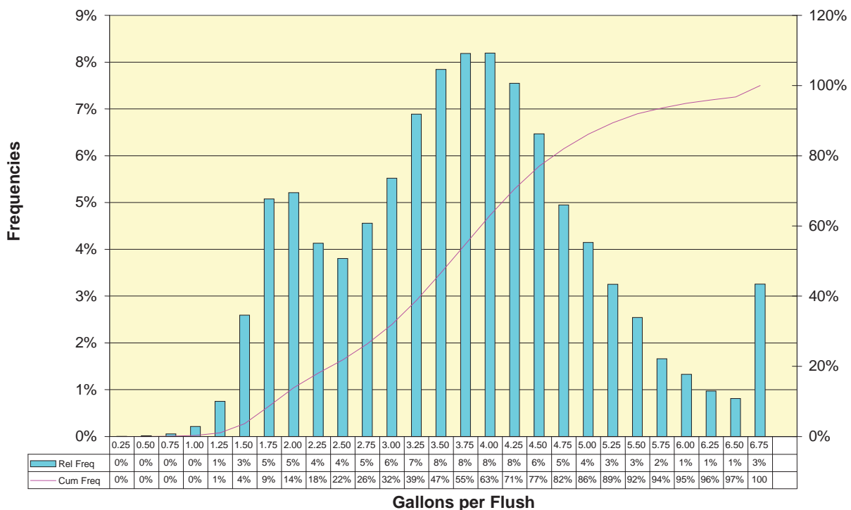
Figure 42: Histogram of toilet flushes from REUWS study group
