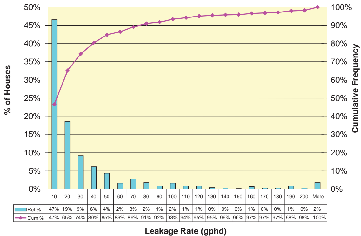
Figure 50: Percent of homes by leakage rate
