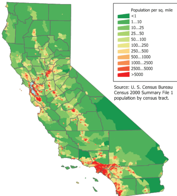
Figure 73: Population intensities 56
