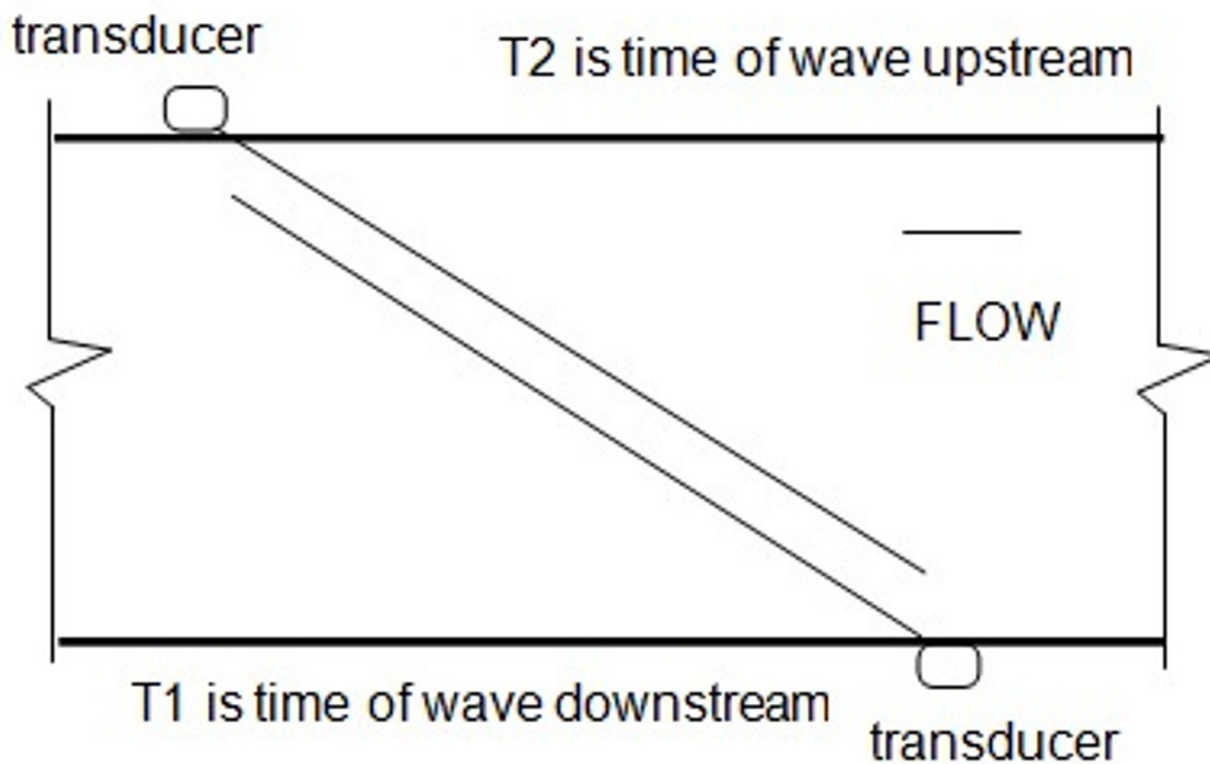
Figure 3. Acoustic Meter (Transit time style in pipeline)
