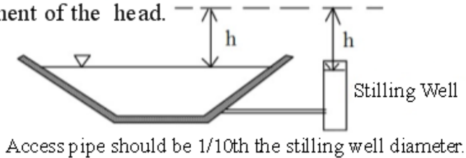
Figure 4. Stilling well used for open channel flow
