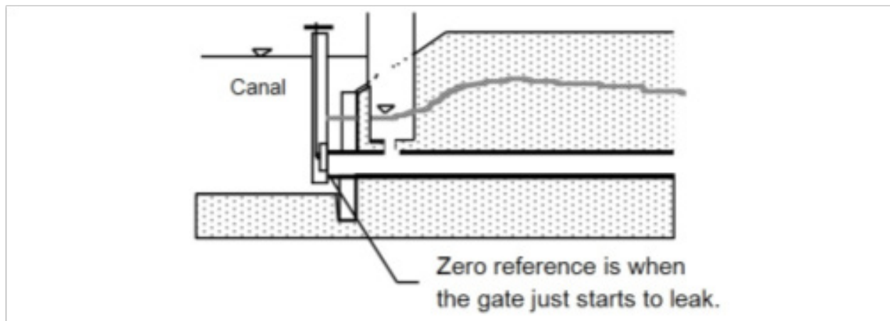
Figure 4. Stilling well used for open channel flow
