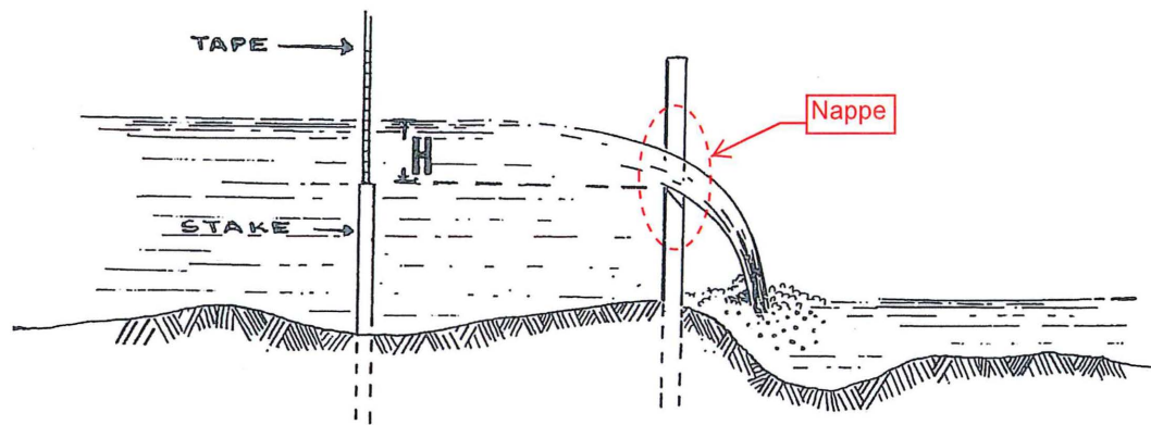
Measuring head on a weir. Measure upstream from downward curve of the water surface.
