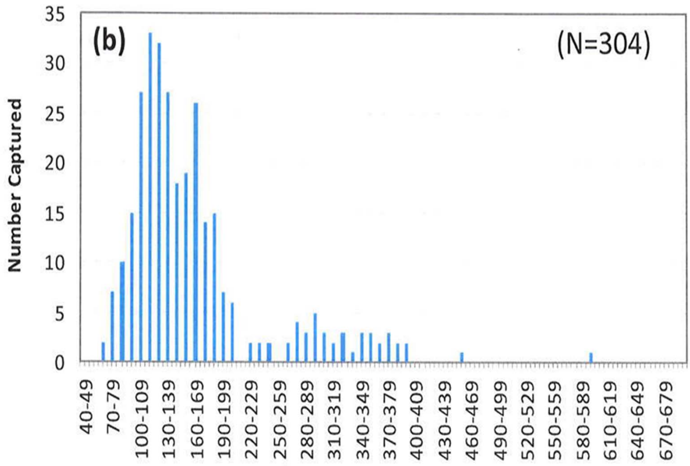
Figure 32: WY2009 Hilton Creek trap length-frequency histogram in 10-millimeter intervals for (a) upstream and (b) downstream migrant captures.
