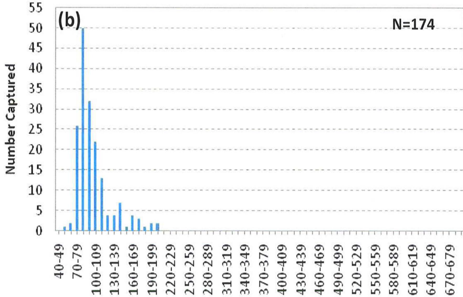
Figure 37: WY2009 Salsipuedes Creek trap length-frequency histogram in 10-millimeter intervals for (a) upstream and (b) downstream migrant captures.
