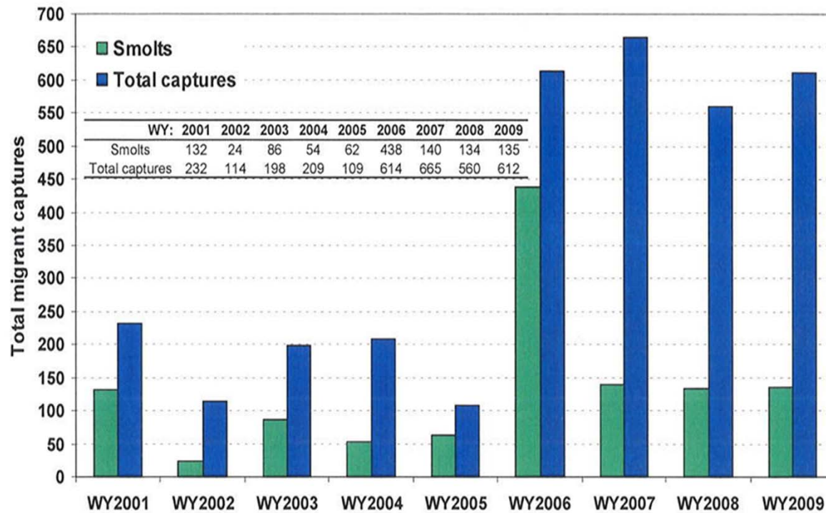
Figure ES-2: Total downstream smolts and migrant upstream and downstream O. mykiss captures at the three trapping sites within the LSYR basin from WY2001 to WY2009.
