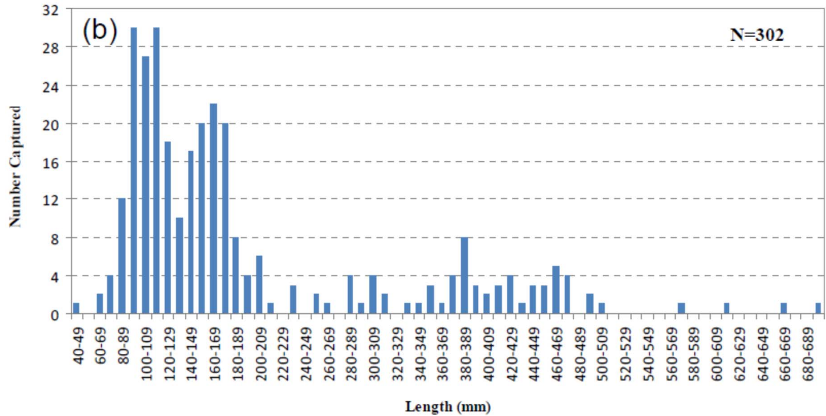
Figure 31: WY2008 Hilton Creek trap length-frequency histogram in 10 millimeter intervals for the (a) upstream and (b) downstream migrant captures.
