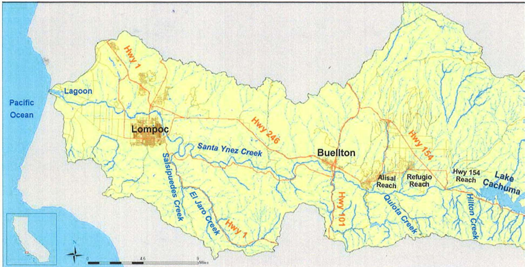
Figure ES-1: LSYR from Bradbury Dam and Lake Cachuma to the Pacific Ocean to the west of Lompoc showing tributary creeks and management reaches of interest for the LSYR Fisheries Monitoring Program.
