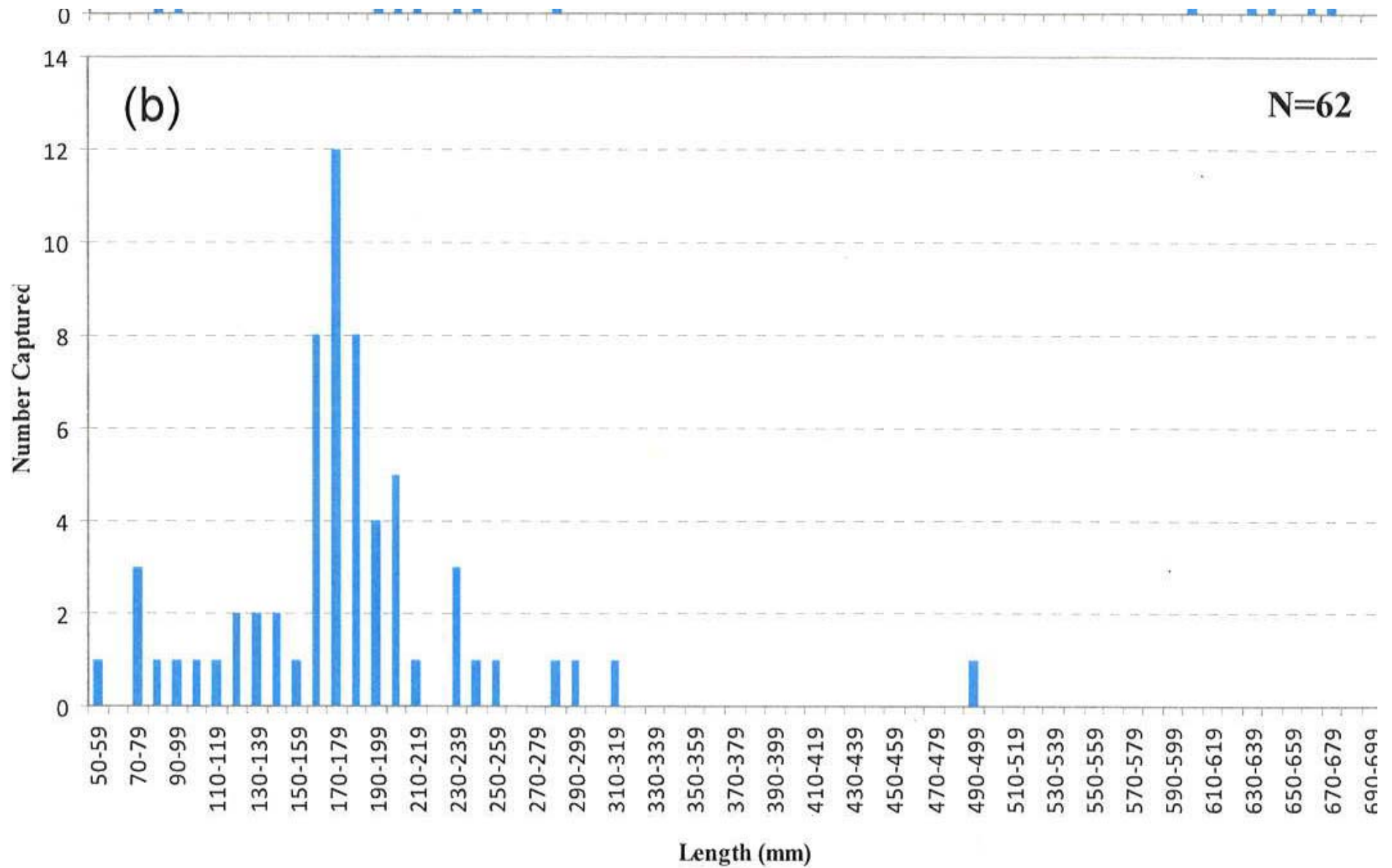
Figure 35: WY2008 Salsipuedes Creek trap length-frequency histogram in 10 millimeter intervals for (a) upstream and (b) downstream migrant captures.
