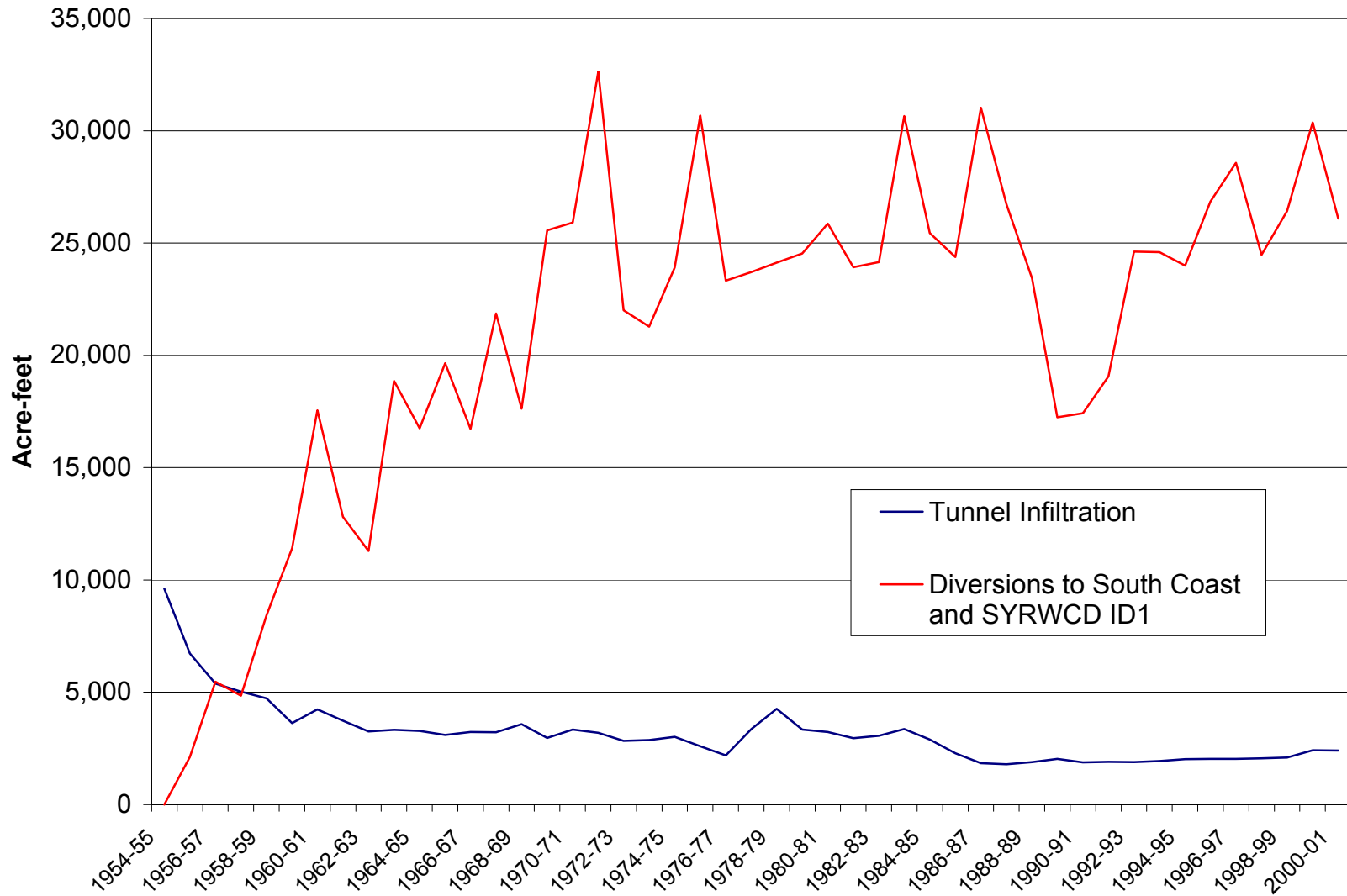
Chart 3-1. Historic Deliveries from the Cachuma Project
