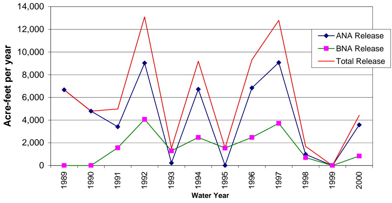
Chart 3-3. Historical Annual ANA and BNA Releases under WR 89-18
