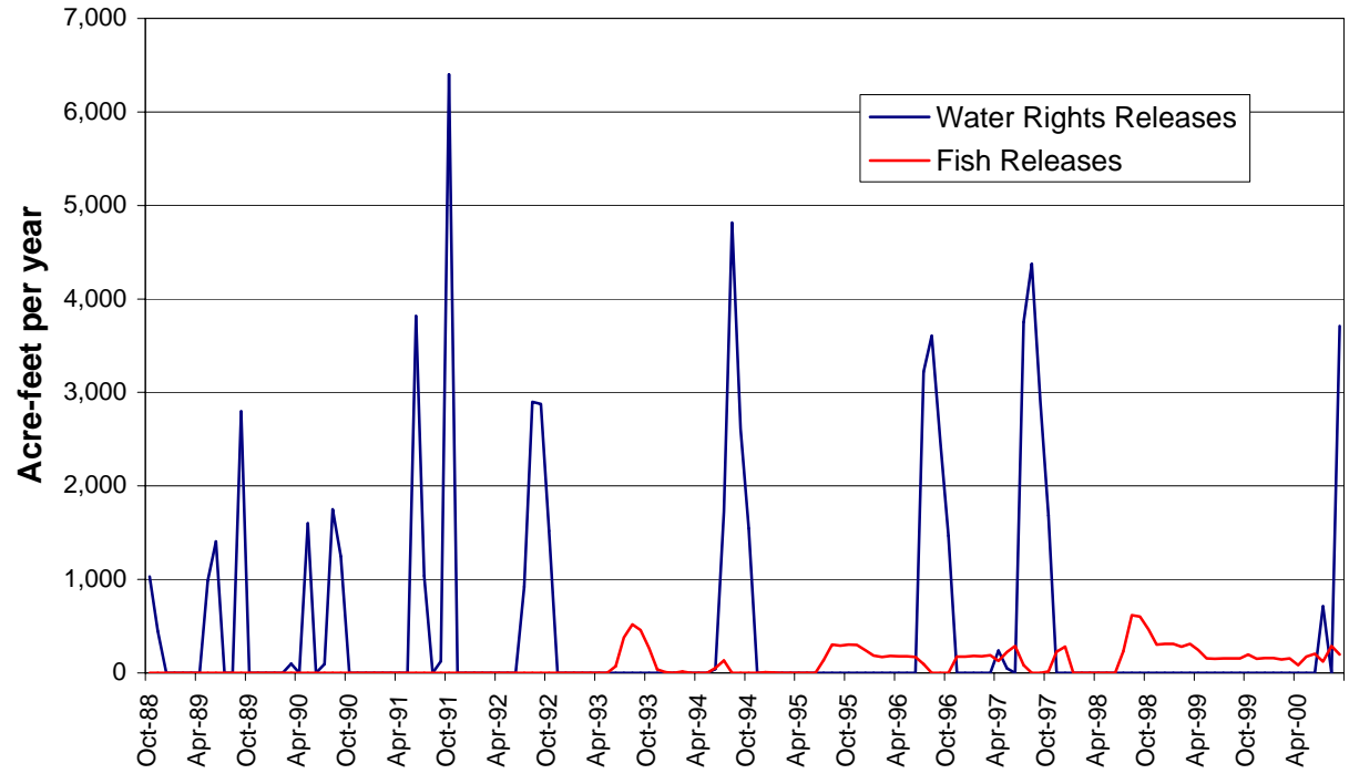
Chart 3-4. Historical Monthly WR 89-18 Water Rights and Fish Releases
