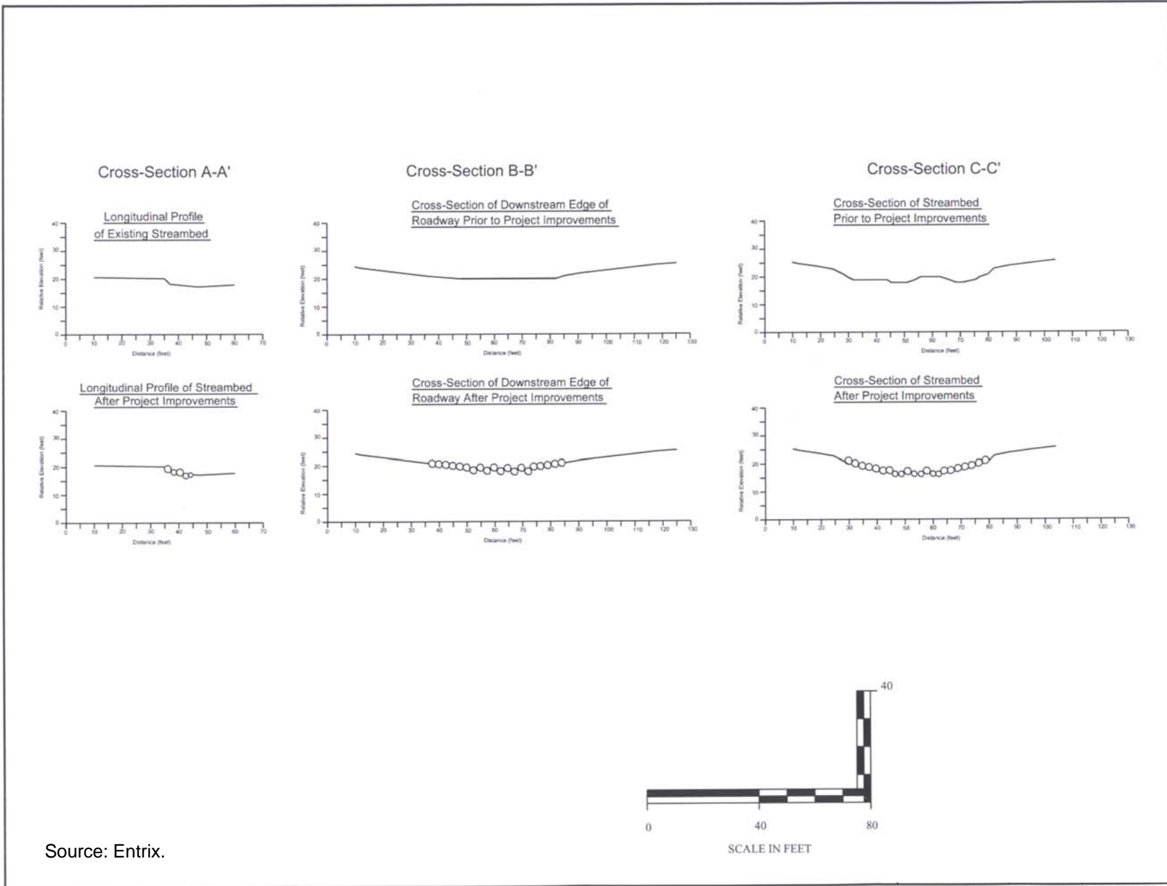
Figure 2-12. Cross Sections of Fishway at Quiota Creek Crossing No. 3
