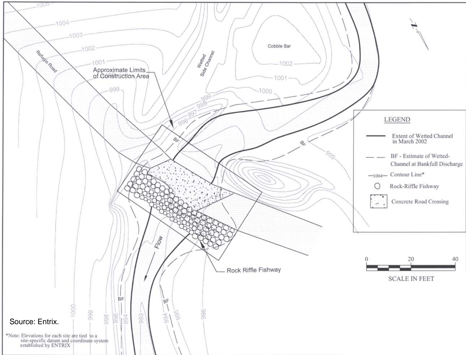
Figure 2-13. Proposed Fishway at Quiota Creek Crossing No. 4
