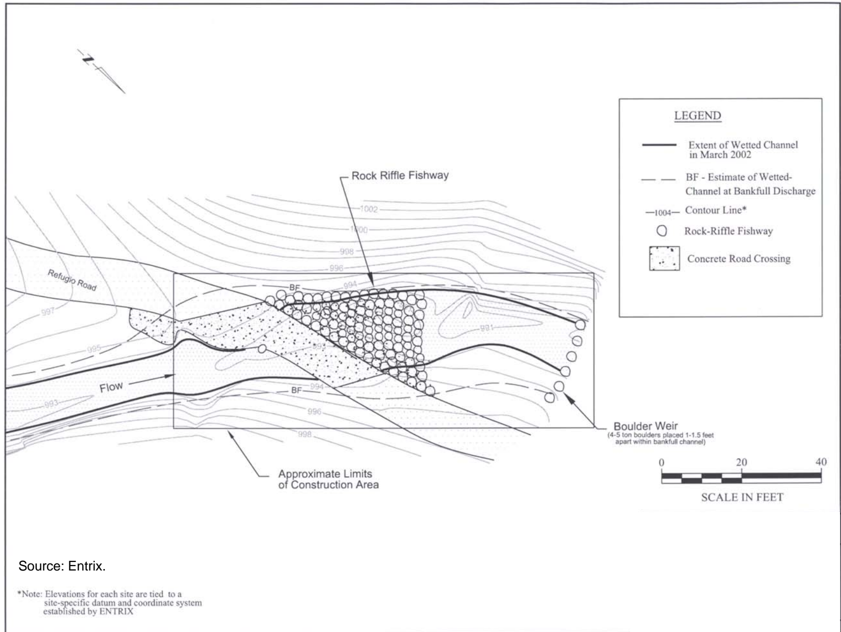
Figure 2-15. Proposed Fishway at Quiota Creek Crossing No. 7
