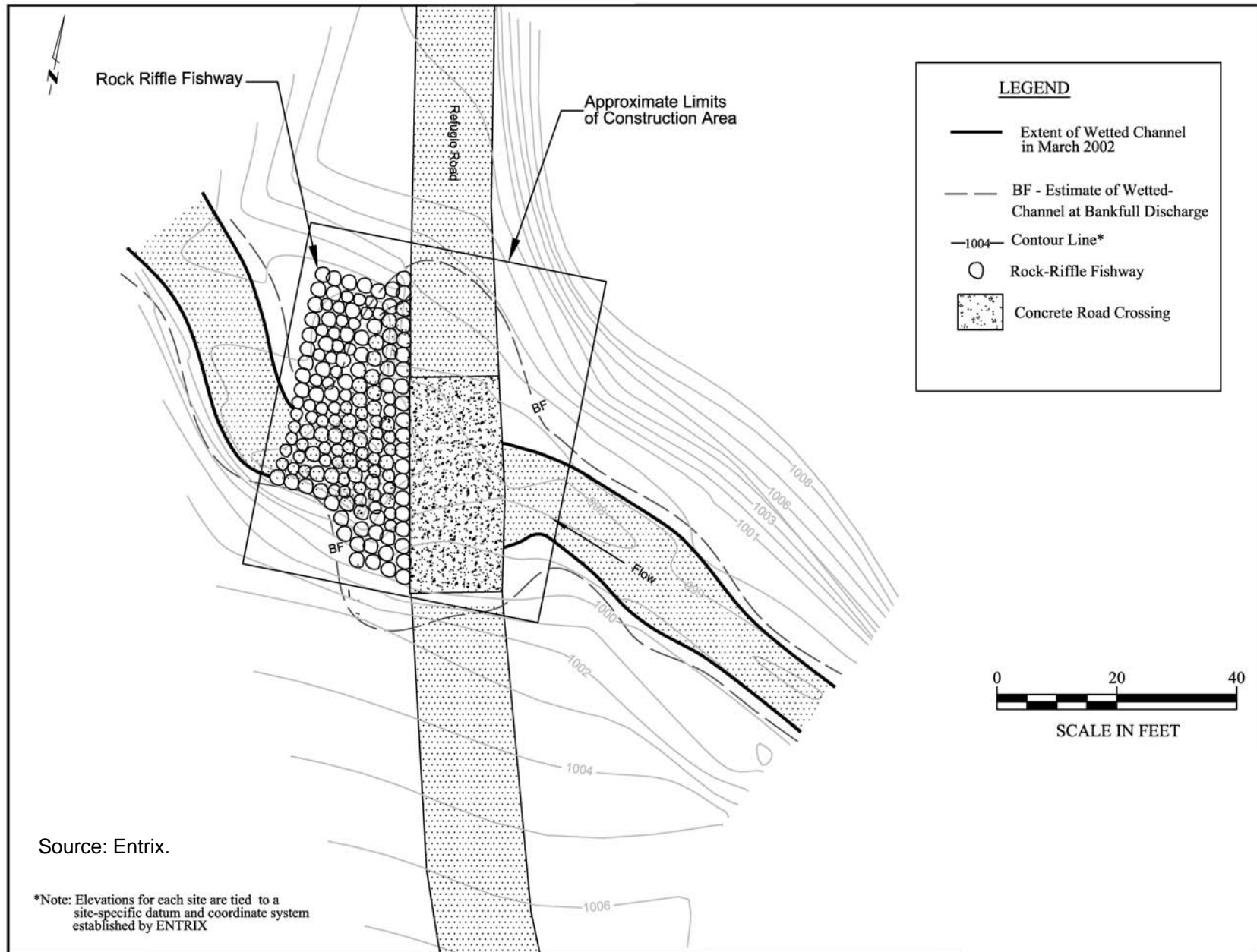
Figure 2-16. Proposed Fishway at Quiota Creek Crossing No. 9
