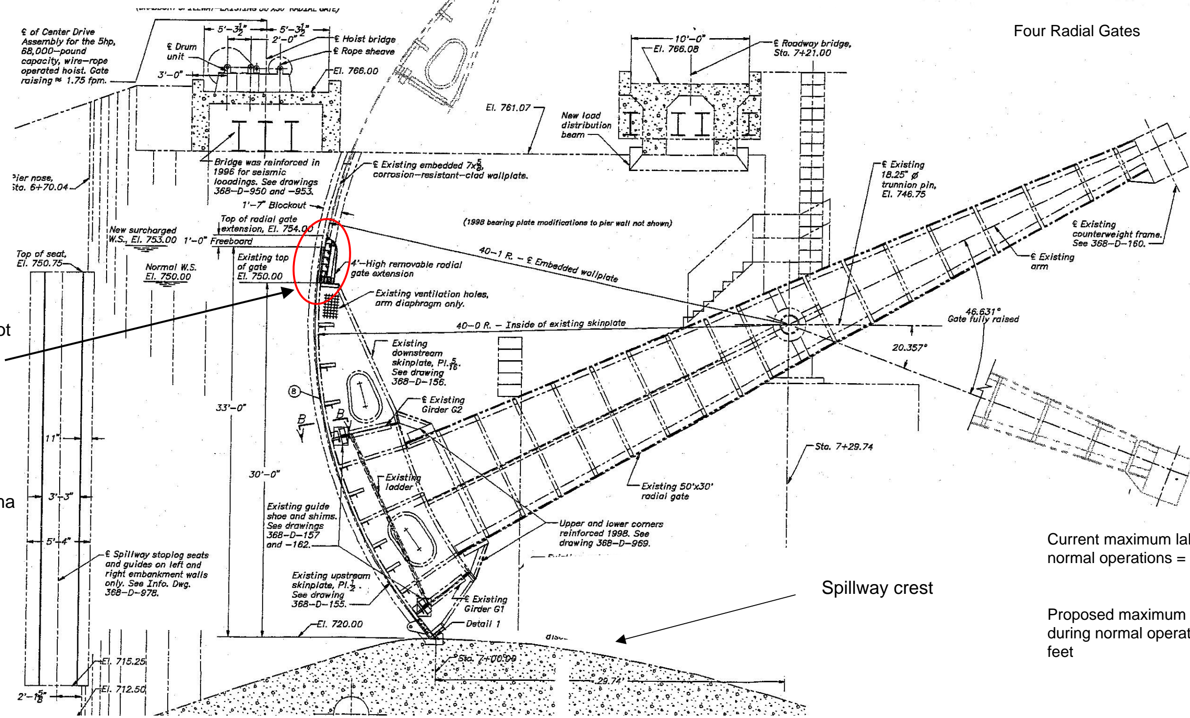
Figure 2-2. Proposed Flashboards for Surcharging
