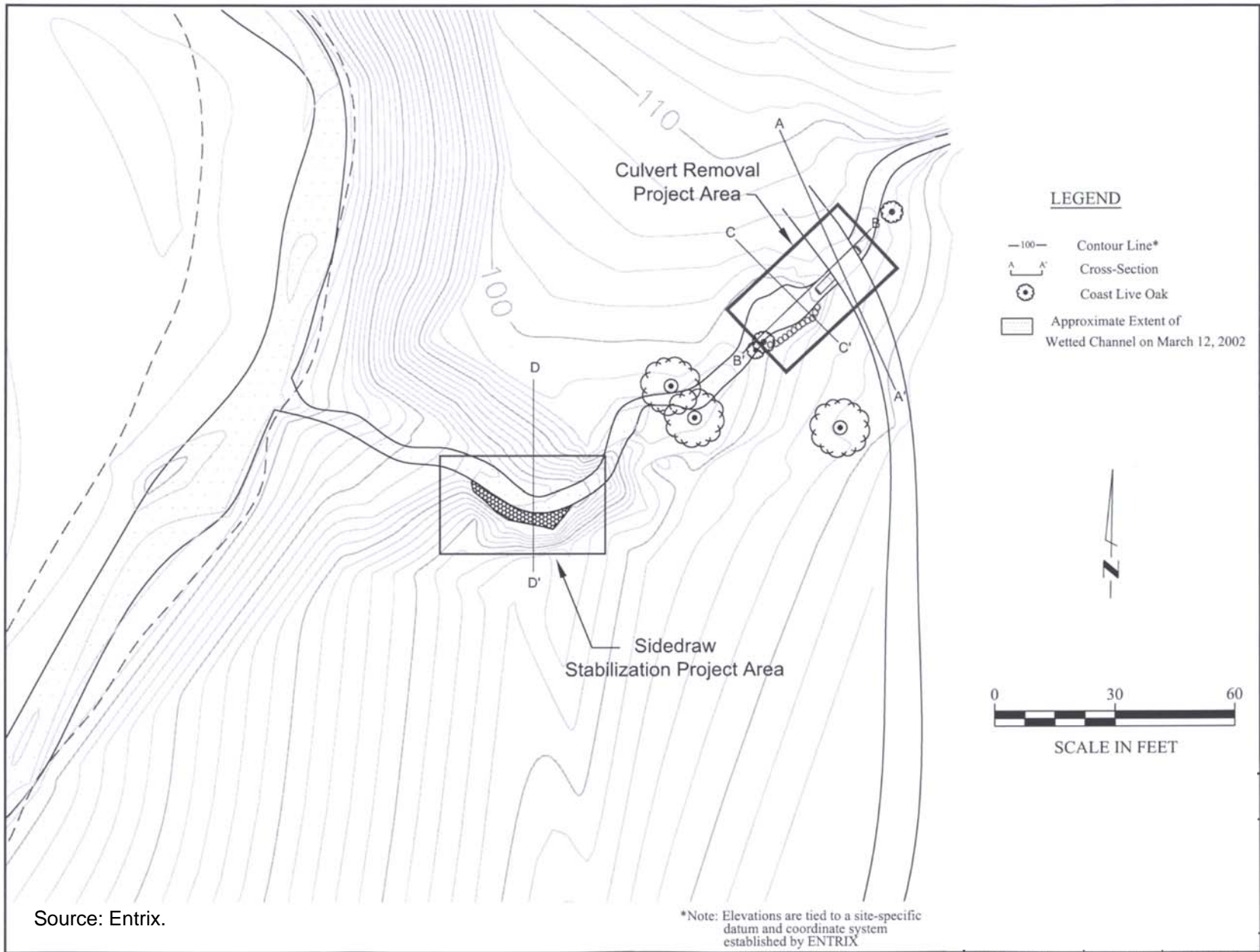
Figure 2-22. Culvert Removal and Sidedraw Stabilization Sites
