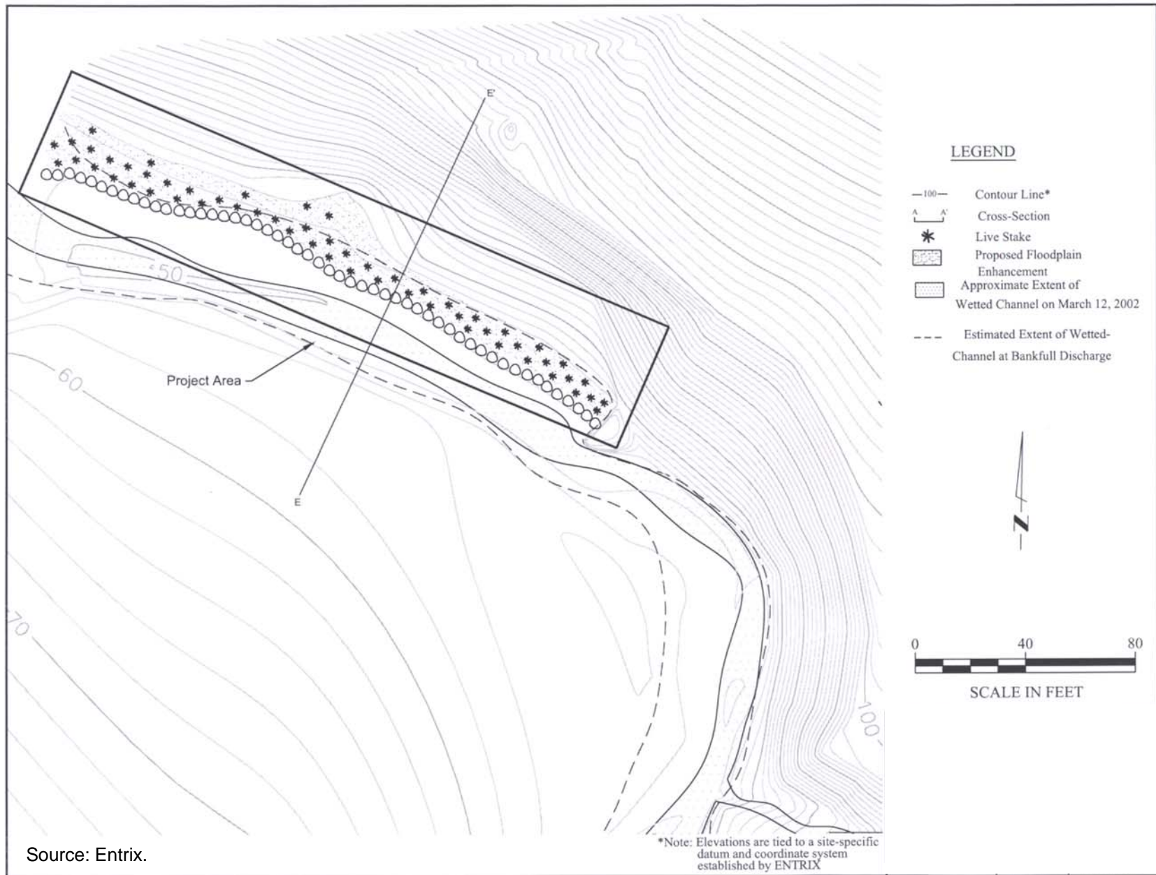
Figure 2-25. Bank Stabilization Project
