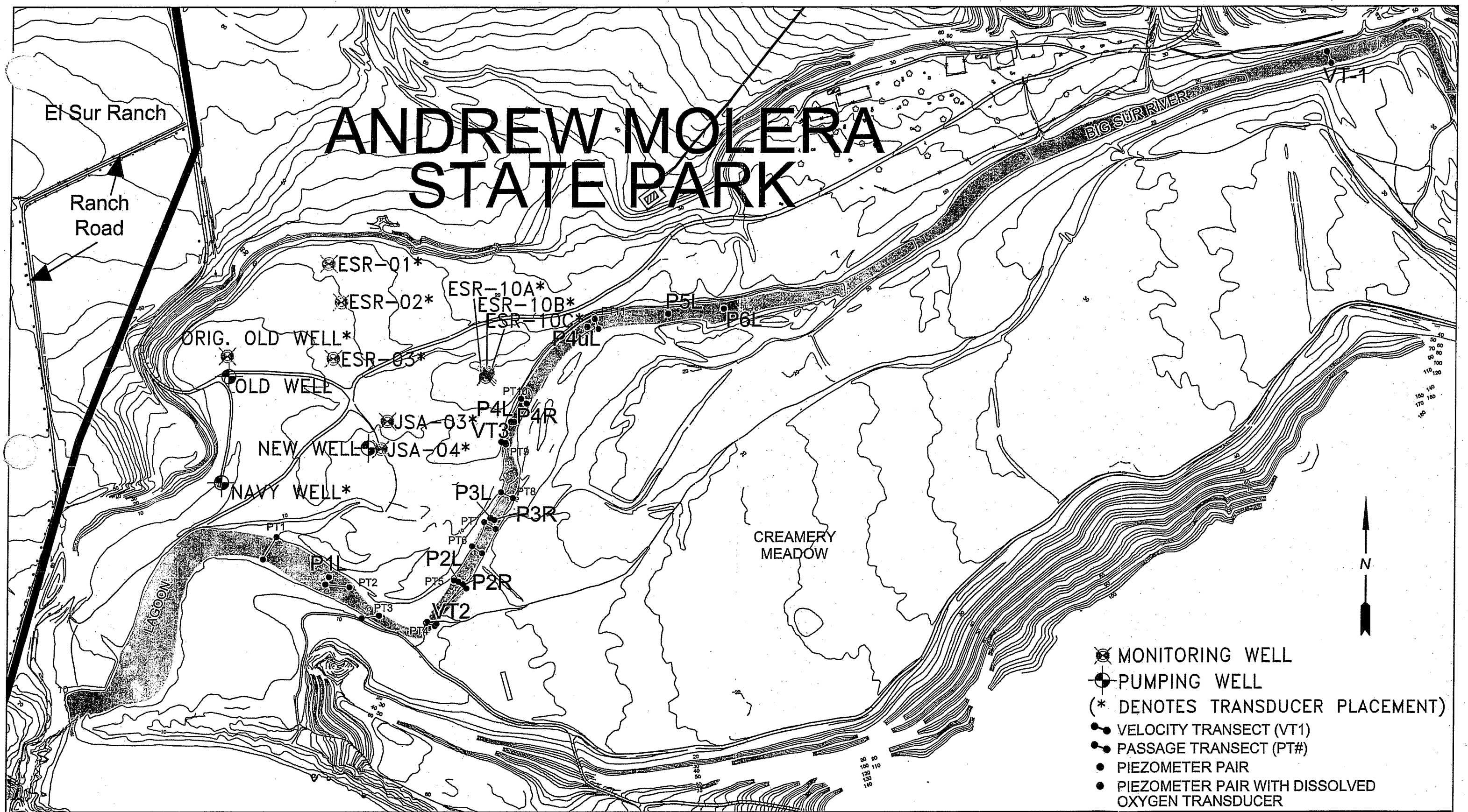
FIGURE 2-1 2007 STUDY AREA MONITORING STATION AND SENSOR LOCATION MAP
