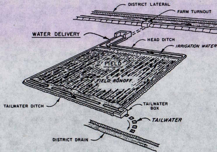
EXISTING IRRIGATION
