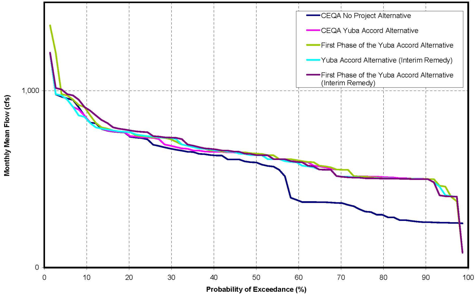
Lower Yuba River Flow at Marysville during September
