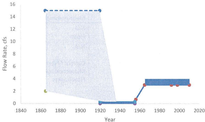
Figure 7. Water Use for Mining and Hydropower Generation
