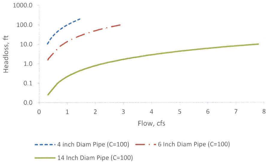
Figure 4. Pipe Headlosses
