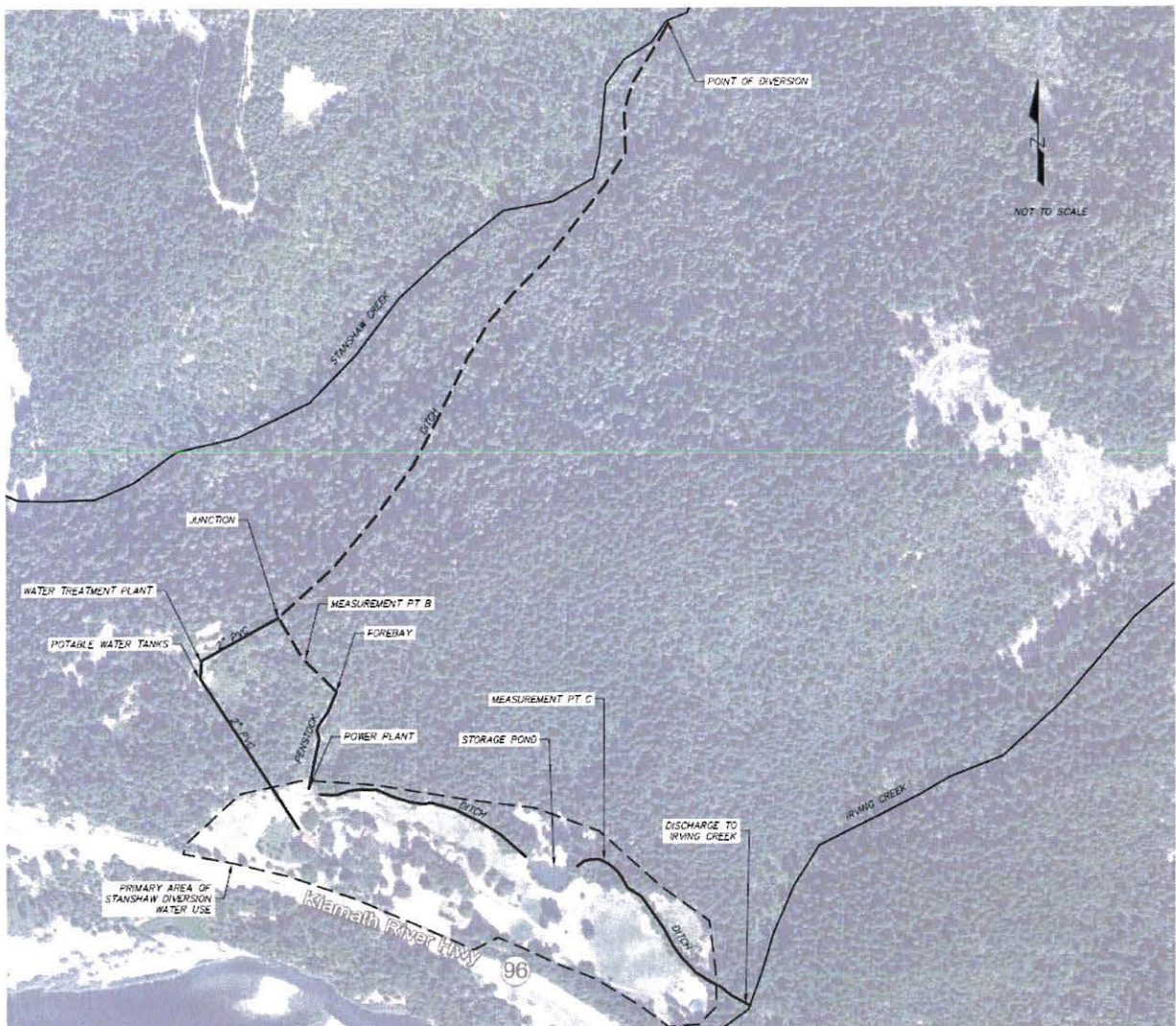
Figure 2. Water Conveyance Map
