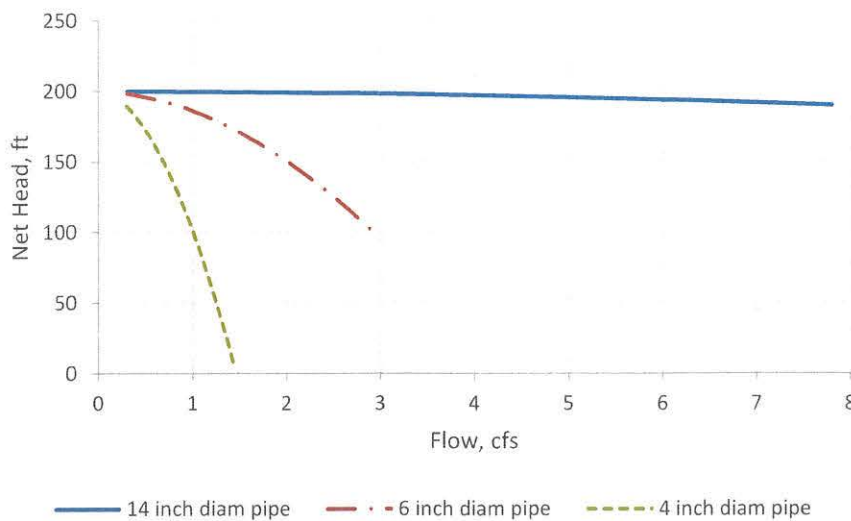
Figure 5. Net Head Change with Flow
