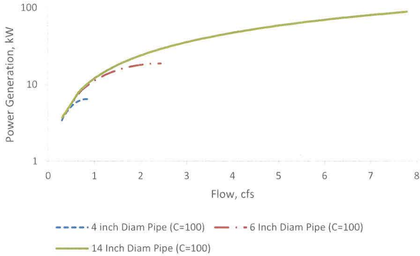
Figure 6. Power Generation Rating Curves
