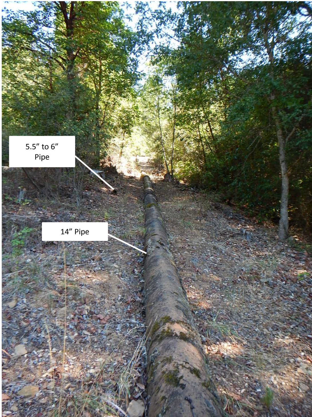
Photograph 2. 14" Diameter Penstock installed by Lue Hayes after he purchased the property in 1955.
