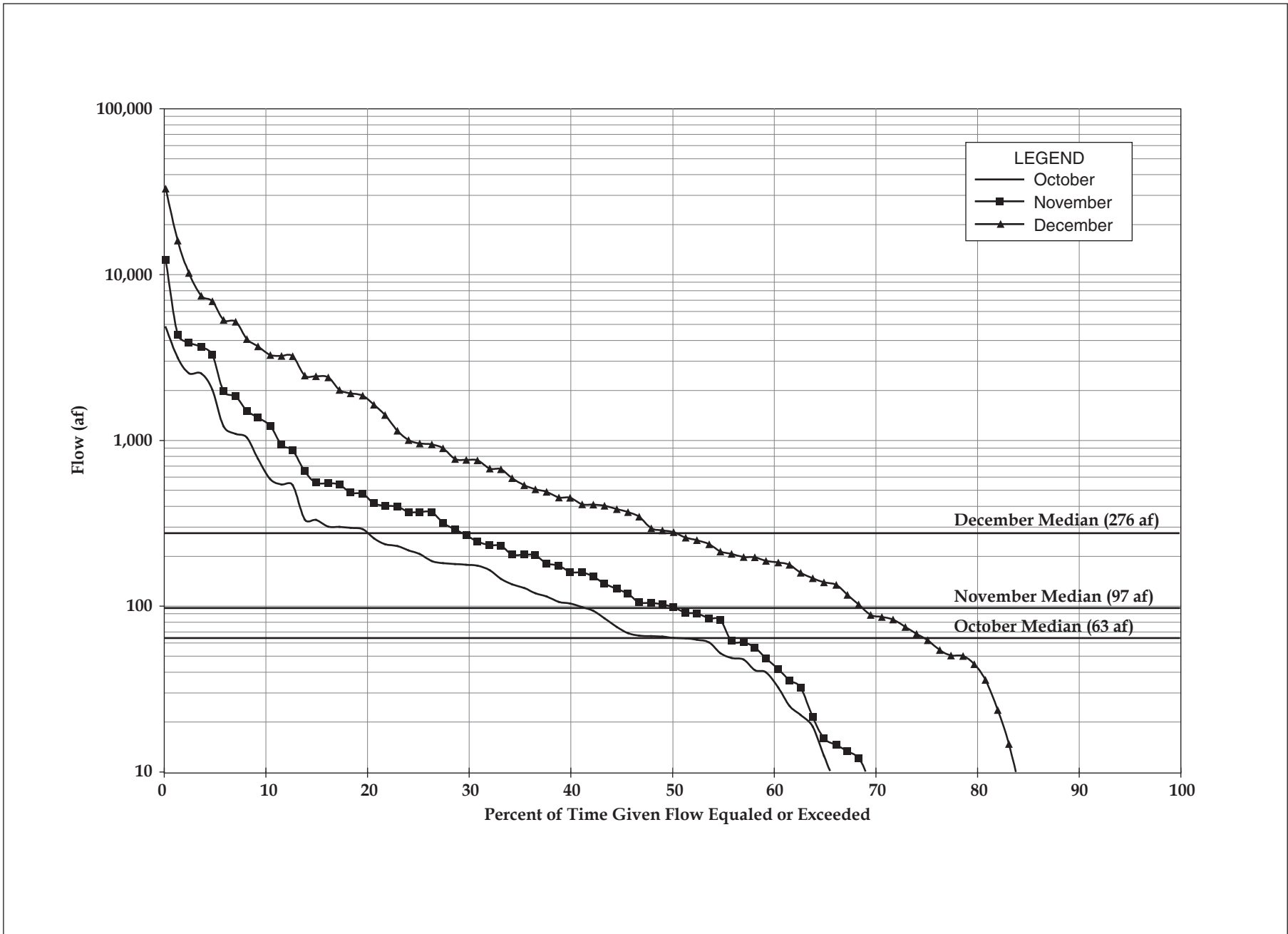
Figure 2.2-5. Probability of Monthly Flow at River Only Mentone Gage, Months of October, November, and December (WY 1911-12 to WY 1999-2000)
