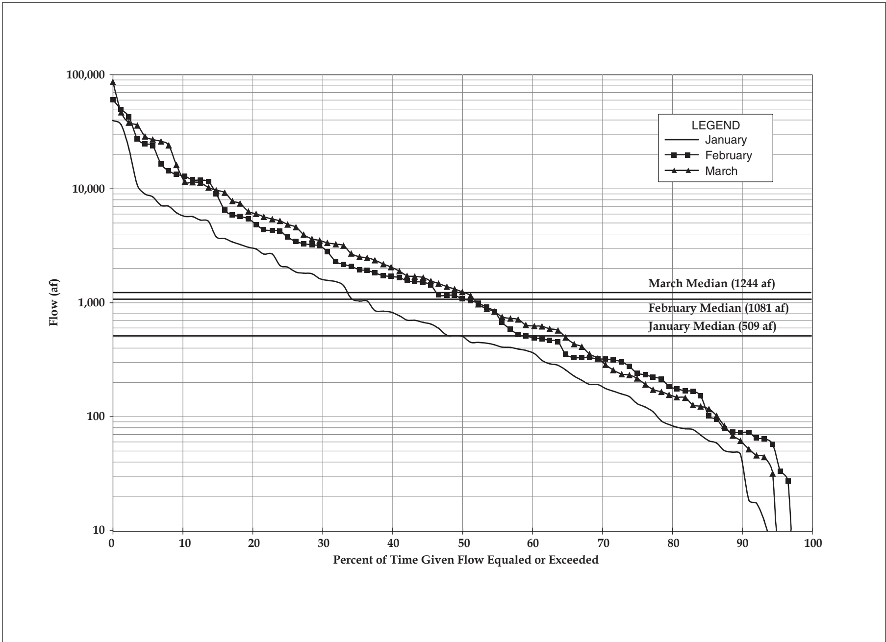
Figure 2.2-6. Probability of Monthly Flow at River Only Mentone Gage, Months of January, February, and March (WY 1911-12 to WY 1999-2000)
