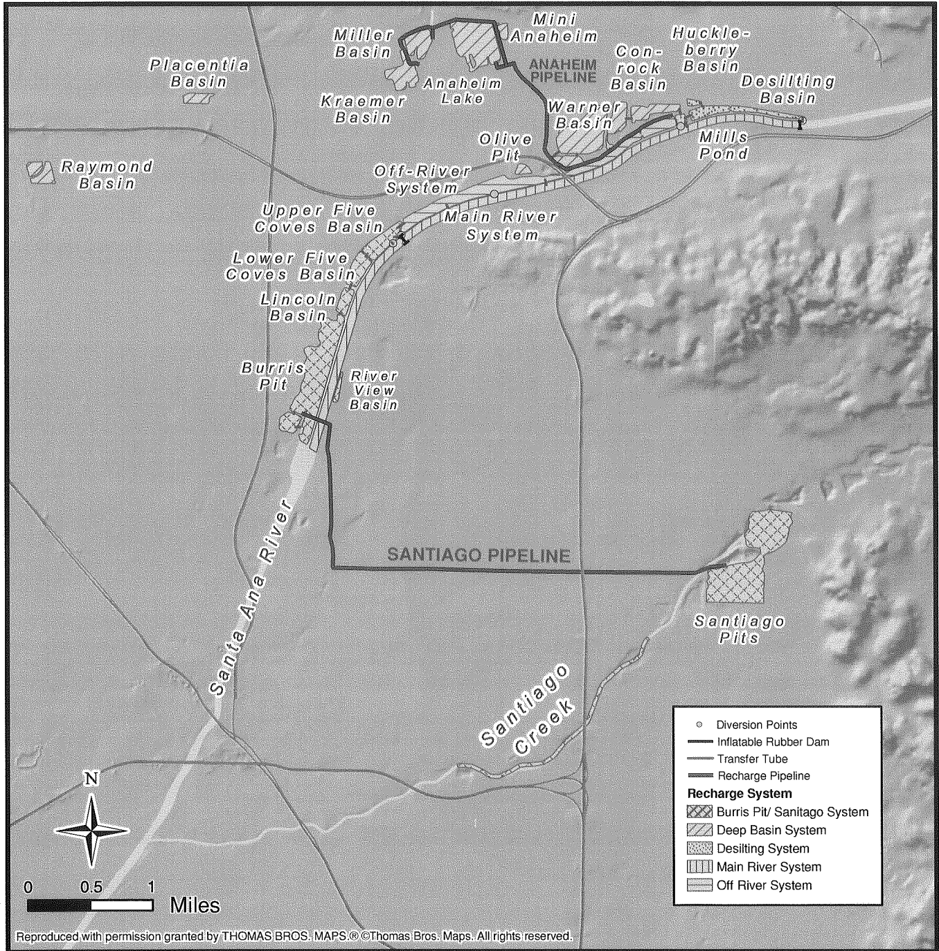
Figure 2-4. OCWD recharge facilities.
