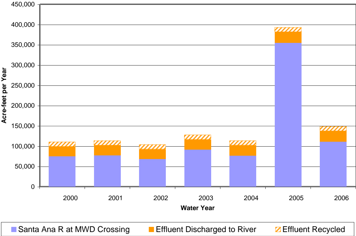
Illustration of Reduced Effluent Discharge Associated with 11,000 AF/yr Recycling Over Recent Six-Year Period
