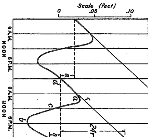
FIGURE 4.-- Representative ground-water curve, showing effect of the daily cycle of transpiration by overlying vegetation (after Troxell).
