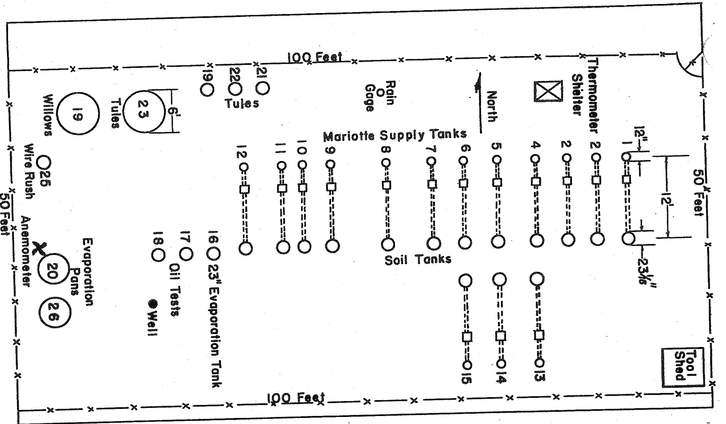
FIGURE 5.-- Plan of evaporation station near Santa Ana, Calif.
