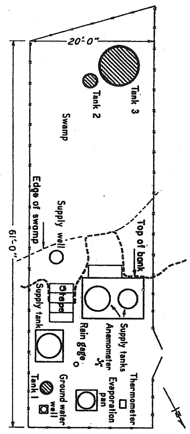
FIGURE 7.-- Plan of Victorville station.
