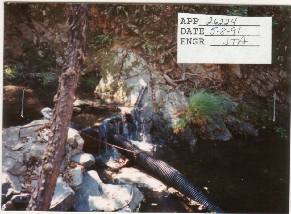
Diversion To Offstream Storage Structure In Oak Flat Creek - 0.7cfs flowing over
