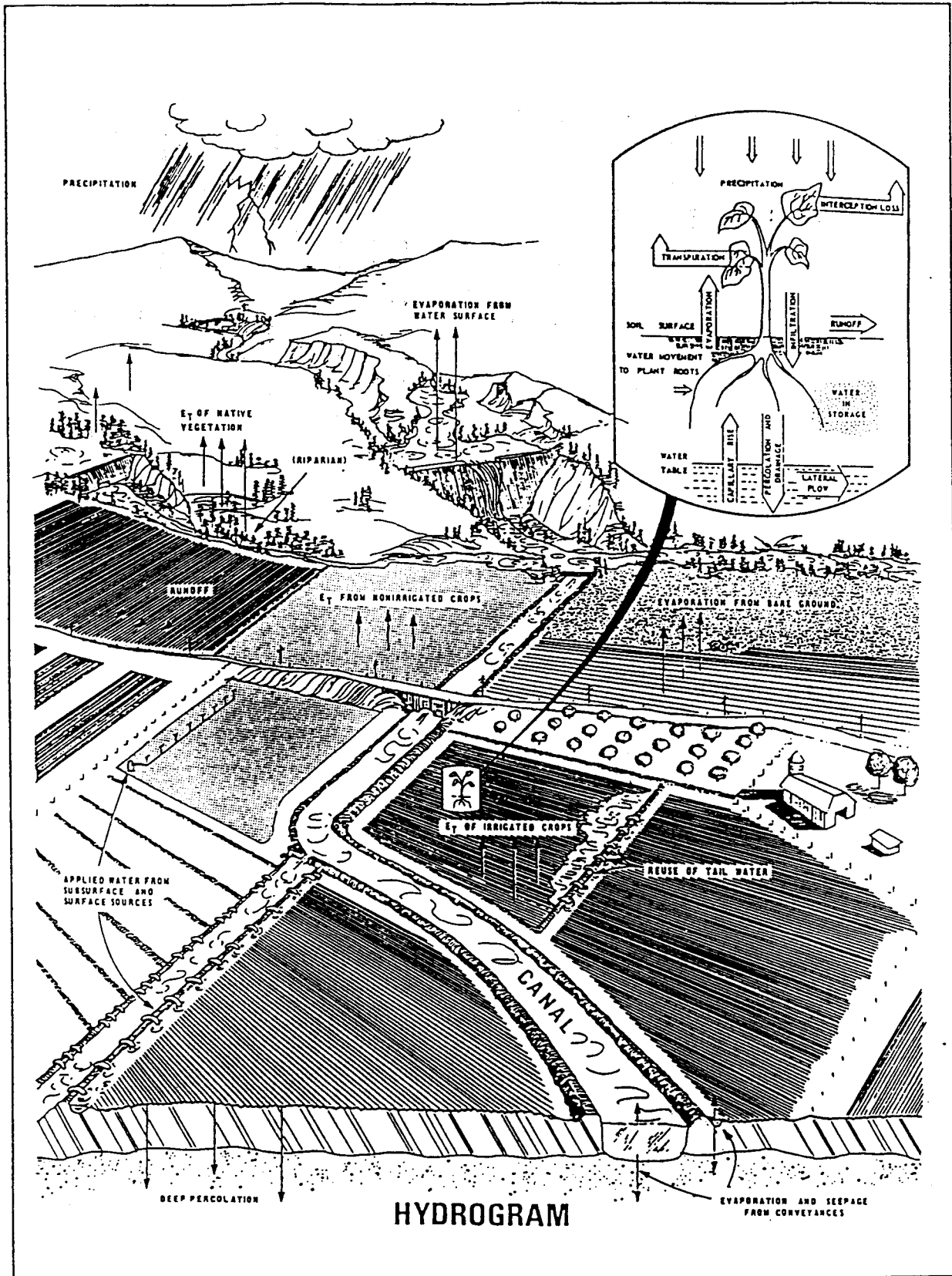
Figure 2-1. Hydrologic Cycle
