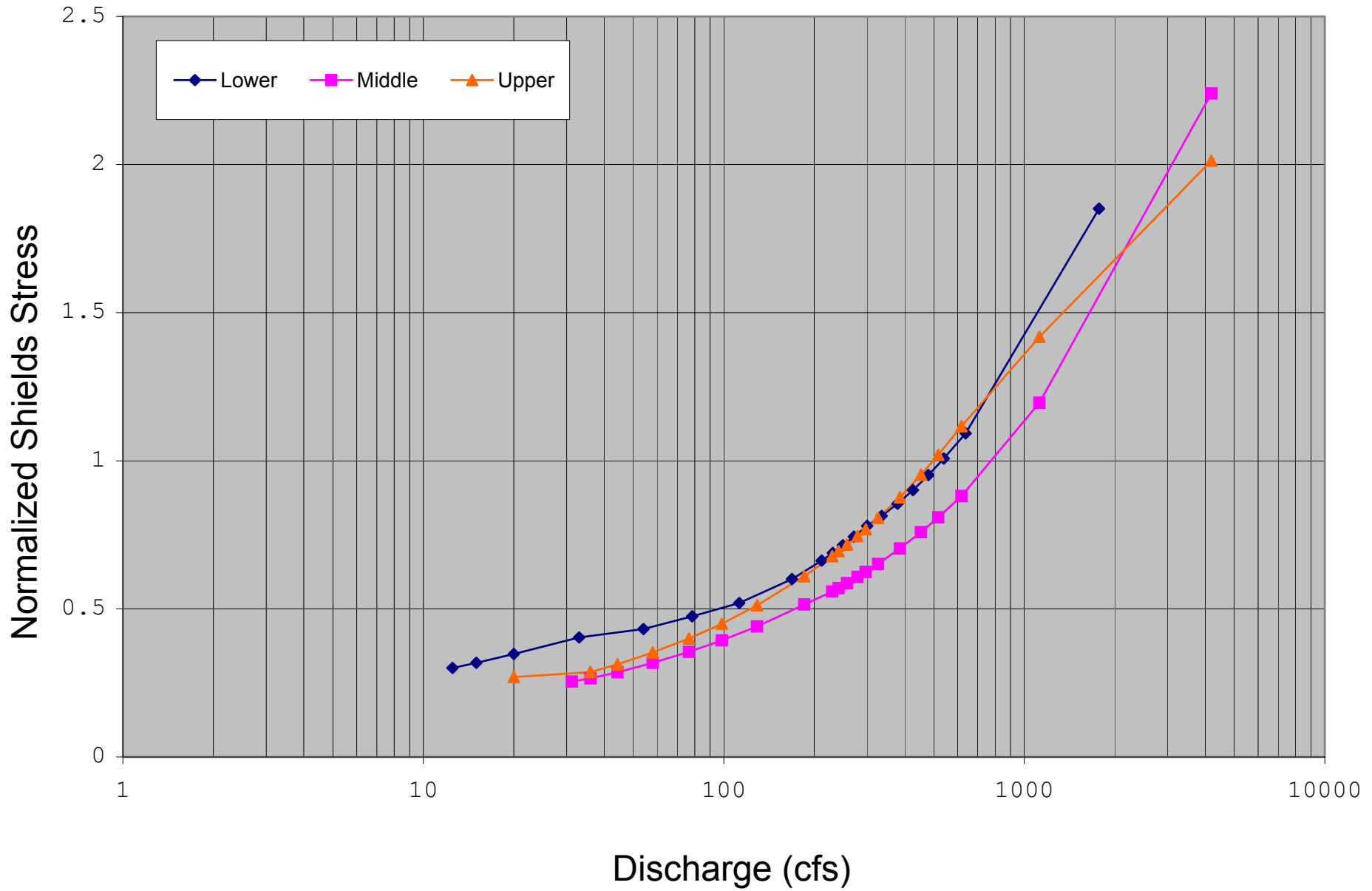
Figure N-12: Estimated Shields stress rating curve for the Ice House Dam Reach Lower Site.
