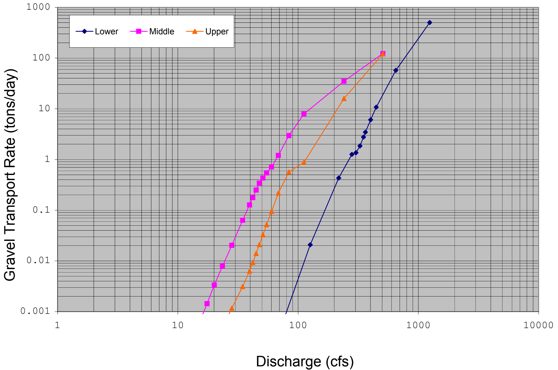
Figure N-3: Estimated bedload transport rating curve for the Loon Lake Dam Reach Middle Site.
