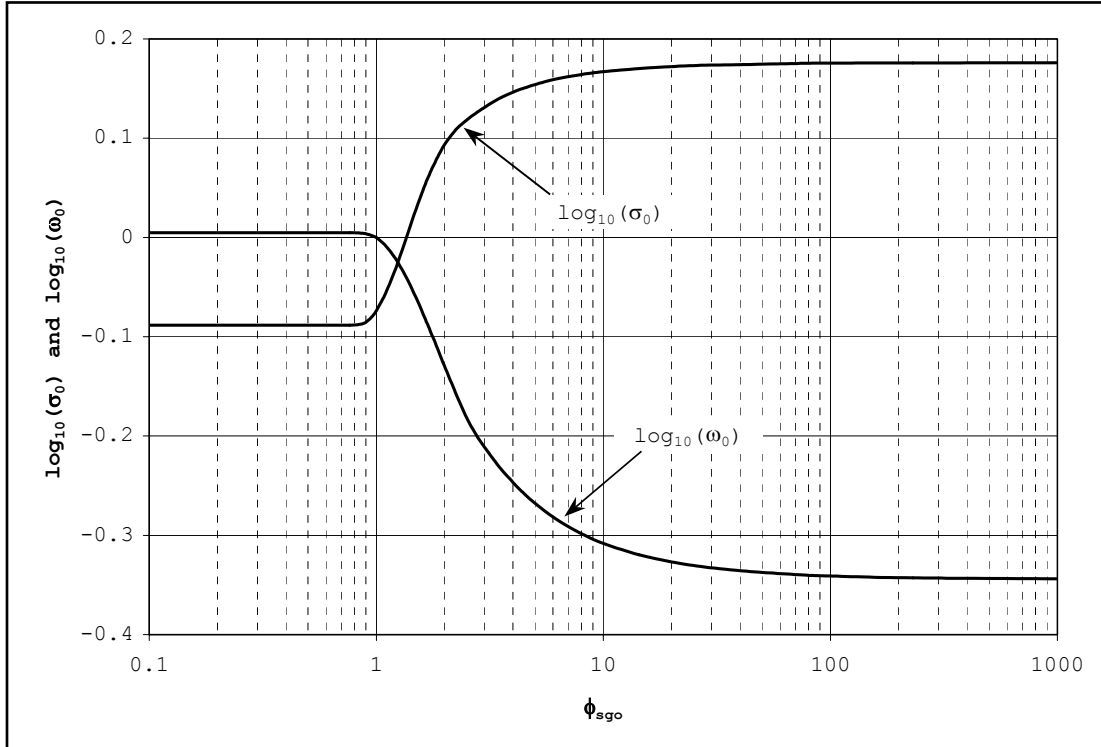
Figure M-1. Parameters \sigma_0 and \omega_0 as functions of \phi_{sgo} in Parker equation
