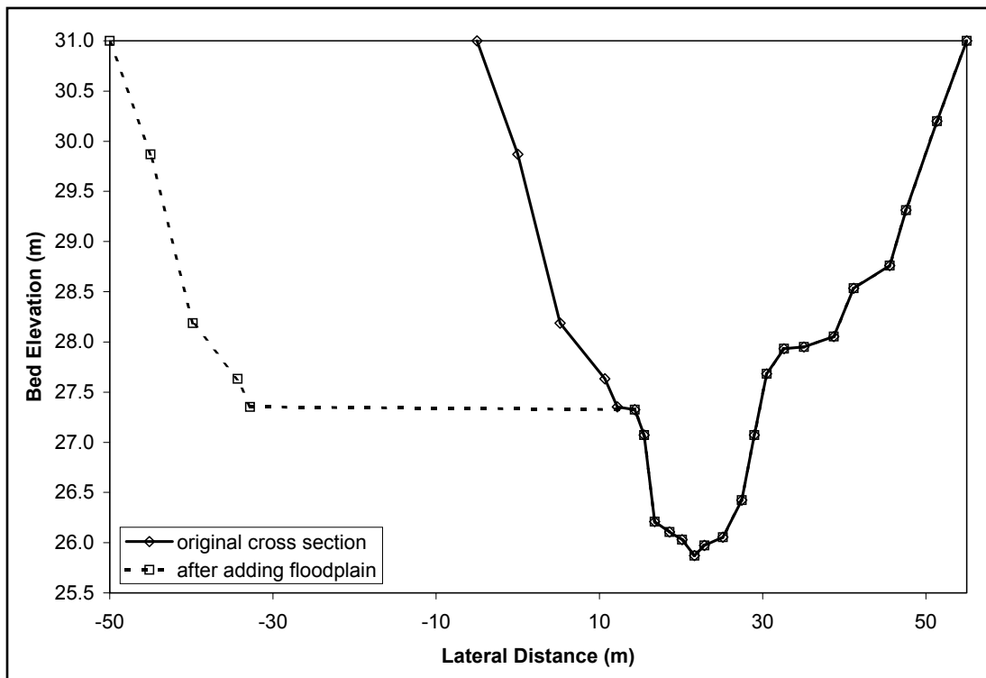
Figure M-3. Channel cross sections to be used in the example
