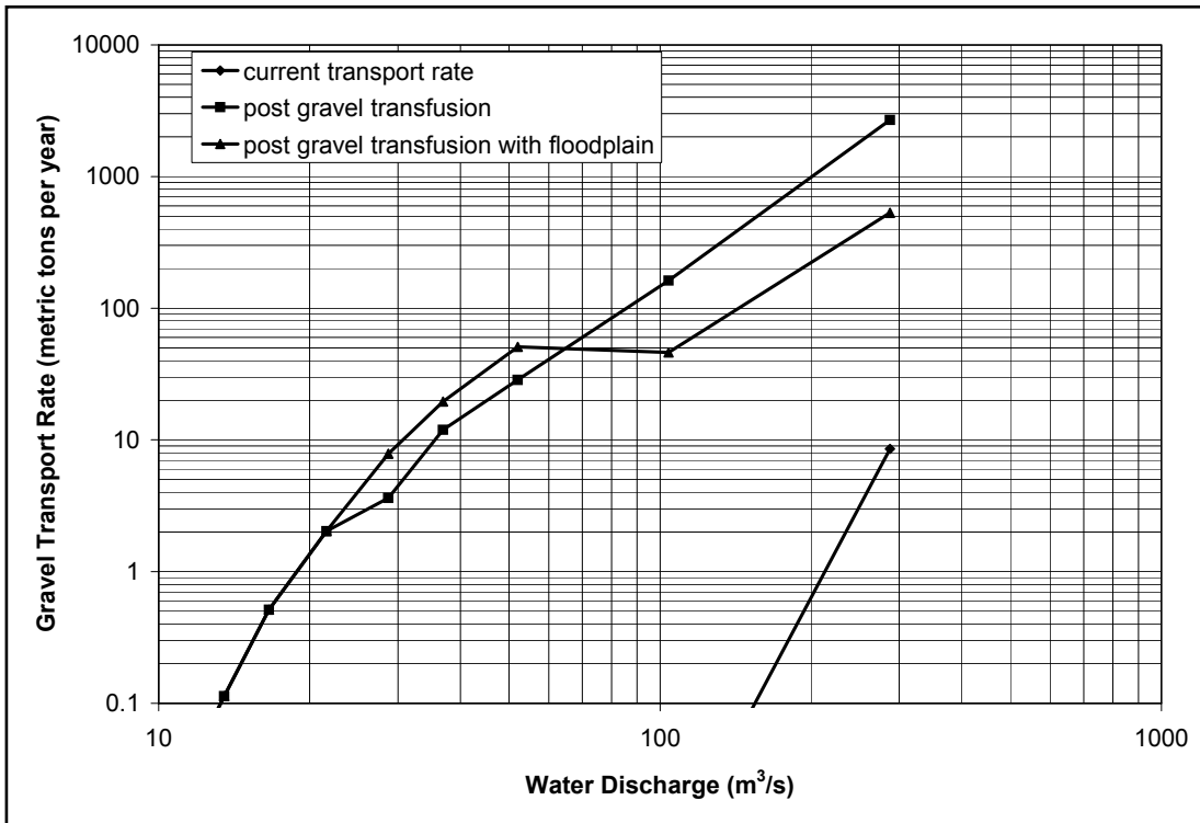
Figure M-6. Predicted gravel transport rate presented in the example.
