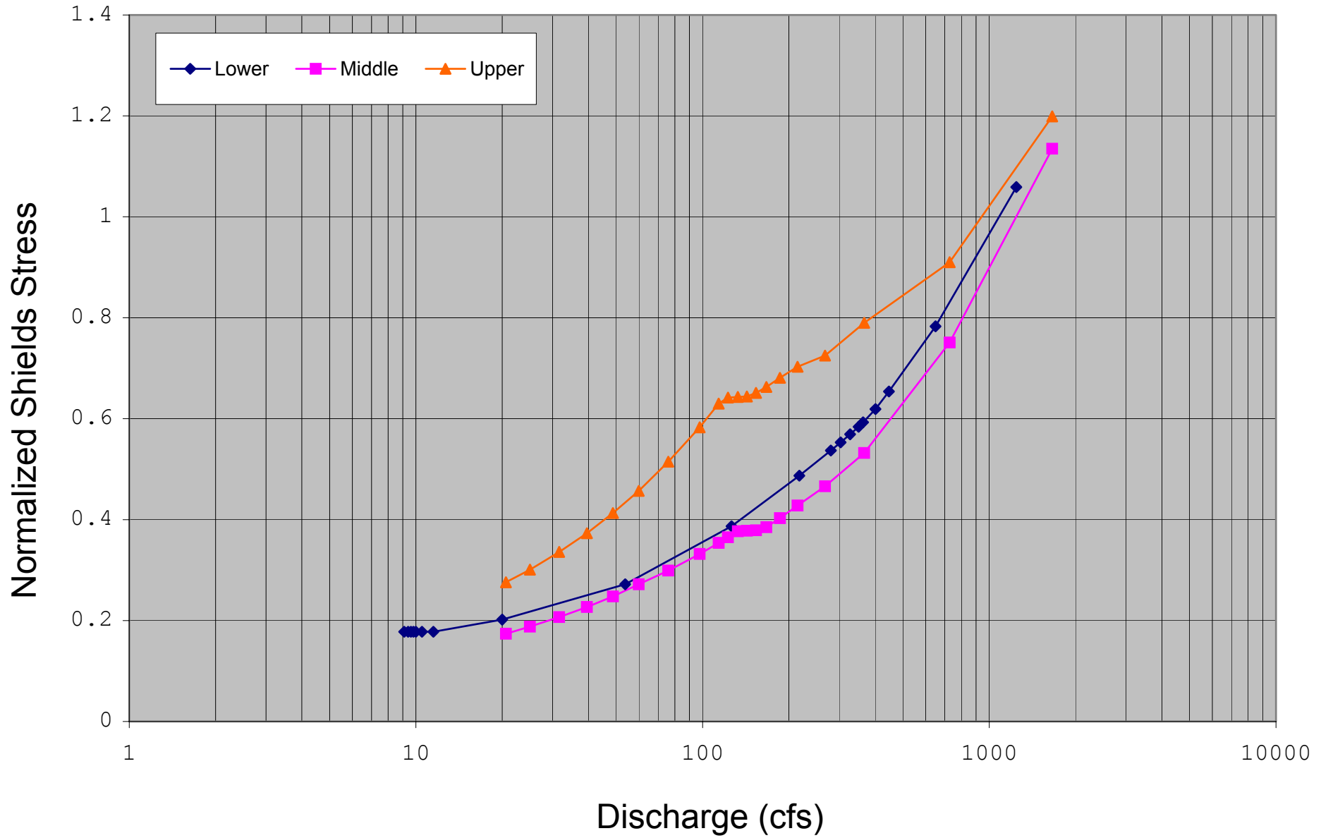
Figure N-6: Estimated Shields stress rating curve for the Loon Lake Dam Reach Lower Site.
