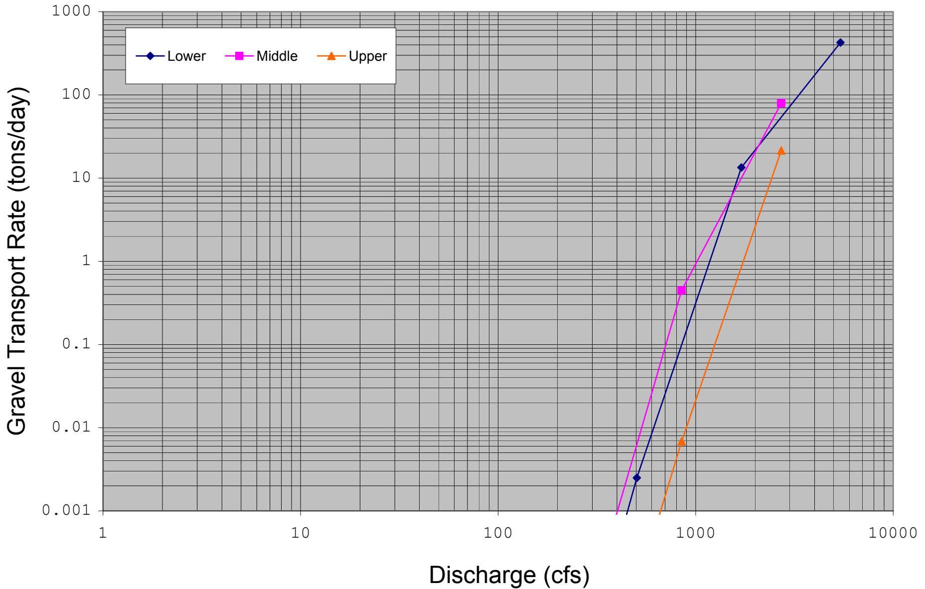
Figure N-7: Estimated bedload transport rating curve for the Robbs Peak Dam Reach Site.
