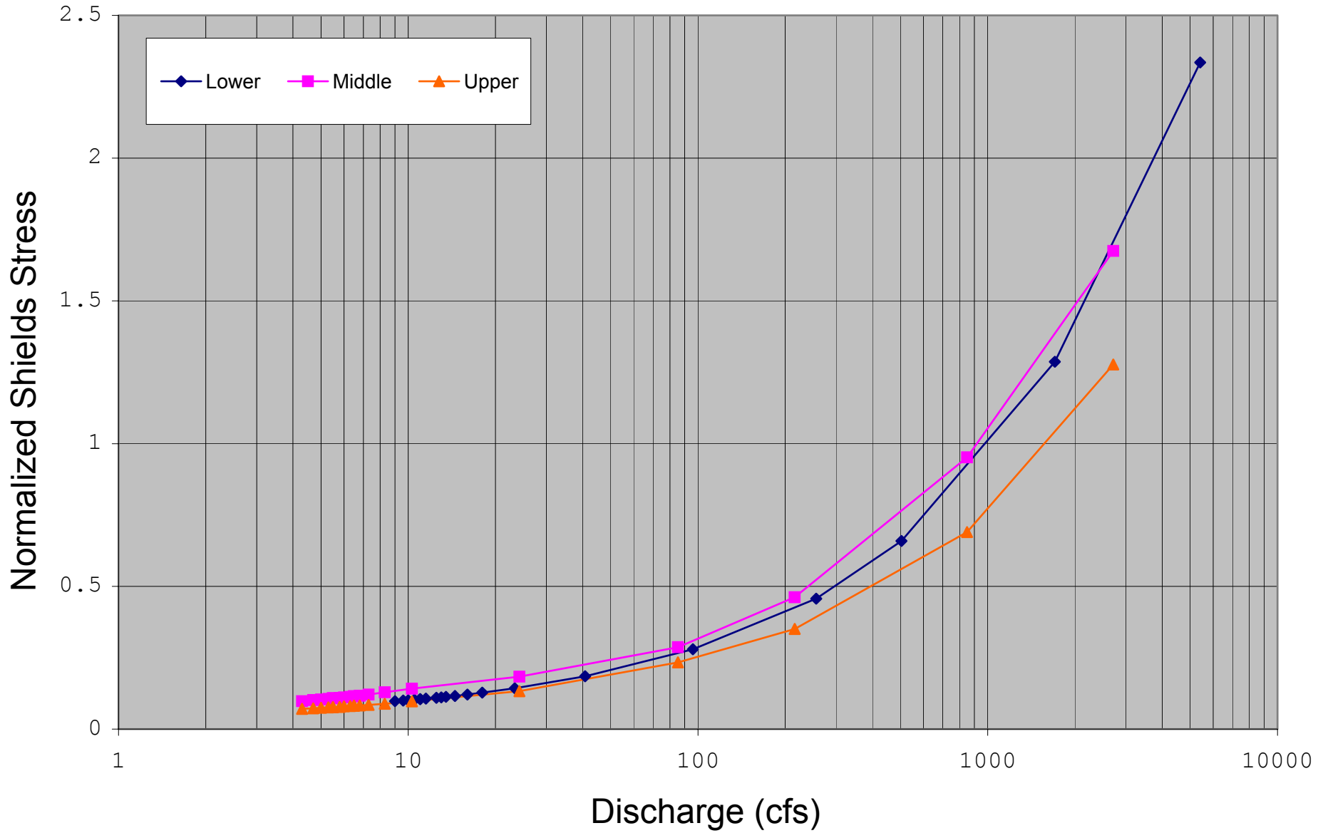
Figure N-8: Estimated Shields stress rating curve for the Robbs Peak Dam Reach Site.
