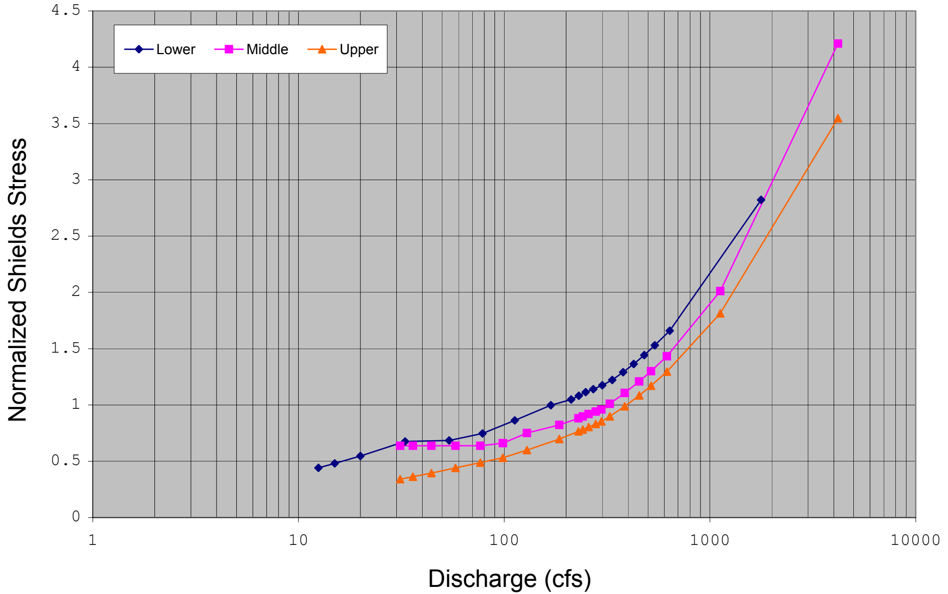
Figure N-10: Estimated Shields stress rating curve for the Ice House Dam Reach Upper Site.
