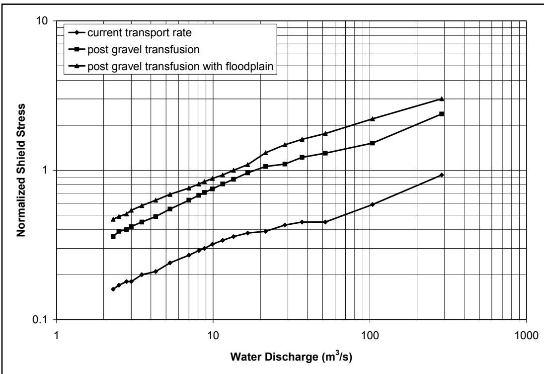
Figure M-7. Predicted normalized Shields stress as presented in the example.
