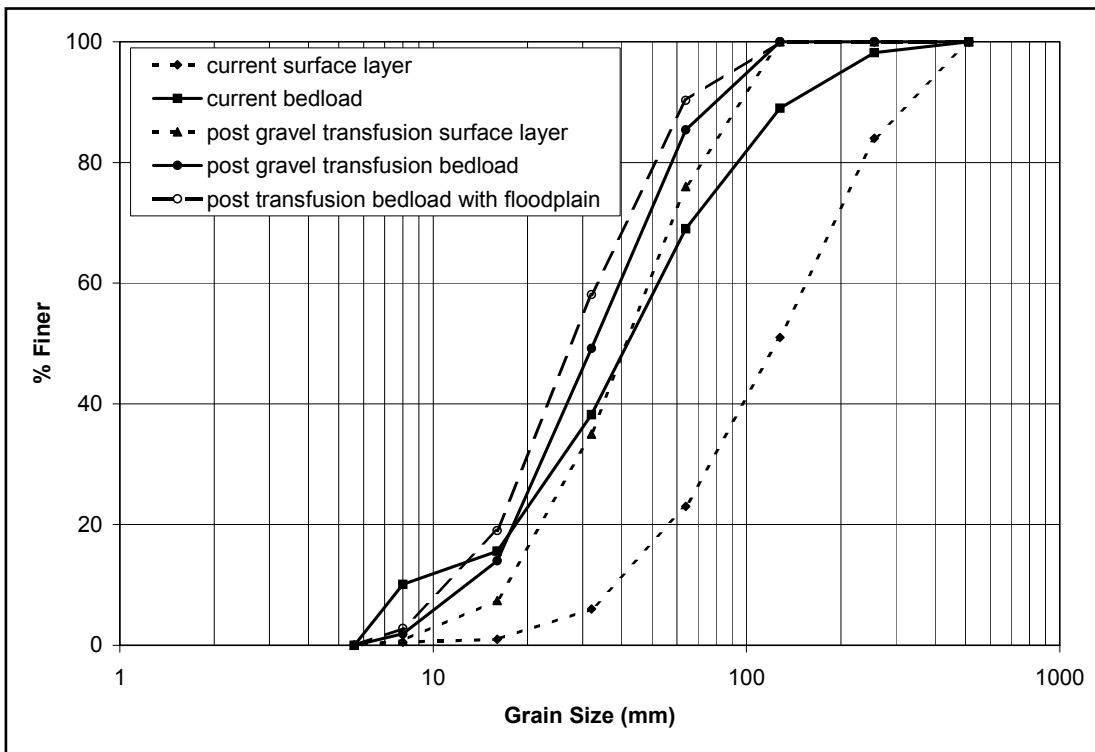
Figure M-5. Grain size distributions presented in the example.
