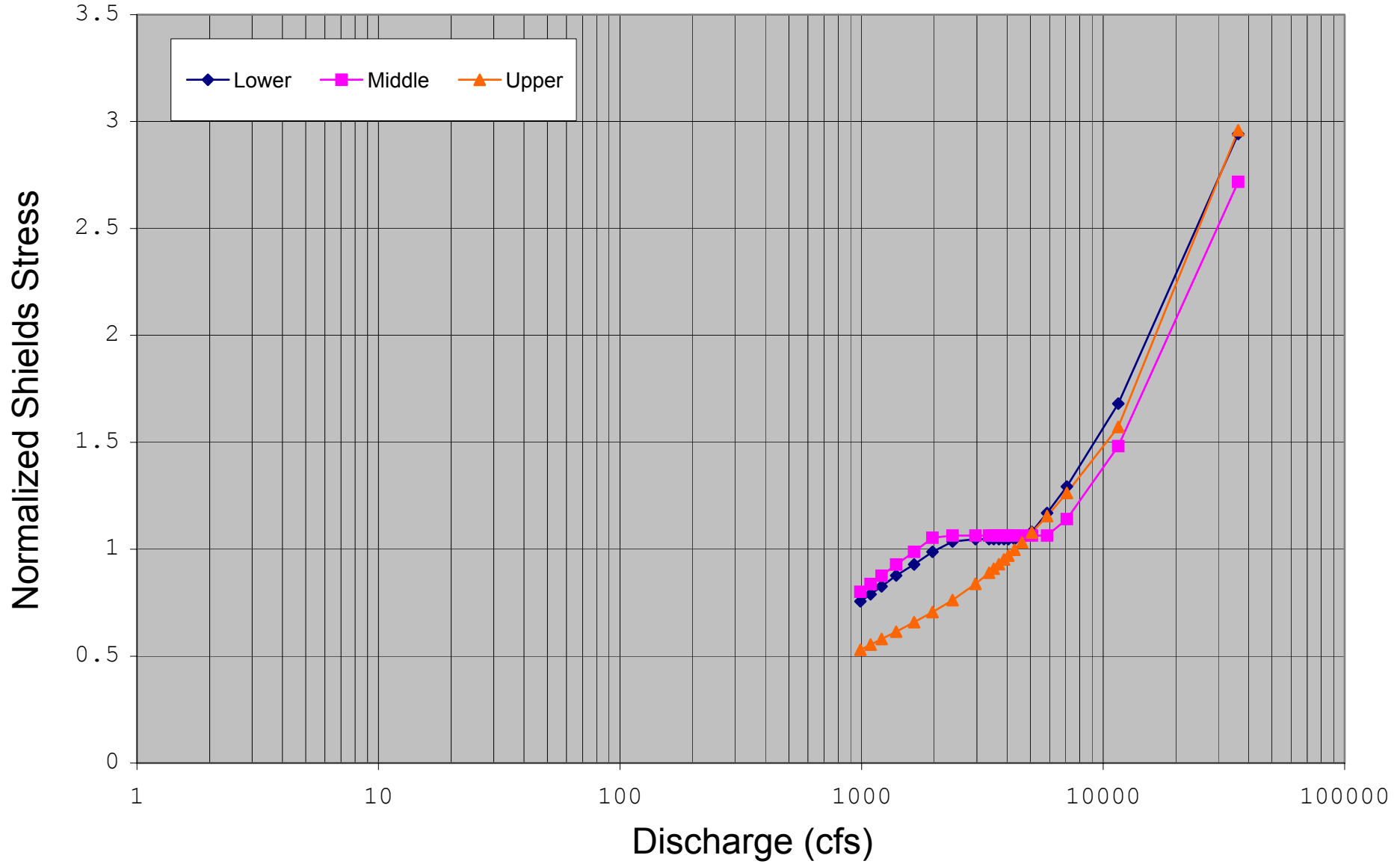
Figure N-14: Estimated Shields stress rating curve for the Reach Downstream of Chili Bar, Upper Coloma Study Site.
