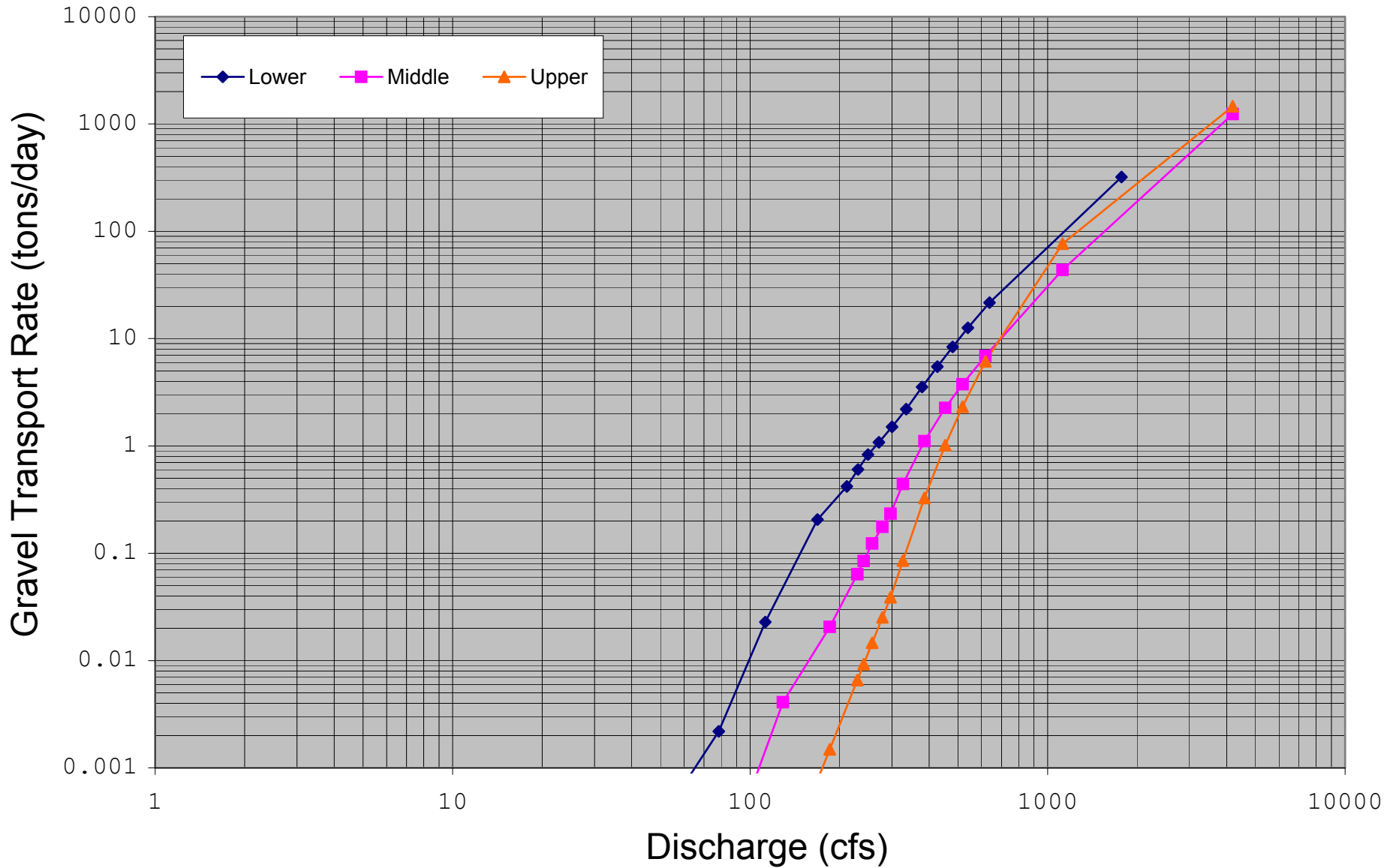
Figure N-9: Estimated bedload transport rating curve for the Ice House Dam Reach Upper Site.
