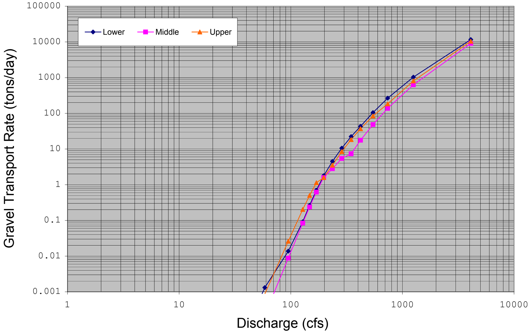
Figure N-1: Estimated bedload transport rating curve for the Rubicon Dam Reach Site.
