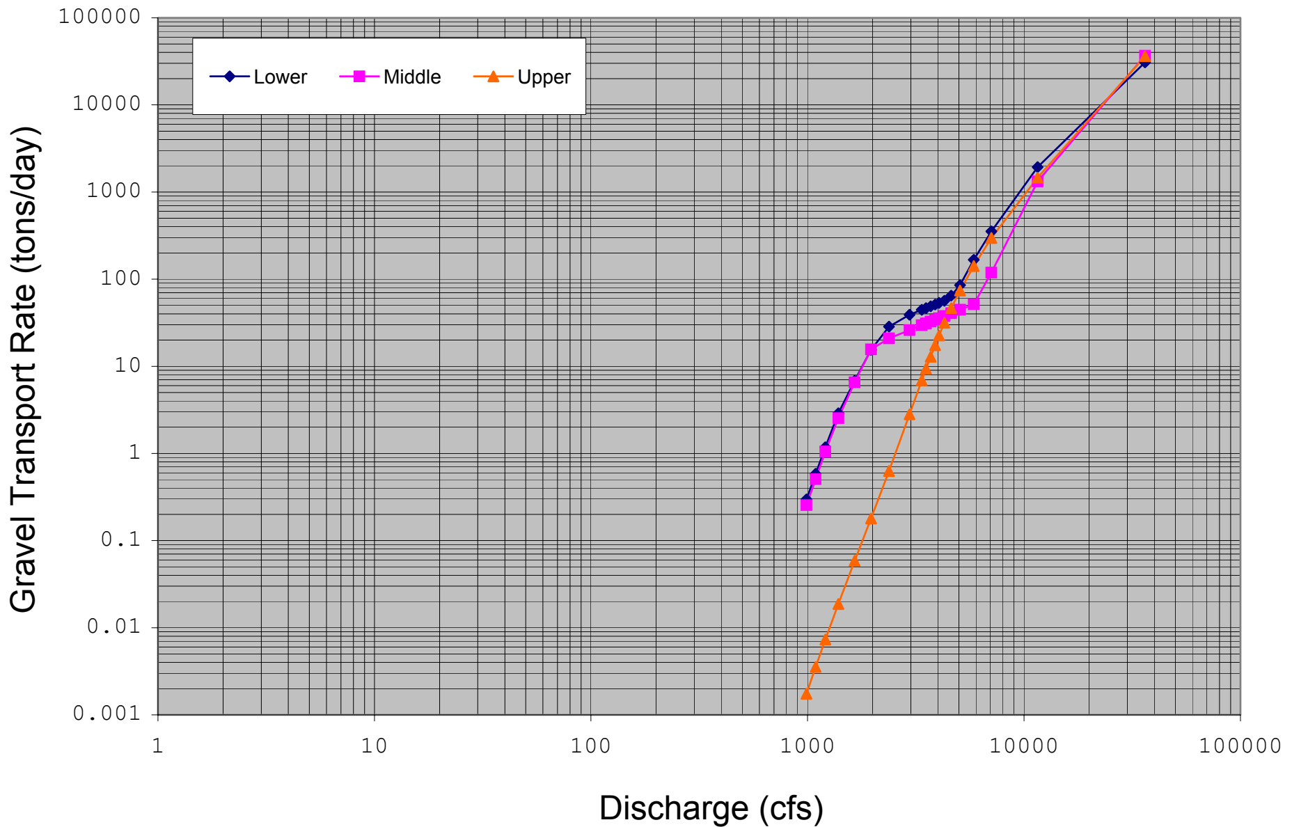
Figure N-13: Estimated bedload transport rating curve for the Reach Downstream of Chili Bar, Upper Coloma Study Site.
