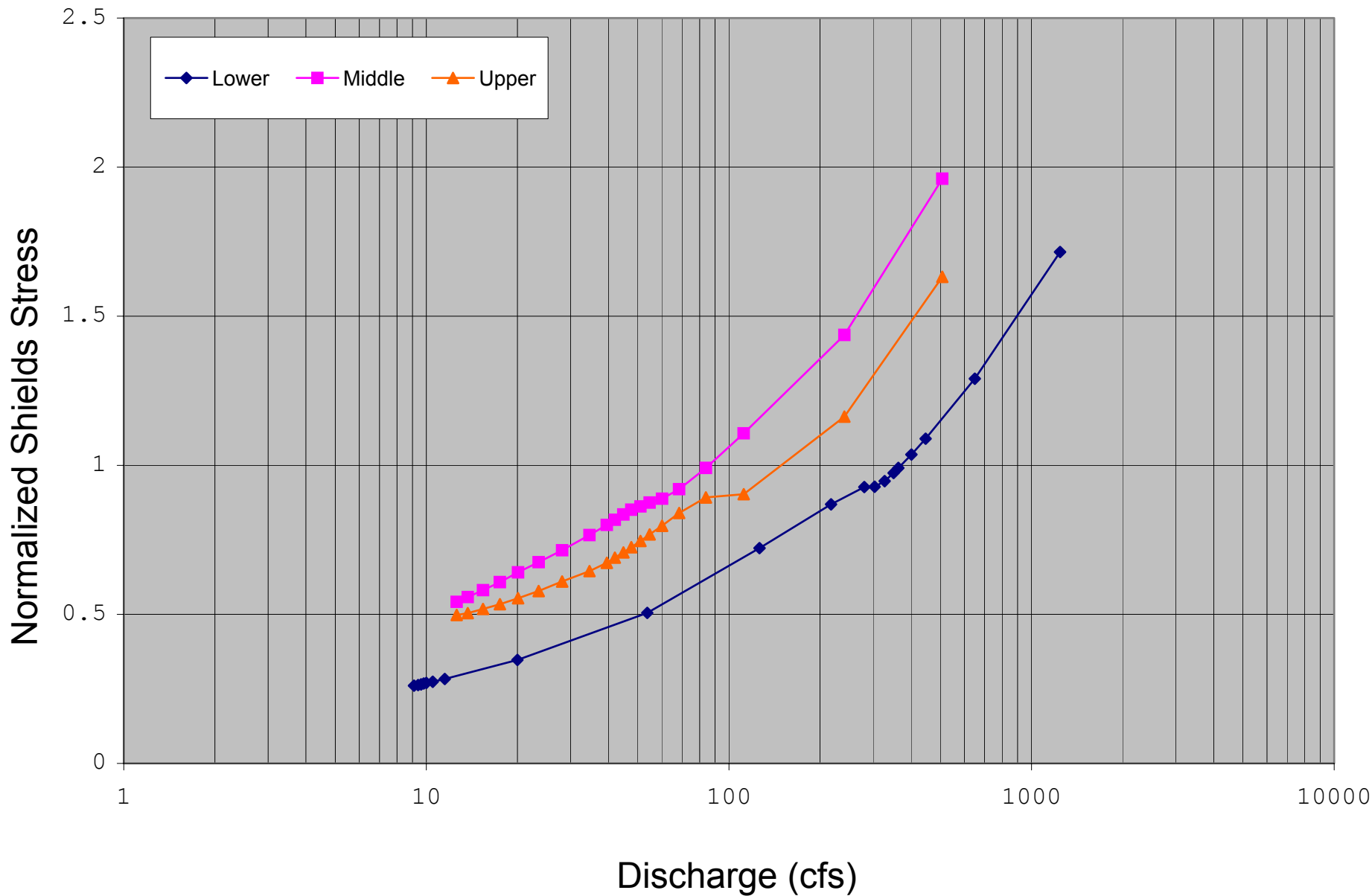
Figure N-4: Estimated Shields stress rating curve for the Loon Lake Dam Reach Middle Site.
