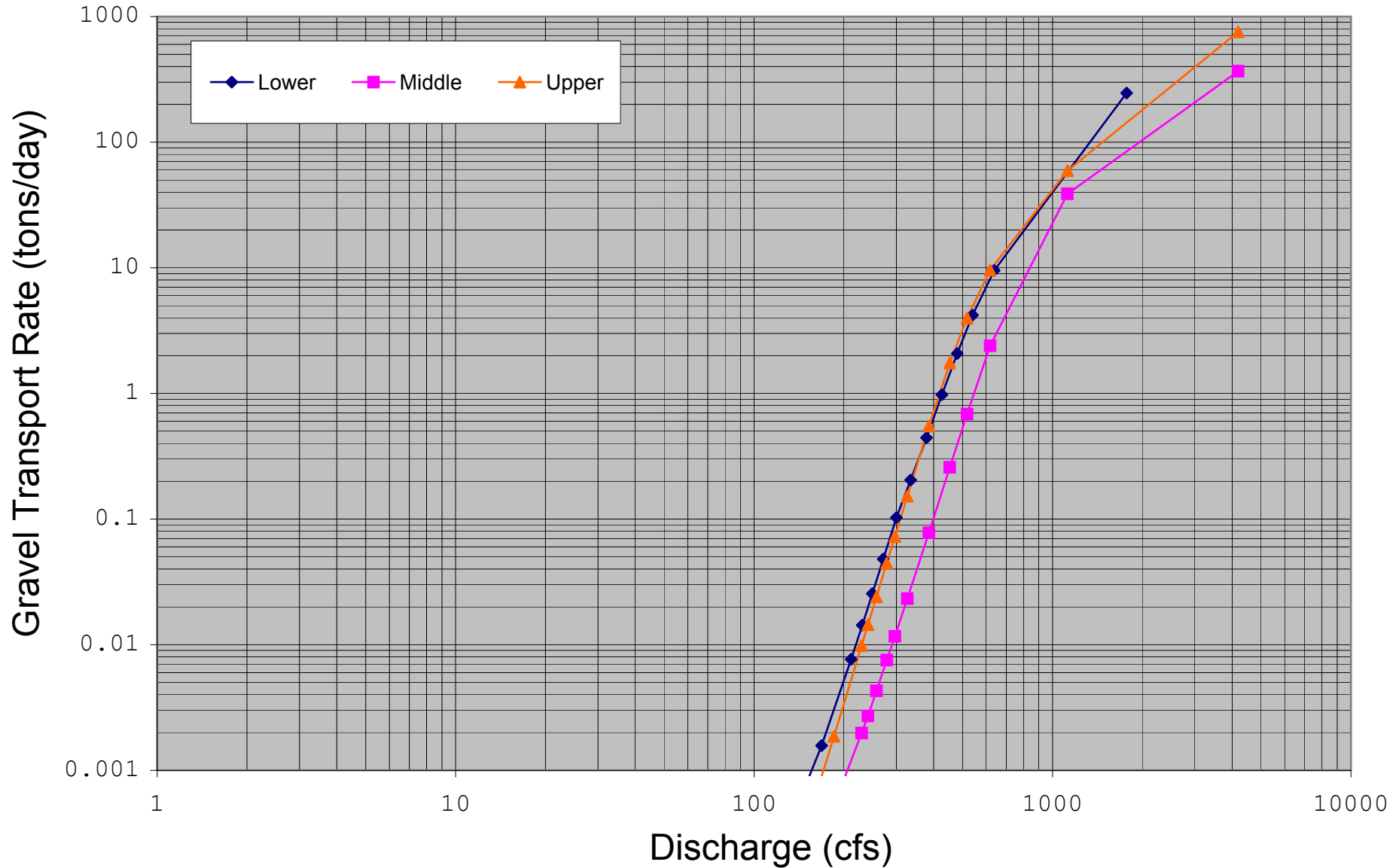
Figure N-11: Estimated bedload transport rating curve for the Ice House Dam Reach Lower Site.
