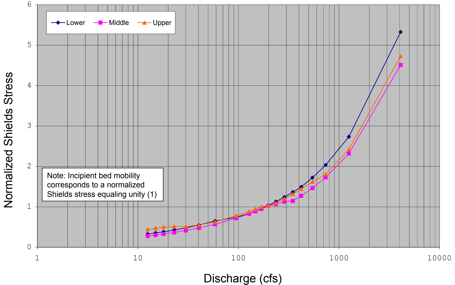
Figure N-2: Estimated Shields stress rating curve for the Rubicon Dam Reach Site.
