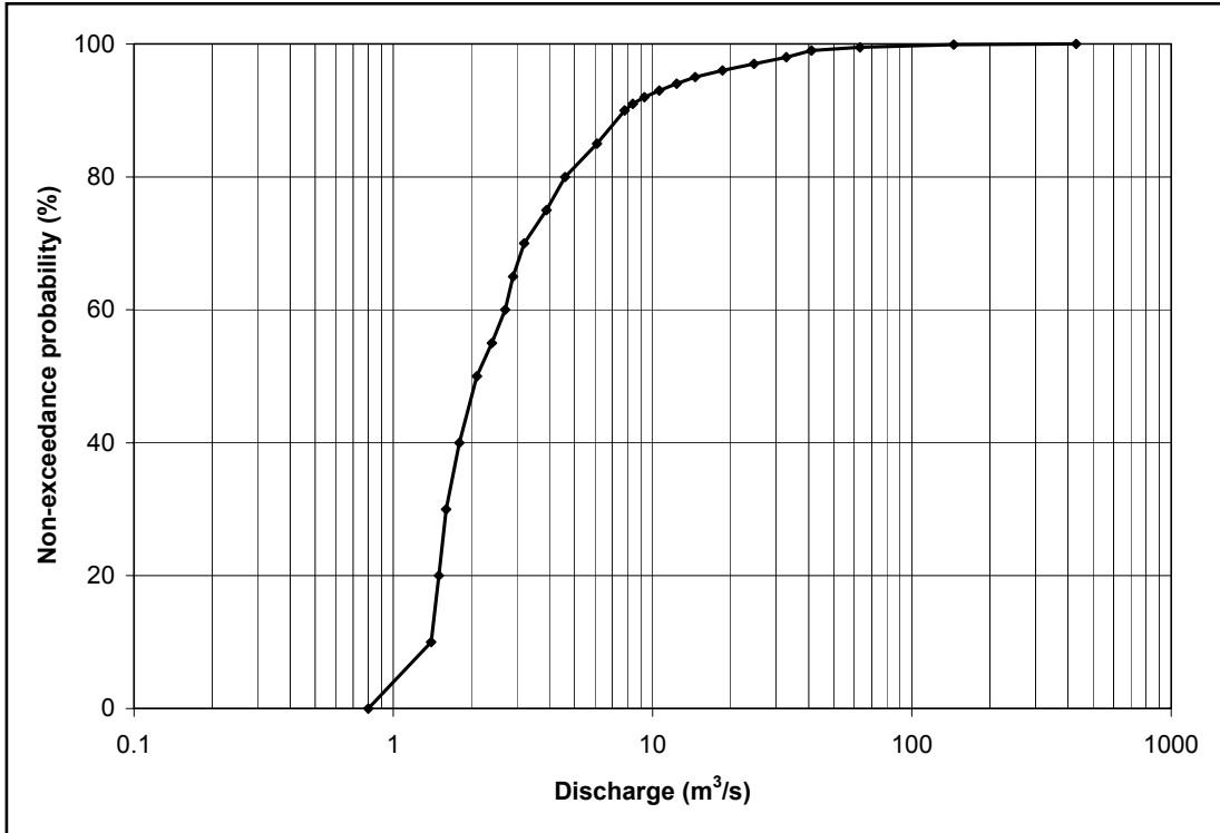
Figure M-4. Pre- and post-dam duration curves to be used in the example.
