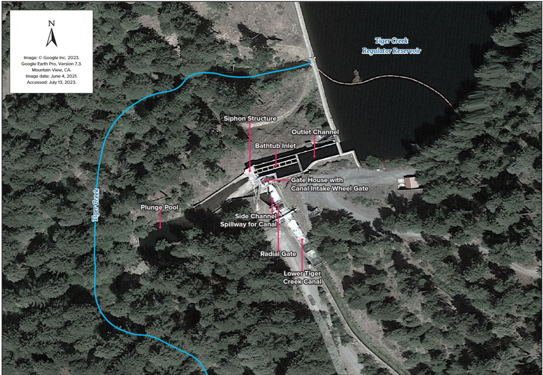
Figure 1-2 Existing Spillway Details
